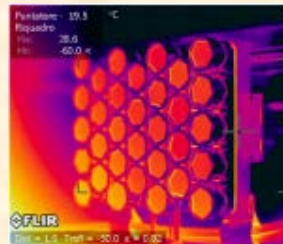
Third GPS flight array inside the SCF (left) and an IR thermogram taken during Solar Simulator illumination (right).
