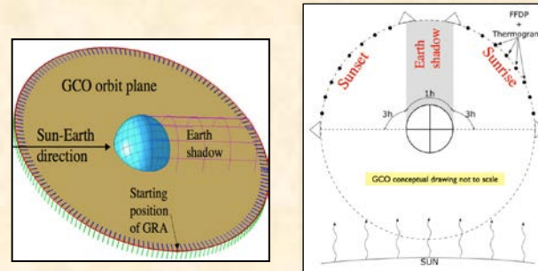
GNSS Critical Orbit (GCO) in space (left); GCO SCF-Test concept with measurement sequence & Solar Simulator illumination (right).
