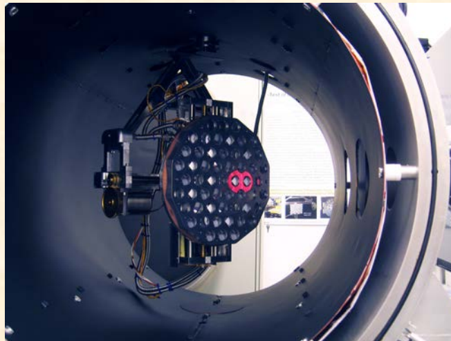
GRA (with the majority of its CCRs mounted) installed on the roto-translation positioning and thermal control system inside the SCF-G (top); GRA CCRs illuminated by external laser interrogation beam (bottom).
