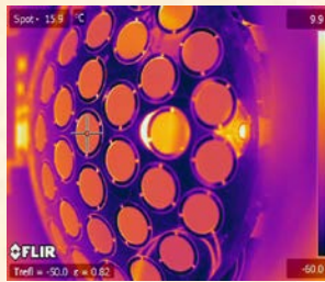
LAGEOS Sector: at GSFC (top left); in the SCF, temperature-controlled by an interface Cu plate, with laser illuminating one CCR (top right); IR thermogram (bottom left); CCR FFDP in velocity aberration plane in microrad units (bottom right).
