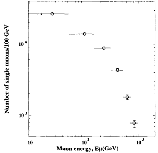
Fig. 5. Differential energy distribution of single muons with zenith angle \leq 45^\circ measured with the TRD. The spectrum was obtained by unfolding the hit distribution shown in Fig. 3.
