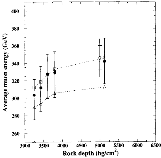
Fig. 9. Average single muon energy measured by the MACRO TRD (black circles) versus standard rock depth. The open symbols connected by dashed lines are the predictions of a HEMAS-based Monte Carlo for the “Light” (squares) and “Heavy” (triangles) composition models. The result reported by the NUSEX experiment is shown by the diamond (the extensions of the error bar represents the systematic uncertainty added in quadrature to the statistical error [4]).
