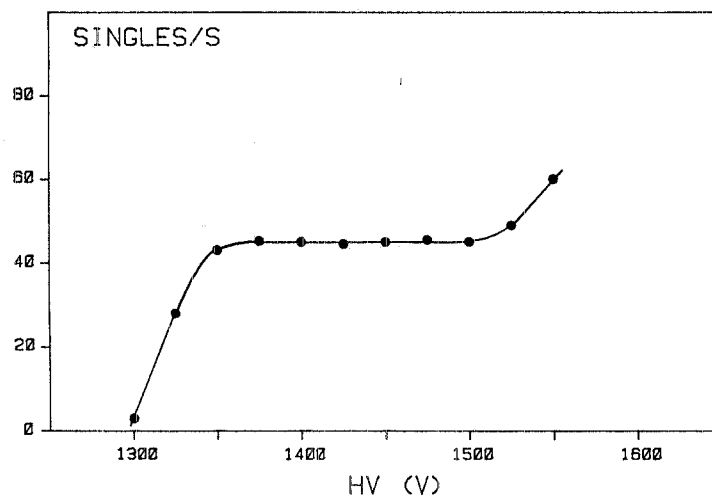
FIG. 2 - Singles rate vs. HV for a Geiger tube module with 100 \mu\text{m} wires; gas mixture: A + 2.6% Ethyl Bromide; the wires are connected to a CMOS GATE, with a 10 kOhm termination.
