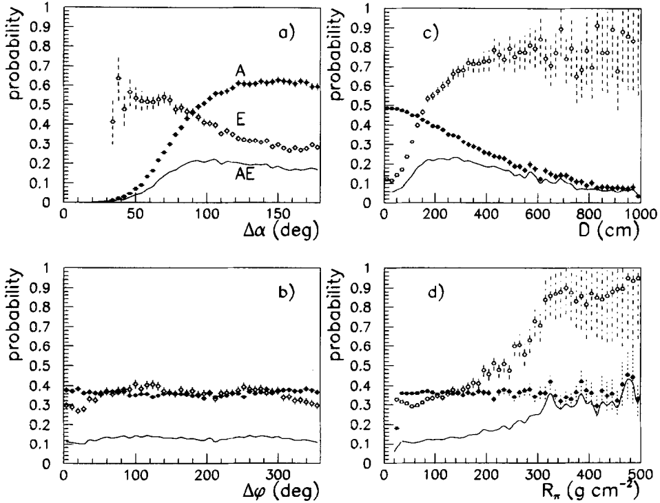
Fig. 6. Distribution of the probability A for events to be accepted, of the tracking efficiency E , and of the reconstruction efficiency AE versus (a) \Delta\alpha , (b) \Delta\phi , (c) D , and (d) R_\pi . Each quantity is averaged over the three remaining variables. Full points: A ; empty points: E ; solid curves: AE .
