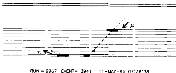
Fig. 1. On-line display of a typical muon interaction in the rock below the apparatus giving rise to an up-going charged particle. The rectangular boxes indicate scintillator counter hits and the points are streamer tube hits. The tracks are shown in the wire view of the streamer tubes. Only two supermodules are drawn.
