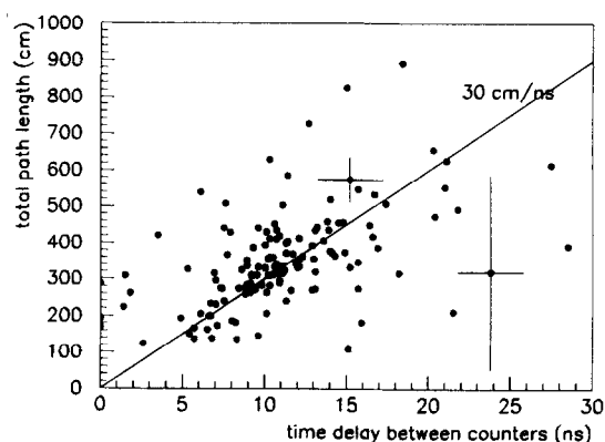
Fig. 3. Total path length (see text) versus time delay \Delta t = (T_3 - T_2) between scintillation counter hits in the bottom plane. Only the 168 events for which |z_v^w - z_v^s| < 50 cm are included. The large spread around the central line is due to the combined uncertainty in the total path length and timing reconstruction. As an example, error bars are drawn for two events. For three events, T_2 is missing and \Delta t = 0 .
