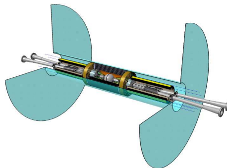
Figure 2: Design of the KLOE-2 interaction region, showing the new inner tracker and low-angle calorimeters.
