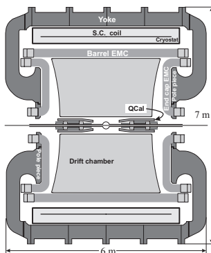
Figure 1: Cross section of the KLOE detector.
