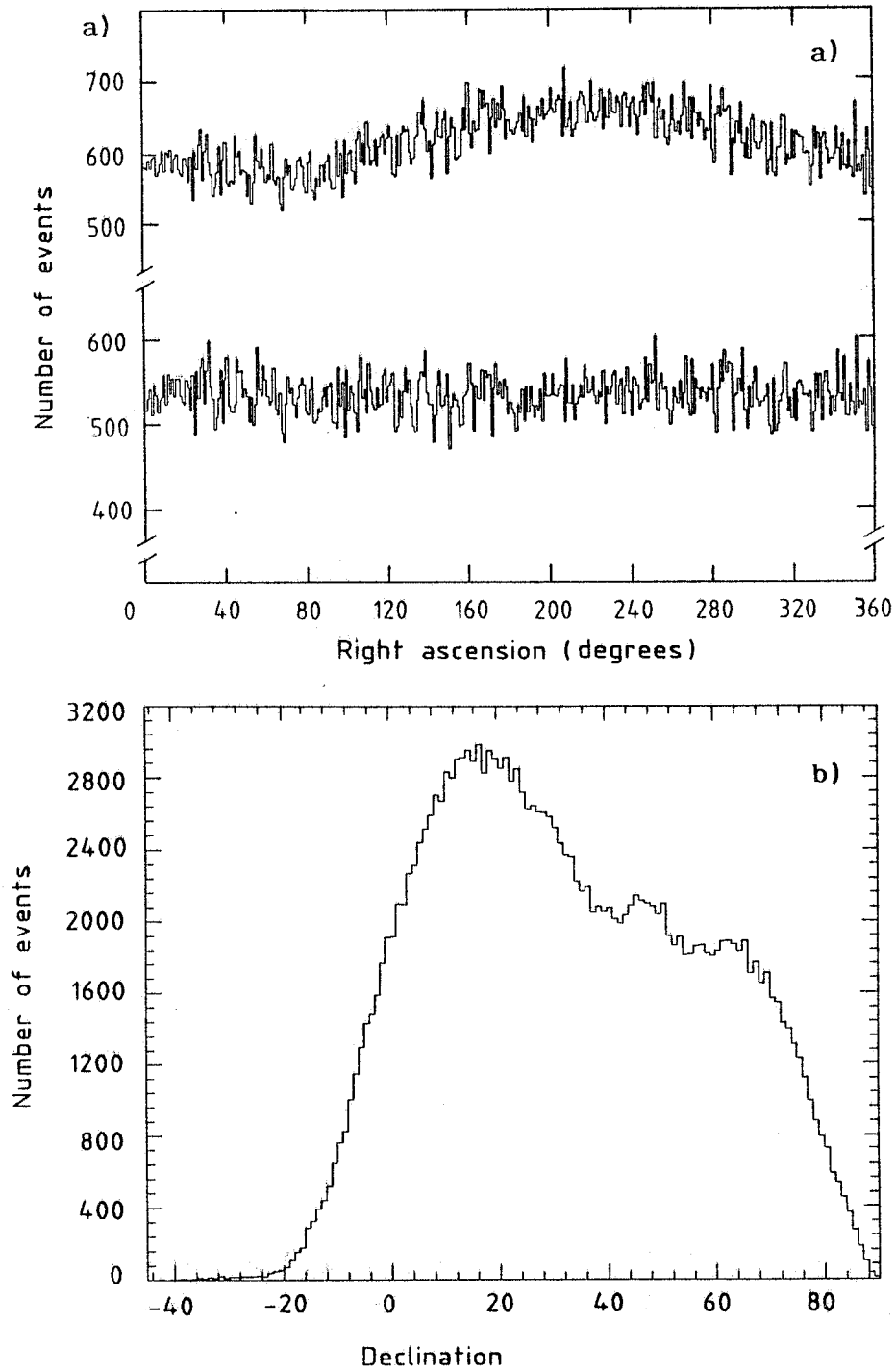
FIG. 4 - (a) Distributions in right ascension for single muons, before (top distribution) and after correction (bottom distribution) for the live-time of the apparatus. (b) Declination distribution for single muons after live-time correction.
