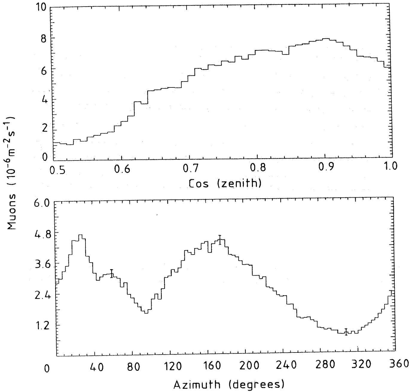
FIG. 2 - Measured zenith (a) and azimuth (b) distributions of muons crossing 10 horizontal planes of the MACRO detector corrected for detector acceptance ( \Delta\phi = 3.6^\circ , \Delta\cos\theta = 0.01 ). Some typical statistical errors are shown.
