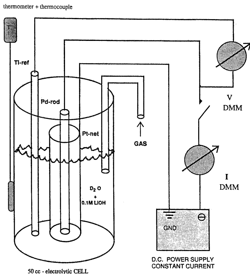
FIG. 2 - Experimental setup of electrolytic cell and power supply section (not to scale). All the connections between the electrolytic cell and the power supply or DMM are by coaxial cables to reduce the possibility of picking up external noise or radio-frequency emission from the electrolytic cell itself during the charging procedure. During the nuclear measurements, all Digital Multimeters and the thermometer were switched off to avoid spurious signals due to the sampling.
