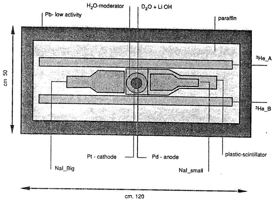
FIG. 1 - Electrolytic cell and detection apparatus setup (top view). The external shielding is made of 5-cm-thick low-activity lead bricks that completely surround the detectors. Paraffin bricks are enclosed between the neutron detectors and the external lead wall. The electrolytic cell, bunged with a rubber plug, is in a 4-cm-deep water bath.
