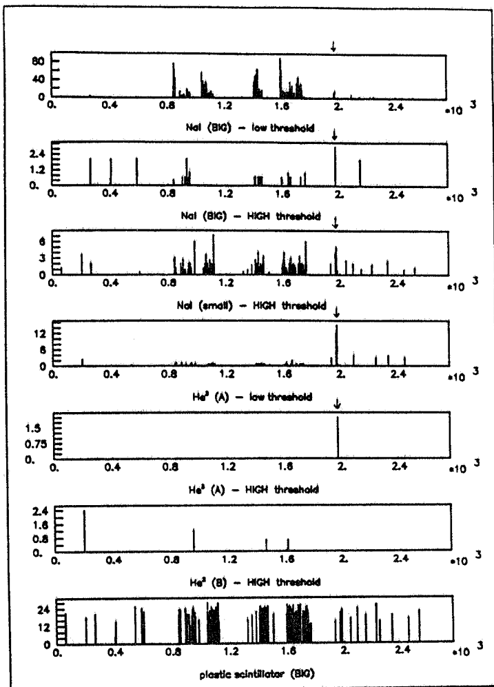
FIG. 3 - Palladium electrode life from May 2 to June 12, 1989. The effective total measurement time was > 20 days. Seven events were detected with a fusion rate > 3 \times 10^{-20} fusion/(deuteron pair-s). The arrow indicates when the new experimental setup was initiated.
