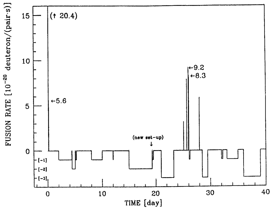
FIG. 3 - Palladium electrode life from May 2 to June 12, 1989. The effective total measurement time was > 20 days. Seven events were detected with a fusion rate > 3 \times 10^{-20} fusion/(deuteron pair-s). The arrow indicates when the new experimental setup was initiated.
