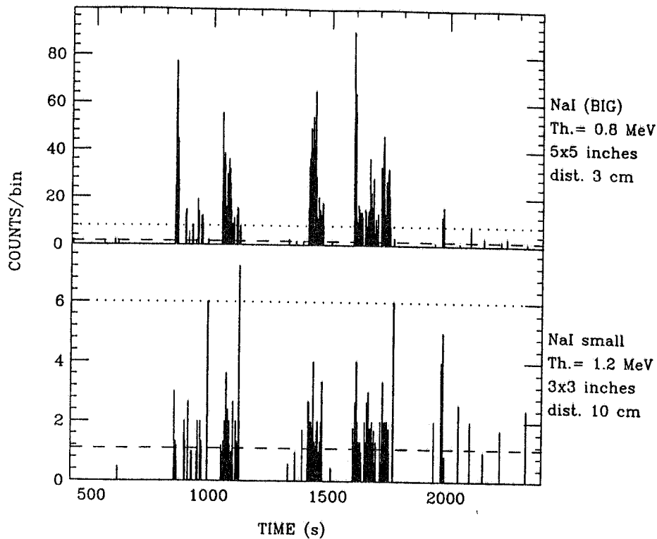
FIG. 5 - Details of event 4: counts from the two NaI(Tl) detectors. The dotted line indicates the software thresholds (8 and 6 count/bin for the large and small detectors, respectively) and the dashed line indicates the average background ( \sim 1.5 and 1.1 count/bin, respectively).
