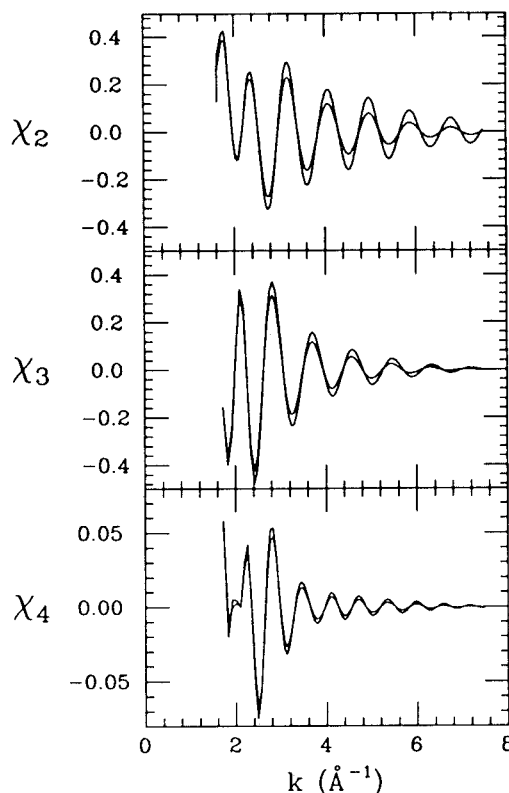
FIG. 3. Comparison between typical undamped multiple-scattering signals and their thermal averages at 500 K. From the top to the bottom the signals refer to the second-shell EXAFS or path 0-2-0 ( \chi_2 ), the double-scattering 0-1-2-0 ( \chi_3 ), and the triple-scattering 0-1-2-3-0 ( \chi_4 ), as shown in Fig. 1.
