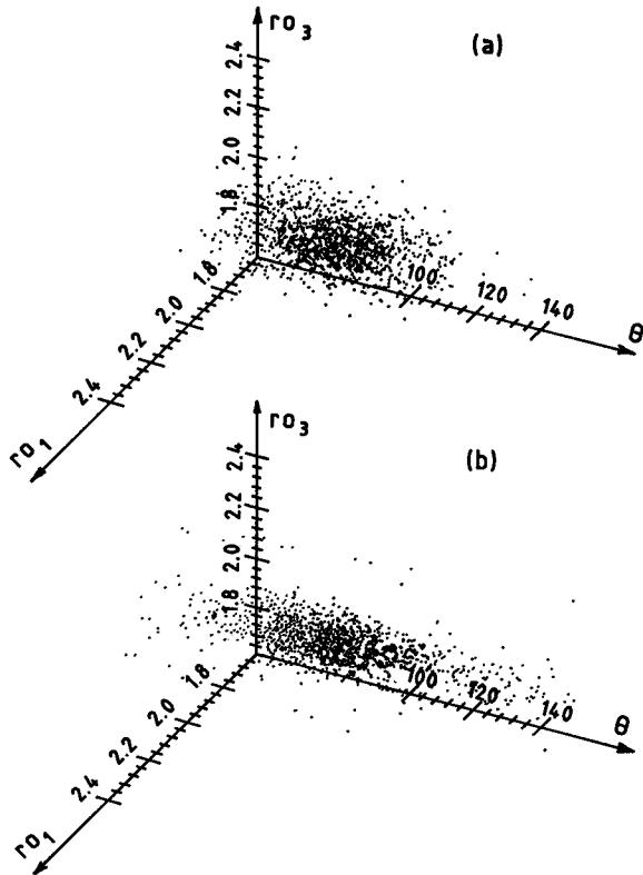
FIG. 2. Three-dimensional views of the fundamental peak of the three-body correlation function for the (a) Wooten-Winer-Weaire model and for the (b) Biswas-Soukoulis-Grest model. The peak refers to the basic triangle in the tetrahedron. The coordinates are, respectively, r_{01} , the first bond length; \theta , the angle between the two bonds 0-1 and 0-3; and r_{03} is, the second bond length (see Fig. 1). The peaks are evidently Gaussians and are centered around the c -Si values of 2.352 Å for the distances and 109.47° for the angle. The difference between the two models is evident.
