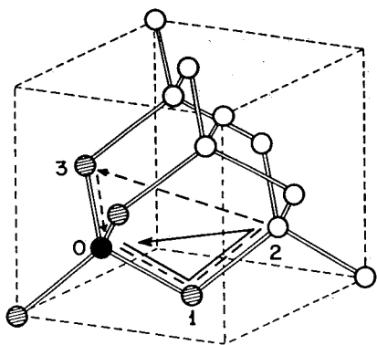
FIG. 1. Local order of the c -Si structure. The \chi_3 path 0-1-2-0 and the \chi_4 path 0-1-2-3-0 are shown by the arrows.
