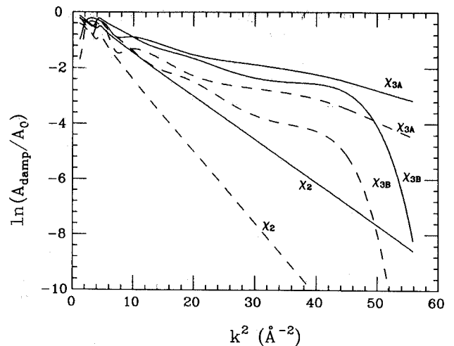
FIG. 5. Effective dampings for the three relevant multiple-scattering paths in the a -Si structure besides the trivial first-shell EXAFS. They are the second-shell \chi_2 signal and the \chi_{3A} and \chi_{3B} double-scattering signals as described in the text. On the y axis we report the logarithm of the ratio between damped and undamped amplitudes and on the x axis the square of the photoelectron momentum. The solid lines refer to the Wooten-Winer-Weaire model, while the dashed lines refer to the Biswas-Soukoulis-Grest model. The difference between the corresponding signals is evident.
