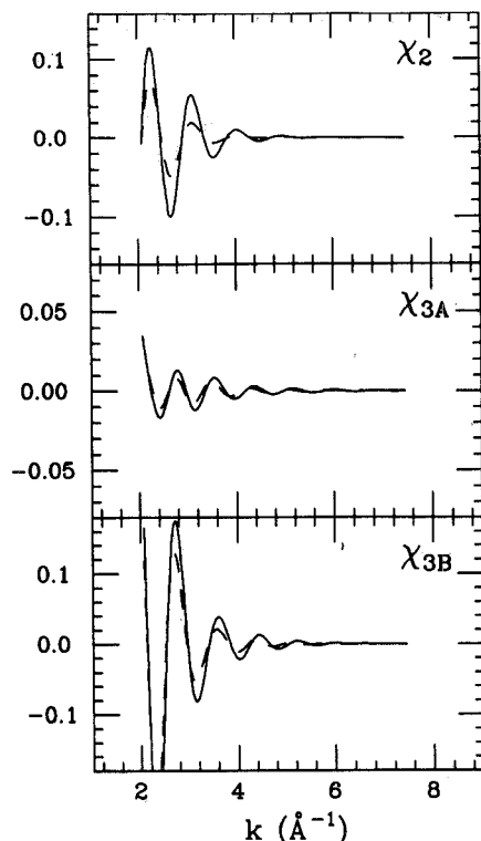
FIG. 6. Comparison of the signals \chi_2 , \chi_{3A} , and \chi_{3B} between the WWW and BGS models for \alpha -Si. The differences in amplitude and in phase are evident. The dashed line refers to the BGS model.
