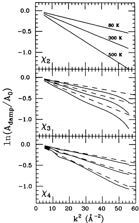
FIG. 4. Effective dampings for the three prototypical multiple-scattering, \chi_2 , \chi_3 , and \chi_4 , paths described in the text. On the y axis we report the logarithm of the ratio between damped and undamped amplitudes and on the x axis the square of the photoelectron momentum. In each plot three curves are reported which refer to the temperatures of 80, 300, and 500 K, as indicated in the plot for \chi_2 . The dashed lines refer to the pure geometrical damping, while the solid lines refer to the total effective damping which also takes into account the phase term.
