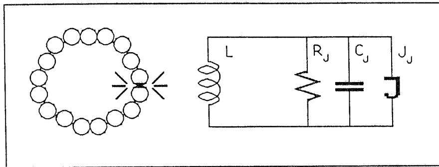
Fig. 1. Superconducting granular loop, and its equivalent circuit; L is the inductance of the loop, R_J and C_J are the resistance and the capacitance of the weakest Josephson junction between grains.
