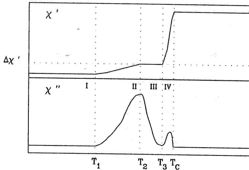
Fig. 3. Qualitative temperature dependence of \chi' and \chi'' ; four ranges are identified: I) \bar{H}_A < H_{C1}^G , II) H_{C1}^G < \bar{H}_A < H_{C2}^G , III) H_{C2}^G < \bar{H}_A < H_{C1} , IV) H_{C1} < \bar{H}_A < H_{C2} .
