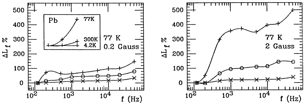
Fig. 5. Frequency dependence of \Delta L_f\% as function of the frequency for two different fields. (+ Oxygen made pellet, x Ozone made pellet, o Ozone powder).
