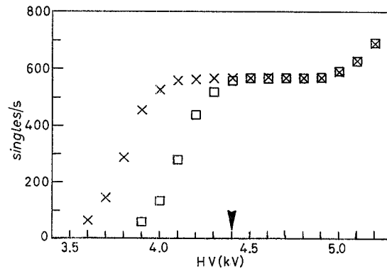
Fig. 3. - Singles counting rate for the streamer tubes for isotropic electrons ( ^{90}\text{Sr} ) and single photoelectrons. Starting from \sim 4.4 kV, single electrons are detected with practically full efficiency and without spurious pulse detection. (3 \times 3) cm ^2 , 60 \mu\text{m} , He+n-pentane, 3:1. x \beta , \square single electron.
