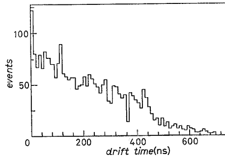
Fig. 5. — Drift time distribution for the streamer tubes as measured with cosmic rays. The distribution is that expected given the geometry of the cell. The resulting time accuracy is \sim 150 ns. (3 \times 3) cm 2 , 60 \mu\text{m} ; He+n-pentane, 3:1, HV = 4.4 kV.
