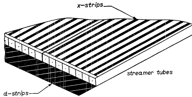
Fig. 1. - Schematic sketch for a plastic streamer tube layer for large-area detectors. Many 8-tube units can be combined together. Two-dimensional localization is performed by two sets of pick-up strips. They can be placed at any angle according to the experimental requirements.
