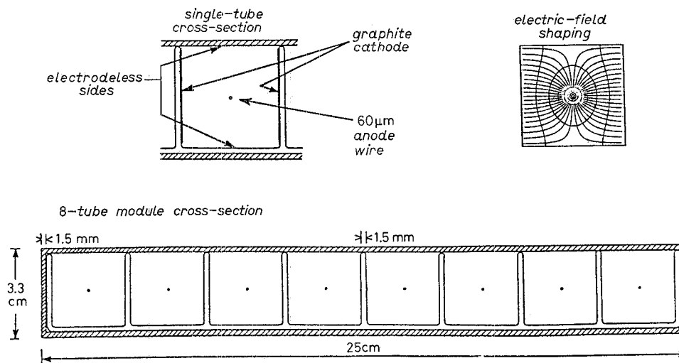
Fig. 2. - Cross-section of an 8-tube unit. The electric field shaping is given by the wire, the graphite cathode and the positive ion charge deposited in the electrodeless faces by stationary streamer operation.
