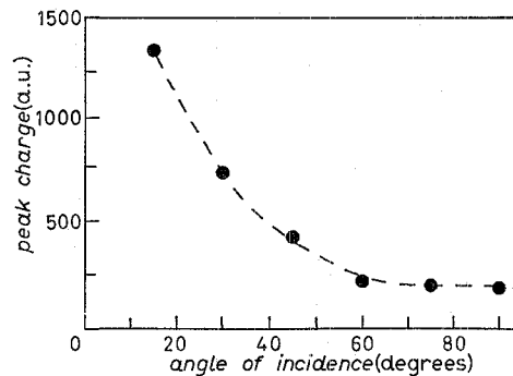
Fig. 6. — Streamer pulse height vs. the angle of the track with respect to the wire, as measured with cosmic rays. For a given streamer dead region length (fixed by the gas mixture) the pulse height is a measure of the track projection along the wire. (3 \times 3) cm 2 , 60 \mu\text{m} , \mu , He+n-pentane, 3:1, 4.4 kV.
