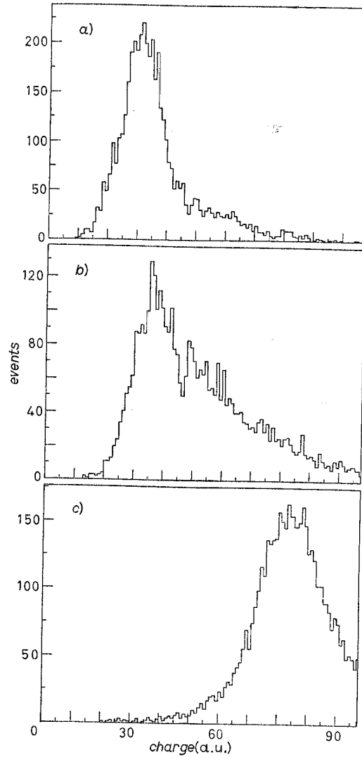
Fig. 7. - Streamer pulse height distribution with our tube module and gas mixture for a) single electrons, b) isotropic minimum-ionizing particles and c) isotropic heavily ionizing \alpha -particles. This preliminary result shows the capability of streamer tubes to detect large ionization losses with respect to the minimum.
