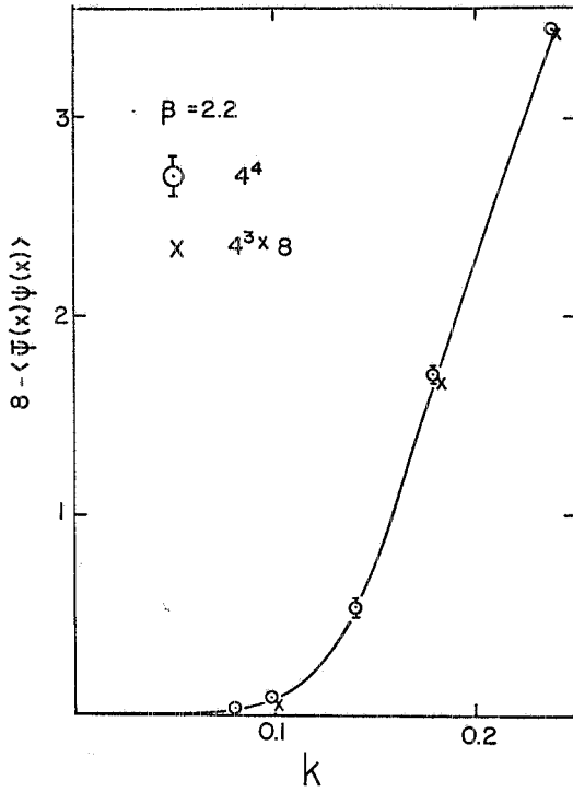
FIG. 7 - Expectation value per flavour of 8 - \bar{\psi}(x)\psi(x) as a function of the hopping parameter k . The solid line is a spline interpolation for the data on a 4^4 lattice. The crosses are the corresponding expectation values in a 4^3 \times 8 lattice.
