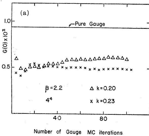
FIG. 6 - (a) Time slice plaquette-plaquette correlation function G(\tau) at \tau=0 against the number of MC gauge sweeps. The solid line stands for the pure gauge case. The triangles correspond to k=0.20 and have been obtained with a thermalization of 40 gauge MC iterations. The crosses correspond to k=0.23 and the thermalization is 68 sweeps. (b) Time slice plaquette-plaquette correlation function G(\tau) at \tau=1 against the number of MC gauge sweeps. The hatched region stands for the corresponding value in the pure gauge case. The crosses correspond to k=0.23 and the thermalization for gauge fields is 68 sweeps.
