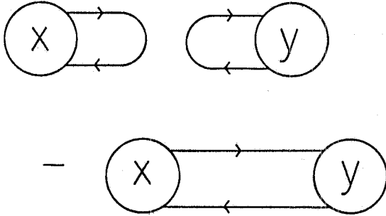
FIG. 1 - Diagrammatic representation of the fermion contribution to the meson propagator (equation (10)). The first graph represents the quark loops contribution to meson propagator, which is different from zero only for flavour-singlet mesons.
