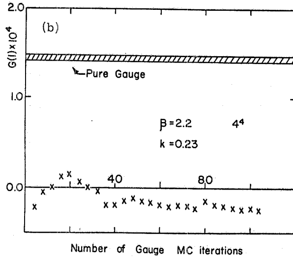
FIG. 6 - (a) Time slice plaquette-plaquette correlation function G(\tau) at \tau=0 against the number of MC gauge sweeps. The solid line stands for the pure gauge case. The triangles correspond to k=0.20 and have been obtained with a thermalization of 40 gauge MC iterations. The crosses correspond to k=0.23 and the thermalization is 68 sweeps. (b) Time slice plaquette-plaquette correlation function G(\tau) at \tau=1 against the number of MC gauge sweeps. The hatched region stands for the corresponding value in the pure gauge case. The crosses correspond to k=0.23 and the thermalization for gauge fields is 68 sweeps.
