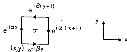
Fig. 1. The flux of the magnetic field H through an elementary plaquette \sigma in the x, y plane.
