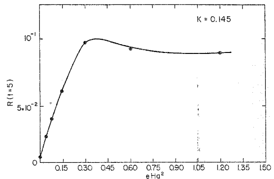
Fig. 2. R(t=5) defined in eq. (10) as a function of H . Notice that its behaviour for large H is expected to go (approximately) as the difference of two hyperbolic tangents.
