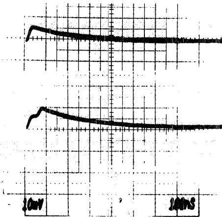
FIG. 7 - Signals on a pad due to single and double streamers (50 Ω load).
