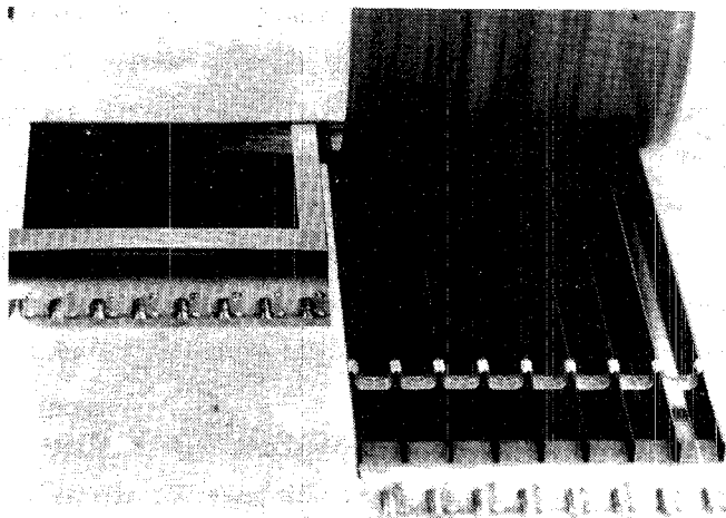
FIG. 1 - Plastic Streamer Tube module.
