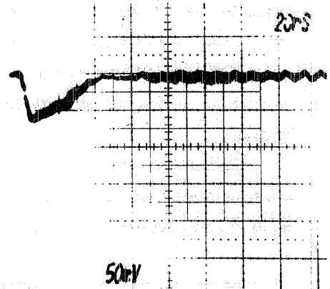
FIG. 6 - A typical single streamer pulse as detected on the wire (50 Ω load).
