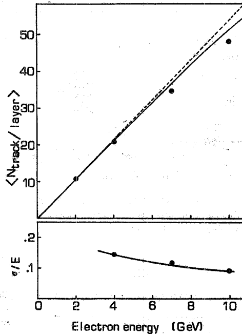
FIG. 10 - Signal and energy resolution as a function of electron energy. The signal is in units of orthogonal track signal (non interacting pions). The solid line comes from the experimental points corrected for shower losses on the back. The non linearity at 10 GeV is 6%.
