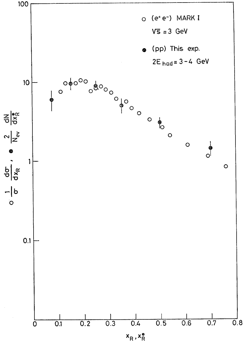
Fig. 1. -- The inclusive fractional-momentum distribution (2/N_{ev})(dN/dx_R^*) ( x_R^* = |\mathbf{p}|/E_{had} ) for (pp) data at 2E_{had} = (3 \div 4) GeV, compared with the distribution (1/\sigma)(d\sigma/dx_R) , ( x_R = 2|\mathbf{p}|/\sqrt{s} ) in (e + e - ), at (\sqrt{s})_{e^+e^-} = 3 GeV (Mark I).
