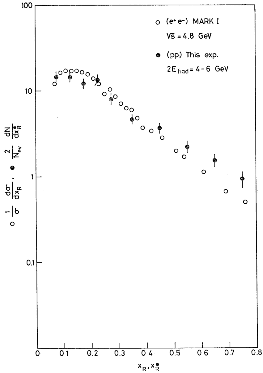
Fig. 2. - The same distributions as in fig. 1, at 2E_{\text{had}} = (4 \div 6) GeV for (pp) data, and (\sqrt{s})_{e^+e^-} = 4.8 GeV for (e^+e^-) data.
