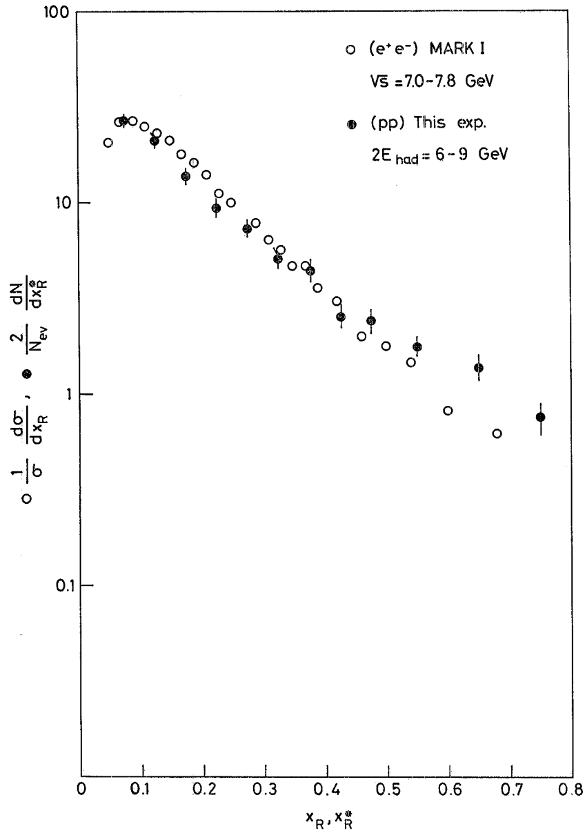
Fig. 3. - The same distributions as in fig. 1, at 2E_{had} = (6 \div 9) GeV for (pp) data, and (\sqrt{s})_{e^+e^-} = (7.0 \div 7.8) GeV for (e + e - ) data,
