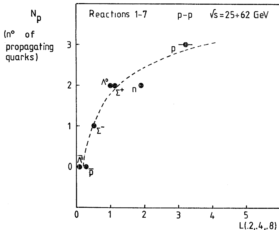
Fig. 13. - The leading quantity L(0.2, 0.4, 0.8) for various final-state hadrons in pp collisions at ISR energies ( 25 \div 62 GeV) is plotted vs. the number of propagating quarks from the incoming into the final-state hadrons. The dashed line is obtained by using a parametrization of the single-particle inclusive cross-section, as described in the text.
