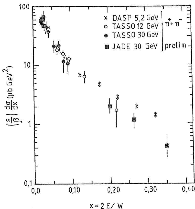
Fig. 1. - Inclusive production of hadrons in (e^+e^-) annihilation. e) The scaled cross-section (s/\beta) d\sigma/dx for charged pions (ref. (17,18)).
