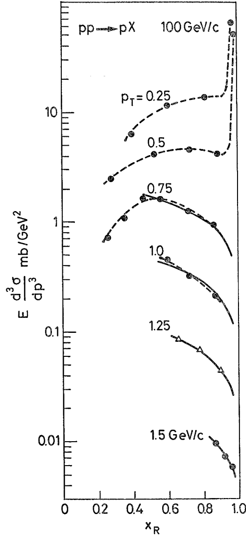
Fig. 4. — Inclusive production of hadrons in (pp) interactions. The invariant cross-section E(d^3\sigma/dp^3) at 100 GeV/c as a function of x_R at various p_T from 0.25 to 1.5 GeV/c for protons (ref. (26)). Open triangles at p_T = 1.25 GeV/c are data at 400 GeV/c. The dashed lines on the figure are hand-drawn to guide the eye through the data points; the full line is the shape of the (1-x)^{0.5} functional behaviour.
