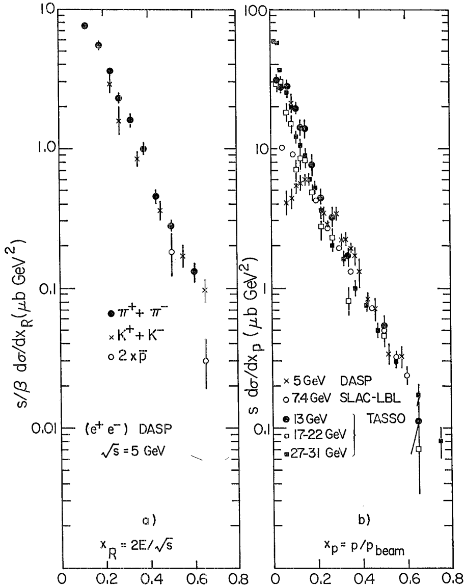
Fig. 1. - Inclusive production of hadrons in (e^+e^-) annihilation. a) The cross-section (s/\beta)(d\sigma/dx_R) vs. x_R for (\pi^+ + \pi^-) , (K^+ + K^-) and twice the \bar{p} yield for \sqrt{s} = 5 GeV (ref. (15) ). b) The cross-section s(d\sigma/dx_p) for inclusive charged-particle production measured at energies of 5 to 30 GeV (ref. (16) ).
