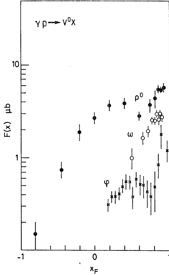
Fig. 10. - Inclusive x_F distribution of vector mesons in (\gamma p) interactions: \rho meson (ref. (33) ) and \omega meson (ref. (34) ) at \gamma energy of 9.2 GeV. The \phi -meson distribution (plotted with arbitrary normalization from ref. (35) ) is for a \gamma energy of 25.70 GeV.
