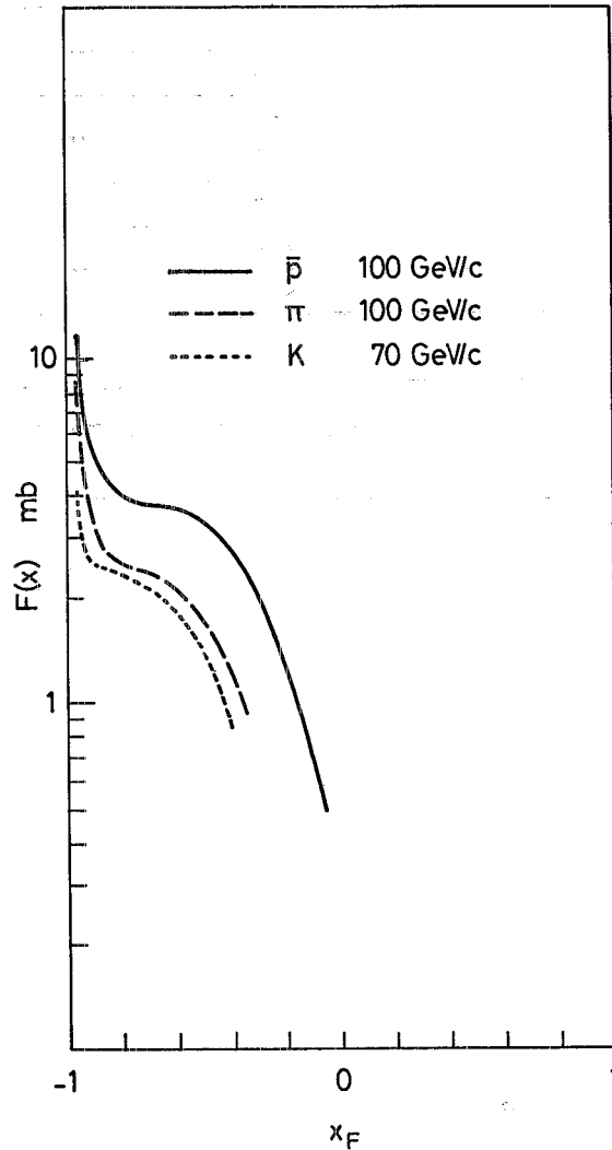
Fig. 12. - b ) x_F distribution for the target proton in the reactions (\pi p) , (Kp) , (\bar{p}p) .
