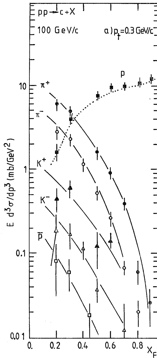
Fig. 2. - Inclusive production of hadrons in (pp) interactions. The invariant cross-section E(d^3\sigma/dp^3) at 100 GeV/c as a function of x_F at fixed p_T = 0.3 \text{ GeV/c} , for p , \pi^\pm , K^\pm and \bar{p} (ref. (25) ).
