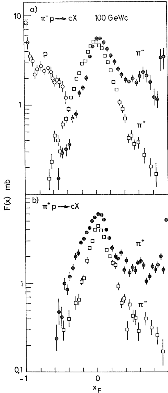
Fig. 7. - Inclusive production of hadrons in (\pi p) and (Kp) interactions. a ) Invariant cross-section integrated over p_T as a function of x_F for \pi^+ , \pi^- and p as measured in 100 GeV/c (\pi^- p) interactions in a hydrogen bubble chamber. (Data from ref. (28,29) .) b ) The same as for (a) using 100 GeV/c (\pi^+ p) interactions. (Data from ref. (28) .)
