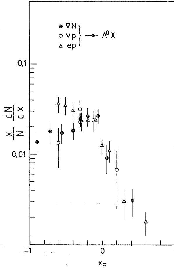
Fig. 16. — Inclusive production of the \Lambda^0 baryon in ( \bar{\nu}N ), ( \nu p ) and ( ep ) interactions. Data from ref. (41) are normalized to the same cross-section.
