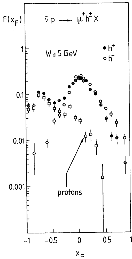
Fig. 15. - Inclusive production of hadrons in (\bar{\nu}p) charged-current interactions. The centre-of-mass x_F distributions for positive-charge particles ( h^+ ), for negative-charge particles ( h^- ), and for identified protons (ref. (40) ).
