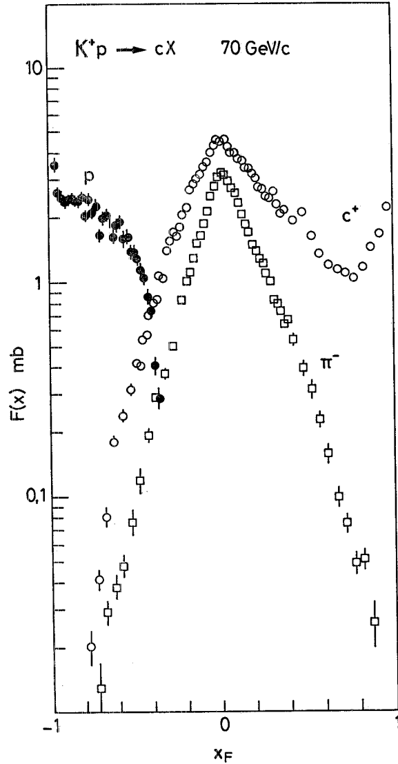
Fig. 7. - Inclusive production of hadrons in (\pi p) and (Kp) interactions. c) Invariant cross-section at fixed p_T = 0.3 GeV/c as a function of x_F for inclusive production in (K^+p) interactions at 70 GeV/c in BEBC. (Data from ref. ( 30,31 )). Shown is the x_F distribution of positively charged mesons c^+ (slow protons subtracted) of \pi^- and of the target protons.
