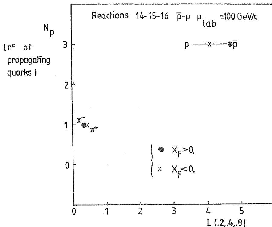
Fig. 6. - L(0.2, 0.4, 0.8) for final-state hadrons produced in \bar{p} -p collisions at P_{\text{lab}} = 100 \text{ GeV/c} .
