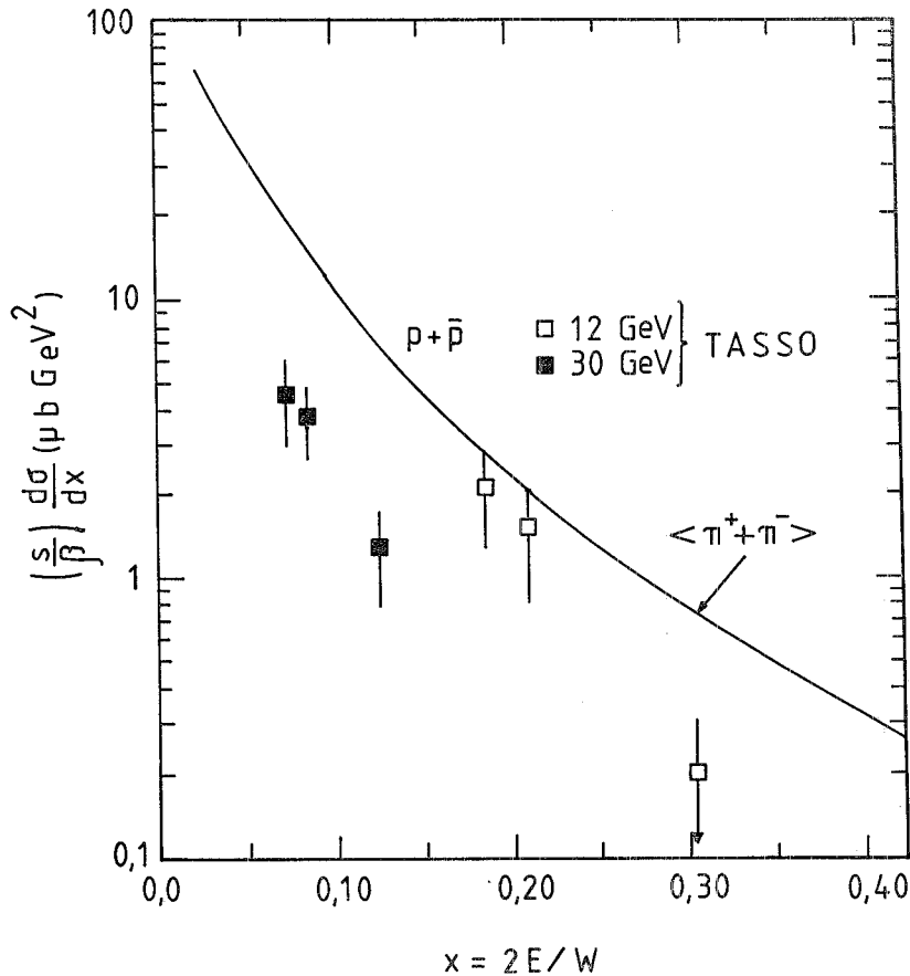
Fig. 1. - Inclusive production of hadrons in ( e^+e^- ) annihilation. e) The scaled cross-section (s/\beta) d\sigma/dx for protons and antiprotons (ref. ( 18,20 )). The average charged-pion cross-section is shown as the solid curve.
