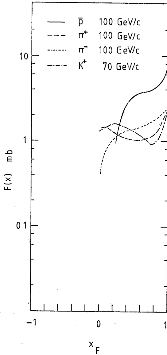
Fig. 12. - a ) x_F distribution in the beam x_F -region ( x_F > 0 ) for \pi^\pm , K^+ and \bar{p} incident particles on the target protons.
