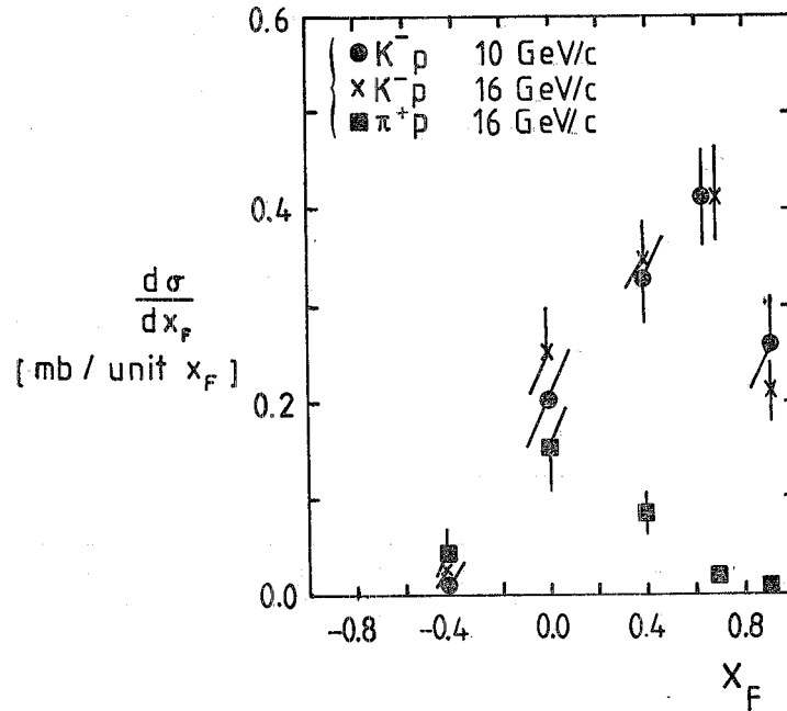
Fig. 14. - Centre-of-mass x_F distribution for inclusive production of \varphi -mesons in K^-p and \pi^+p interactions (ref. (32) ).
