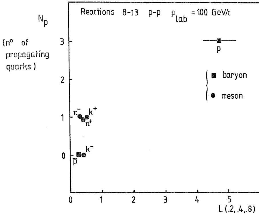
Fig. 3. - L(0.2, 0.4, 0.8) for various final-state hadrons produced in pp collisions at P_{\text{lab}} = 100 GeV/c.
