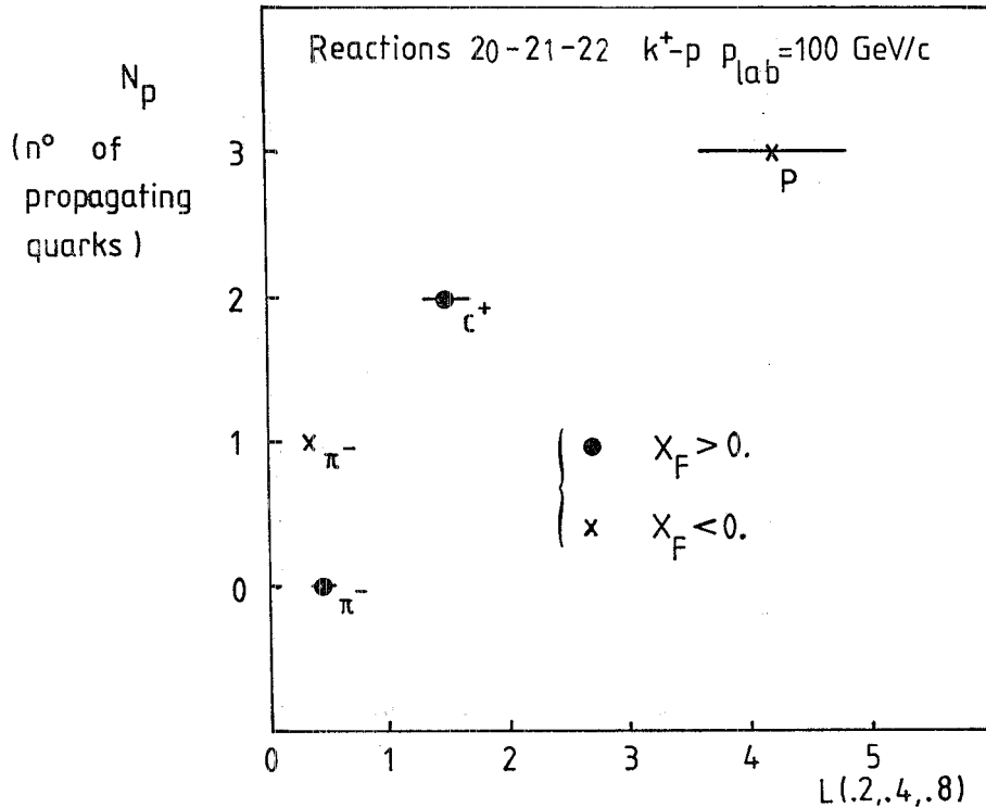
Fig. 9. — L(0.2, 0.4, 0.8) for final-state hadrons produced in K^+p at P_{lab} = 100 GeV/c.
