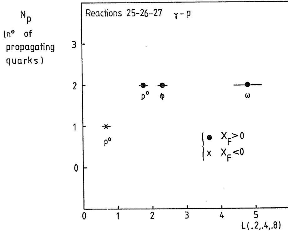
Fig. 11. - L(0.2, 0.4, 0.8) for final-state vector mesons produced in \gamma p .
