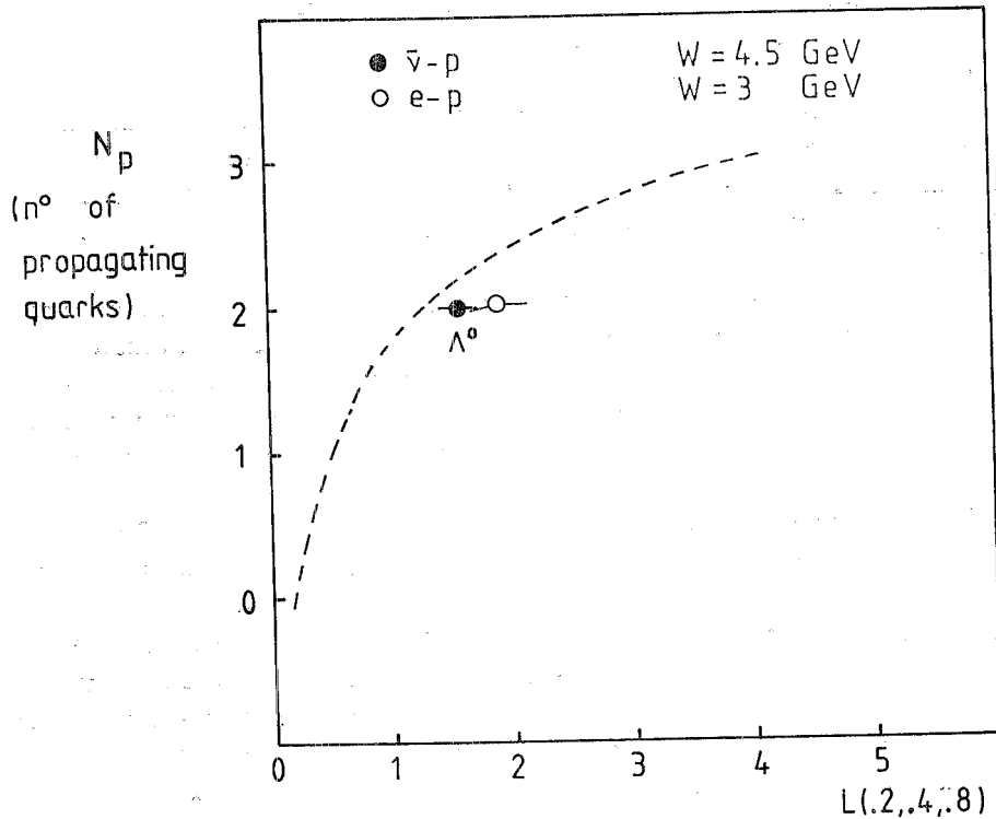
Fig. 17. - L(0.2, 0.4, 0.8) for \Lambda^0 productions in (\bar{\nu}p) and (ep) reactions. The dashed line is the same as that described for fig. 13.
