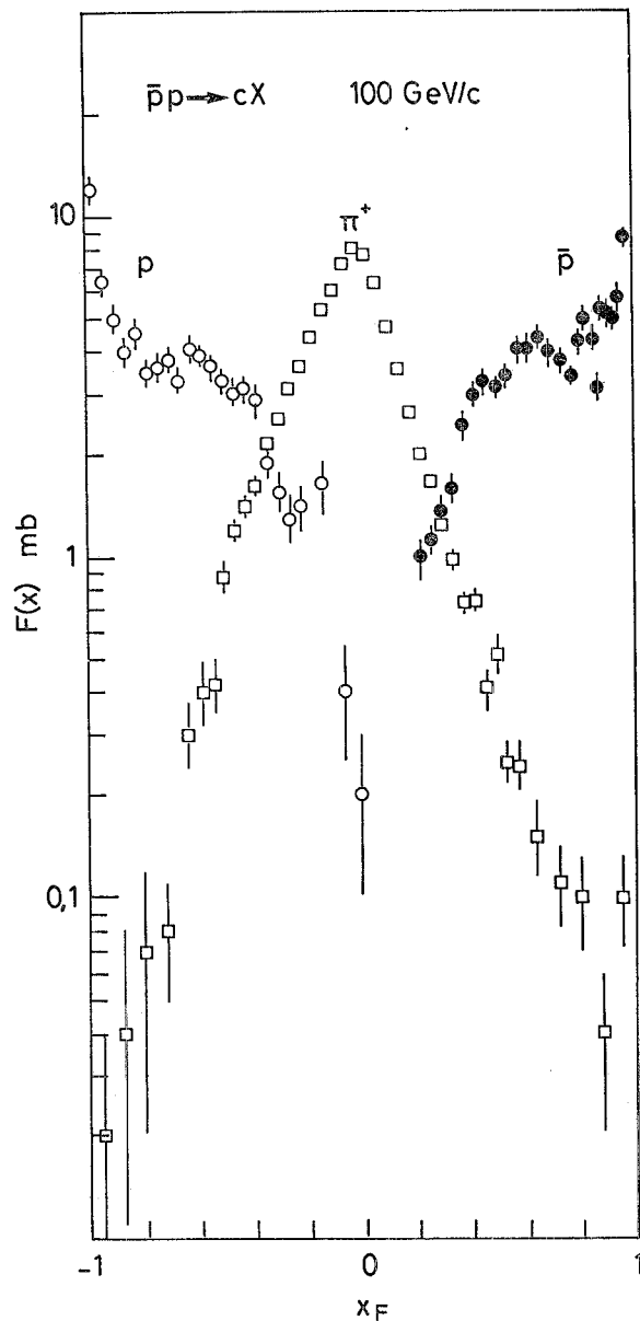
Fig. 5. — Inclusive production of hadrons in ( p\bar{p} ) interactions. Invariant cross-section integrated over p_T as a function of x_F for \pi^+ , p and \bar{p} as measured in 100 GeV/c \bar{p} interactions in a hydrogen bubble chamber. (Data from ref. ( 27 .)
