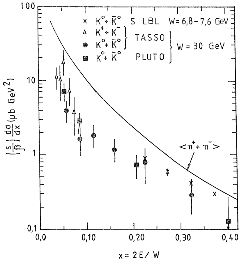
Fig. 1. — Inclusive production of hadrons in (e^+e^-) annihilation. d) The scaled cross-section (s/\beta)d\sigma/dx for neutral and charged kaons (ref. (17-19) ). The average pion cross-section is shown as the solid curve.
