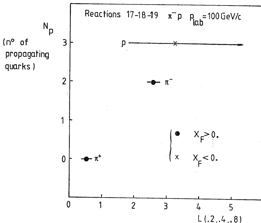
Fig. 8. - L(0.2, 0.4, 0.8) for final-state hadrons produced in \pi^-p at P_{\text{lab}} = 100 \text{ GeV}/c .
