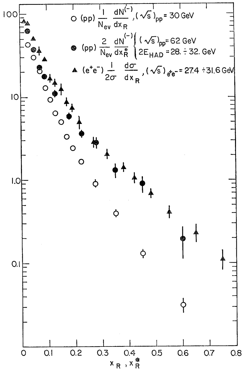
Fig. 1. - The inclusive fractional-momentum distributions of negative particles, for pp interactions by using the standard analysis at (\sqrt{s})_{pp} = 30 GeV ( \circ ), by using the method of removing the leading protons at (\sqrt{s})_{pp} = 62 GeV and 2E_{had} = (28 \div 32) GeV ( \bullet ); the e^+e^- data at (\sqrt{s})_{e^+e^-} = (27.4 \div 31.6) GeV ( \blacktriangle ).
