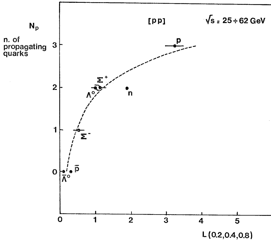
Fig. 1. - The «leading» quantity L(0.2, 0.4, 0.8) derived for different types of baryons produced in (pp) collisions at the CERN ISR. The centre-of-mass energy ranges from 25 to 62 GeV. The hadrons are ordered according to the number of propagating quarks. The dashed curve superimposed is obtained by using a parametrization of the single-particle inclusive cross-section, F(x) = (1-x)^\alpha , as described in sect. 3.
