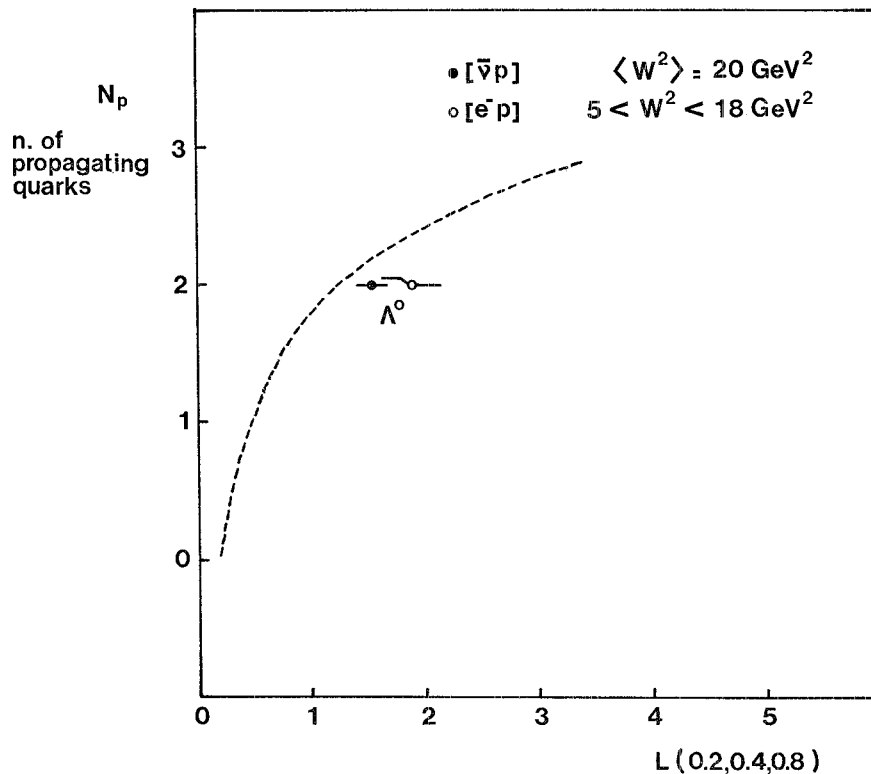
Fig. 2. - The « leading » quantity L(0.2, 0.4, 0.8) of the \Lambda^0 produced in (\bar{\nu}p) interactions at \langle W^2 \rangle = 20 (\text{GeV})^2 and in (e^-p) interactions with 5 < W^2 < 18 (\text{GeV})^2 . In this case the number of propagating quarks is two. The dashed curve of fig. 1 is also shown to guide the eye.
