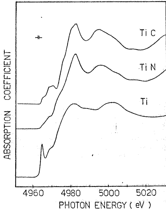
FIG. 2 - X-ray absorption near-edge structure (XANES) of Ti in metallic titanium and stoichiometric TiC and TiN. The onset of K absorption in Ti metal occurs at 4964.0 \pm 0.5 eV. In TiC and TiN a chemical shift of \sim 1 eV with respect to pure Ti is observed. The estimated experimental resolution around 5 keV is better than 0.5 eV.
