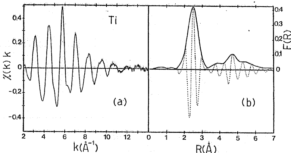
FIG. 15 - a) k \cdot \chi(k) for metallic titanium film. b) Magnitude F(R) and imaginary part \text{Im } F(R) of the Fourier transform of k \cdot \chi(k) vs. R . The integration range is k_{\text{min}} = 2.3 \text{ \AA}^{-1} and k_{\text{max}} = 14.5 \text{ \AA}^{-1} . A Gaussian window W(k) is used.
