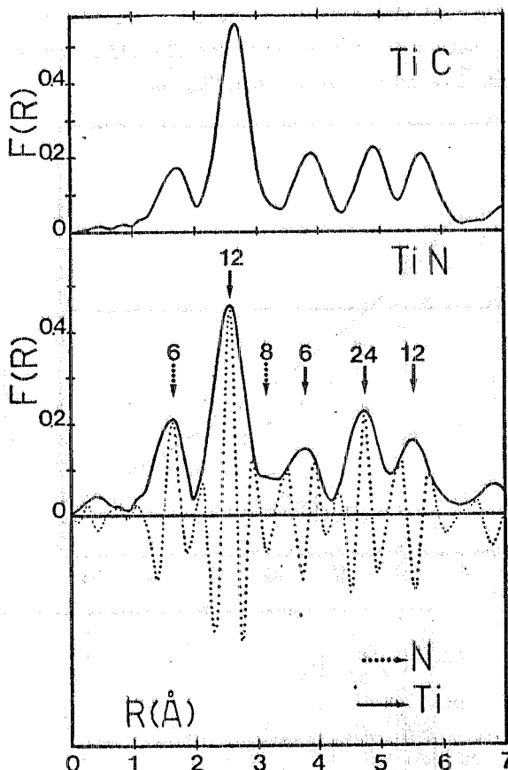
FIG. 20 - F(R) derived from k \cdot \chi(k) of Fig. 19. For TiN the \text{Im } F(R) function is also shown. The labeled arrows mark the position and the coordination number of the N and Ti atoms in the lattice.
