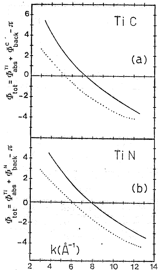
FIG. 21 - Experimental phases a) \Phi_{Ti-C}(k) and b) \Phi_{Ti-N}(k) . The solid lines are the theoretical phases of Teo and Lee.
