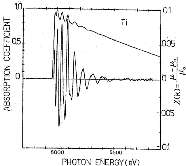
FIG. 14 - Experimental Ti K absorption spectrum after preedge subtraction and extracted EXAFS modulation k\chi(k) .
