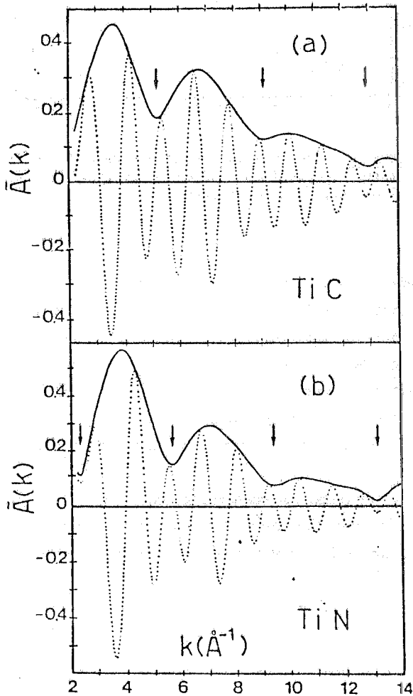
FIG. 24 - k\chi(k) and \tilde{A}(k) for (a) TiC and (b) TiN obtained by backfourier transforming the C and Ti peaks of F(R) in Fig. 20 between 1 and 3 Å. The beating minima are marked by arrows.
