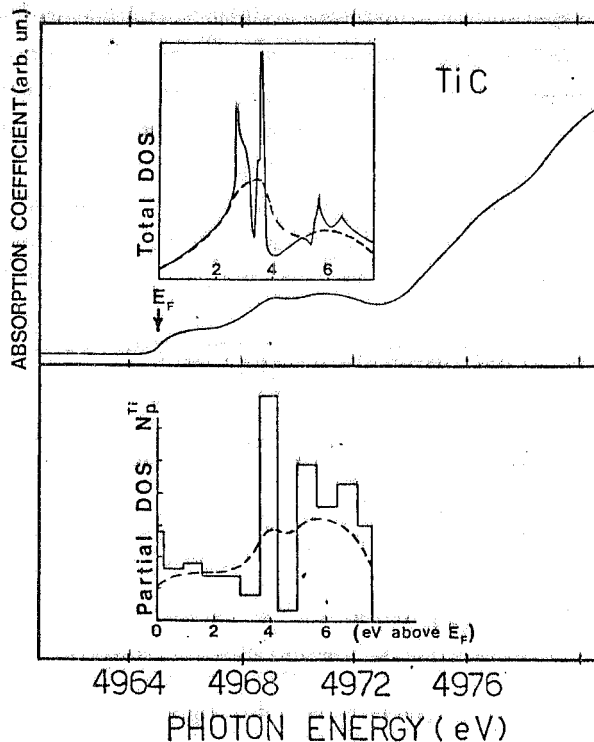
FIG. 4 - XANES of TiC on an expanded scale (solid curve). The upper and lower insets show the total and partial N_p^{Ti}(E) p-like DOS, respectively, after Neckel et al. 11 . The two curves are not drawn on scale. For their relative intensities, see Fig. 9. The dashed curves are as in Fig. 3.
