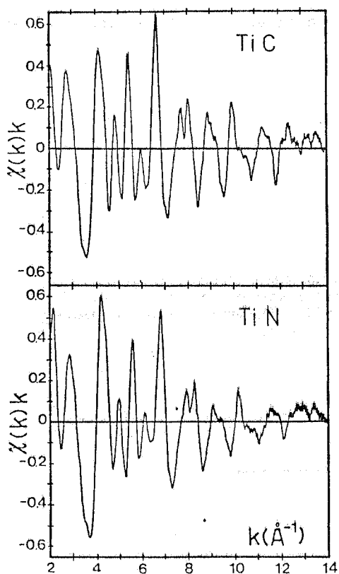
FIG. 19 - k \cdot \chi(k) EXAFS modulation of TiC and TiN above the Ti K-edge.
