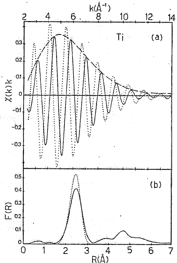
FIG. 16 - a) Backfourier transform k\chi(k) of the first peak of the radial distribution function F(R) of Ti (solid line) and its envelope function \tilde{A}(k) (dashed line). The dotted curve is a model k\chi(k) calculated from Eq. (7), using amplitudes and phases of Teo and Lee 65 , a Gaussian-like g_{ij}(r) and \sigma^2=0.007 \text{ \AA}^2 . The first two Ti shells, located at R_1=2.889 \text{ \AA} and R_2=2.941 \text{ \AA} 61 are considered. b) Fourier transform F(R) of the model k\chi(k) of part a) compared with experimental F(R) .
