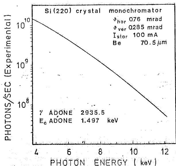
FIG. 1 - Photon flux measured at the exit of the Si(220) channel-cut monochromator. The source of radiation is the storage ring ADONE. \gamma represents the electron energy in units of electron rest energy m_0 c^2 and E_c is the critical energy. \phi_{hor} and \phi_{vert} are the horizontal and vertical angles with respect to the electron orbit plane seen by the detector. I_{stor} is the average current in the machine.
