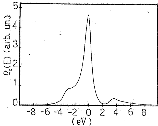
FIG. 12 - Auger core density of states \rho_c(E) according to Watts's theory 54 . The satellite peaks correspond to plasmon loss and gain at \pm \omega_p = 3.23 eV.
