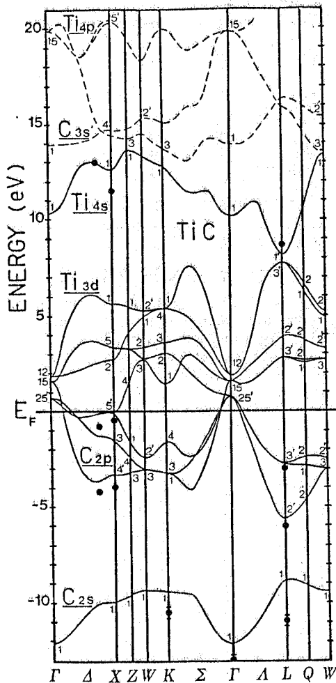
FIG. 6 - APW self-consistent valence and conduction bands of TiC after ref. 11 at high-symmetry points and along high-symmetry lines of the Brillouin zone. The dashed bands are those of Trebin and Bross. Full circles indicate the angular photoemission data of Weaver et al. 32 . The zero of the energy scale is at the Fermi level.
