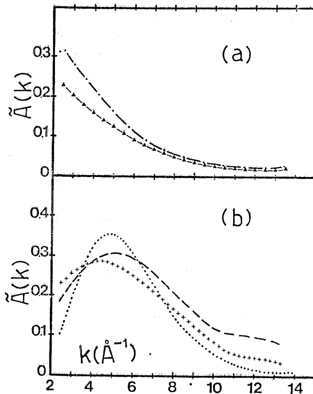
FIG. 22 - Experimental amplitudes for a) C and N atoms and b) Ti in Ti metal (dotted), in TiC (dashed) and in TiN (crosses).
