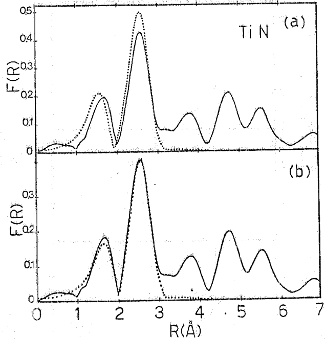
FIG. 23 - Comparison of the experimental F(R) for TiN with (a) model calculations based on Teo and Lee phases and amplitudes, and (b) experimental phases and amplitudes. Only the first two coordination shells (N and Ti) around the central Ti atoms are included.
