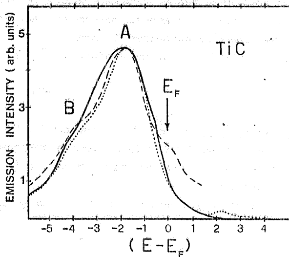
FIG. 13 - Comparison between the calculated L_{III} emission intensity of Ti in TiC (solid line) and the experimental curves from Fischer 13 (dotted) and Fischer and Baun 15 (dashed). The zero of the energy scale is at the Fermi edge.
