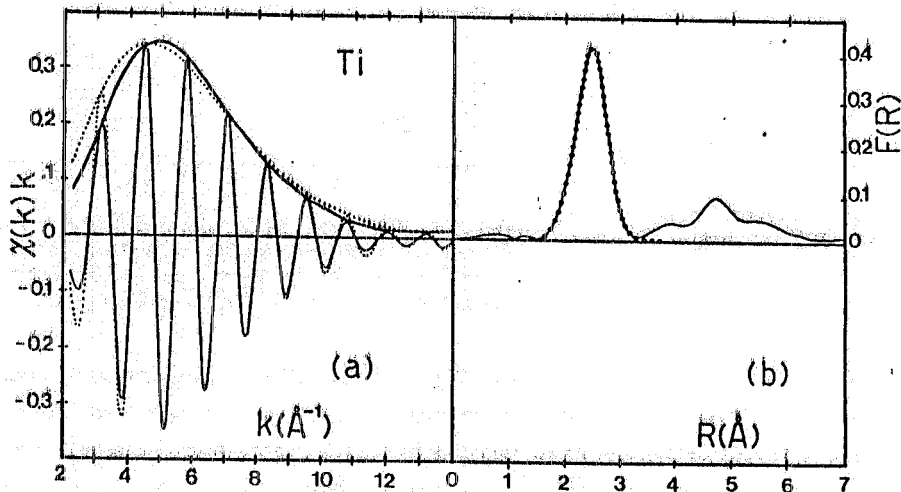
FIG. 18 - a) Model k\chi(k) and \tilde{A}(k) (dotted lines) computed from Eq. (7) using the reduced S_0^2 = 0.85 amplitudes of Teo and Lee 65 and experimental phases. The other parameters are as in Fig. 16. The solid curve is the experimental k\chi(k) . b) F(R) deduced from the model k\chi(k) of part a) (dots) compared with the experimental F(R) .
