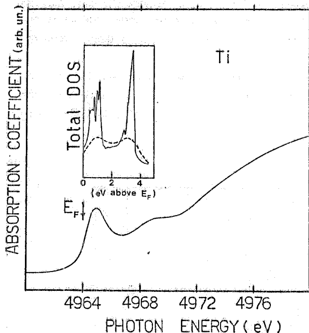
FIG. 3 - XANES of Ti metal on an expanded scale. The total-mainly-d-like-DOS calculated by Jepsen 26 is shown in the inset. The dashed curve represents the convolution with a Lorentzian function with a FWHM of 1.3 eV.
