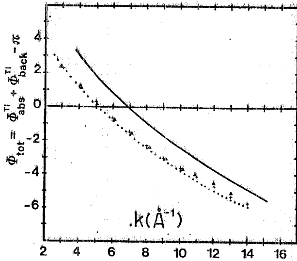
FIG. 17 - Total phase shift \Phi vs. k for the Ti-Ti pair in Ti metal (dotted line), TiC ( \Delta ) and TiN (+). The Teo and Lee theoretical phase is shown for comparison (solid line).
