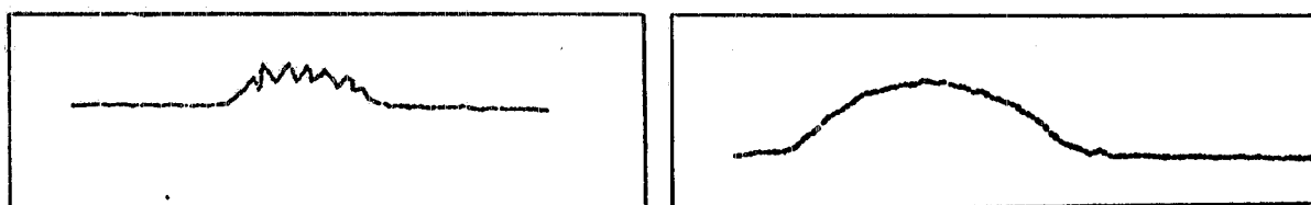
FIG. 7 - A) Modulation effect in the first version of the chamber with a non collimated beam; periodicity: 2 mm.; B) Modulation effect is suppressed by using the present version of the chamber with a \square -shaped electrode.
