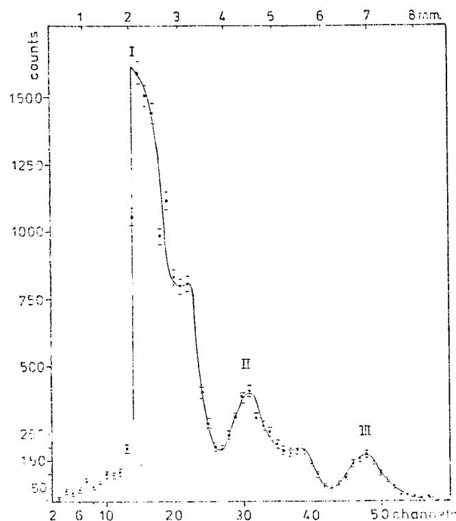
FIG. 10 - Small-angle diffraction pattern from dry tendon collagen. Diameter of the collimator pin-holes: 0.5-0.7 mm; \lambda=3.44 Å; recording time: 180 min; 1 channel=0.144 mm; collagen spacing obtained from these data: 640 Å.
