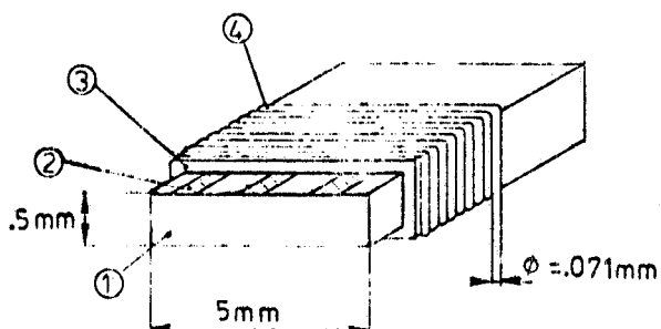
FIG. 8 - Schematic cross-section of delay-line. 1) Fiber-glass frame; 2) earthed copper strips; 3) thermoplastic film; 4) coil. Electrical characteristic: 1) length: 8 \text{ cm} ; 2) characteristics impedance Z_0 : 2.2 \text{ K}\Omega ; delay: 12 \text{ nsec/cm} ; delay/rise-time: 13.
