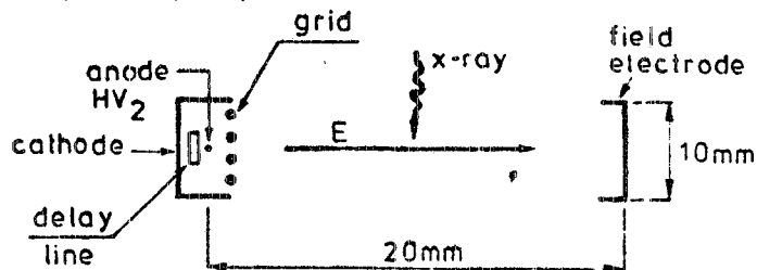
FIG. 1 - Scheme of the drift chamber.
