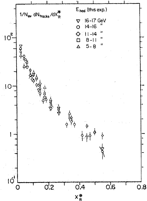
Fig. 1. Normalized single-particle inclusive distribution ( 1/N_{\text{ev}} ) ( dN/dx_R^* ) versus x_R^* for various bands of E_{\text{had}} , obtained from p-p collisions.
