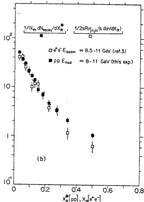
Fig. 2. The p-p single-particle inclusive distributions in terms of the variable X_R^* , are compared to the single-particle inclusive distributions obtained in e^+e^- annihilation; (a) E_{had} = 5-8 GeV, (b) E_{had} = 8-11 GeV, (c) E_{had} = 14-16 GeV.
