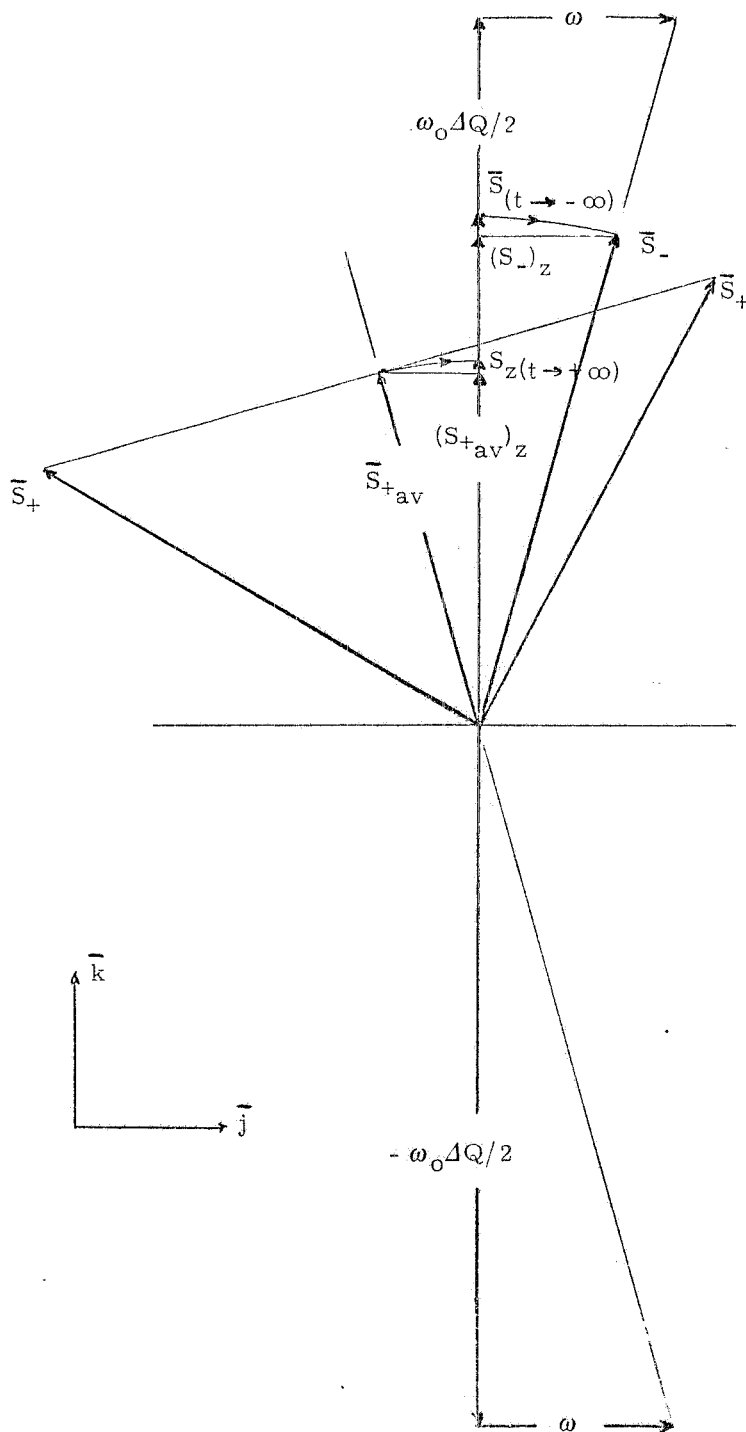
FIG. 1 - Vector diagram, in the (y, z) plane, showing the variations of \bar{S} during the whole time interval -\infty < t < +\infty in the case where a Q-jump is applied in the vicinity of an intrinsic spin-resonance. See text for the meaning of the symbols.
