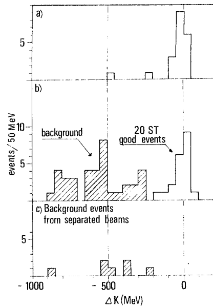
FIG. 2. \Delta K = K_{rec} - K_{meas} distribution (a) for ten DT- \mu events; (b) for 56 ST- \mu events; (c) for seven ST background \mu events obtained with separated e^+ and e^- beams. 36 of the 56 ST events in (b) can be interpreted as background events. Of course each doubly tagged event contributed two points to the \Delta K distribution.
