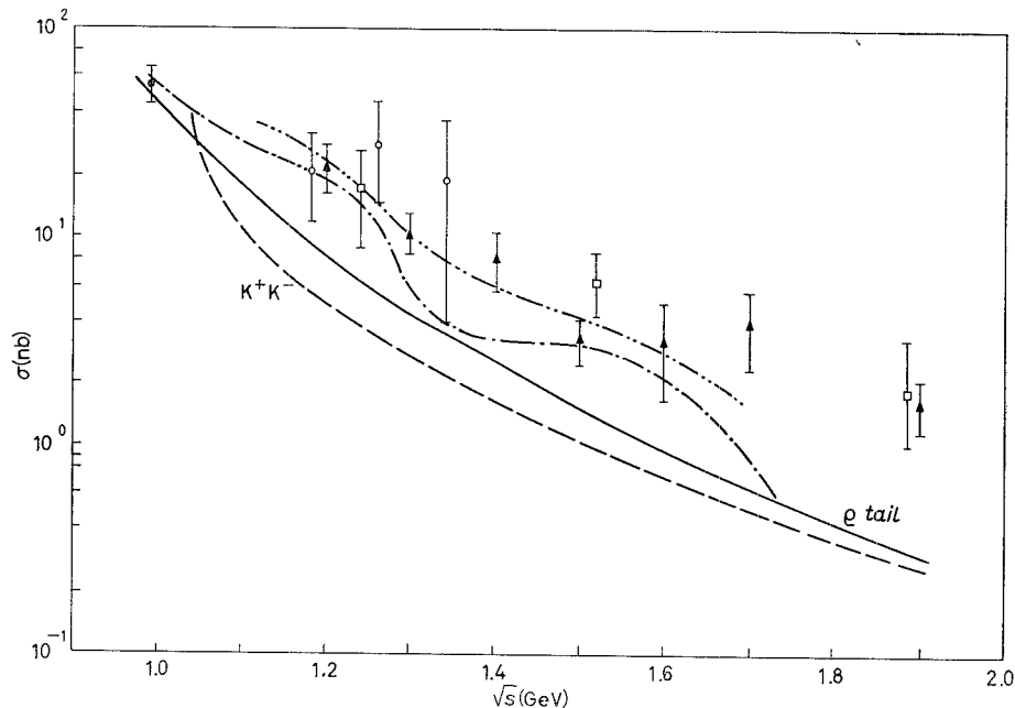
Fig. 2. - Total cross-section \sigma(s) for the process e^+e^- \rightarrow \pi^+\pi^- as a function of the centre-of-mass energy \sqrt{s} . The experimental data are taken from ref. (11). The different curves correspond to: — extrapolation of the Orsay fit (Gounaris and Sakurai formula) which includes \rho - \omega interference; --- \rho , \omega and \phi tails to K^+K^- production; -.-.- \rho'(1250) , \rho''(1600) contributions plus —; ..... the sum of ..... and —. • ACO, ○ VEPP, ▲ ADONE BCF, □ ADONE \mu\pi .
