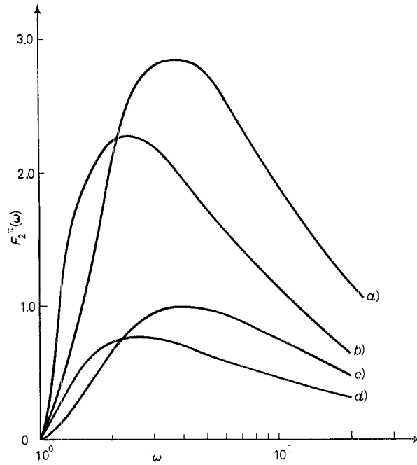
Fig. 1. - Plot of the pion structure functions for various values of the parameters \langle n_\pi \rangle and R .
