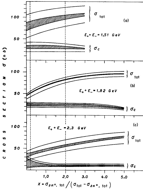
FIG. 18. Reactions e^+e^- \rightarrow a^\pm + b^\pm + \text{anything} . The total cross section, \sigma_{\text{tot}} , and \sigma_c = \sigma_{4\pi^\pm} + \sigma_{6\pi^\pm} are given as functions of the parameter
