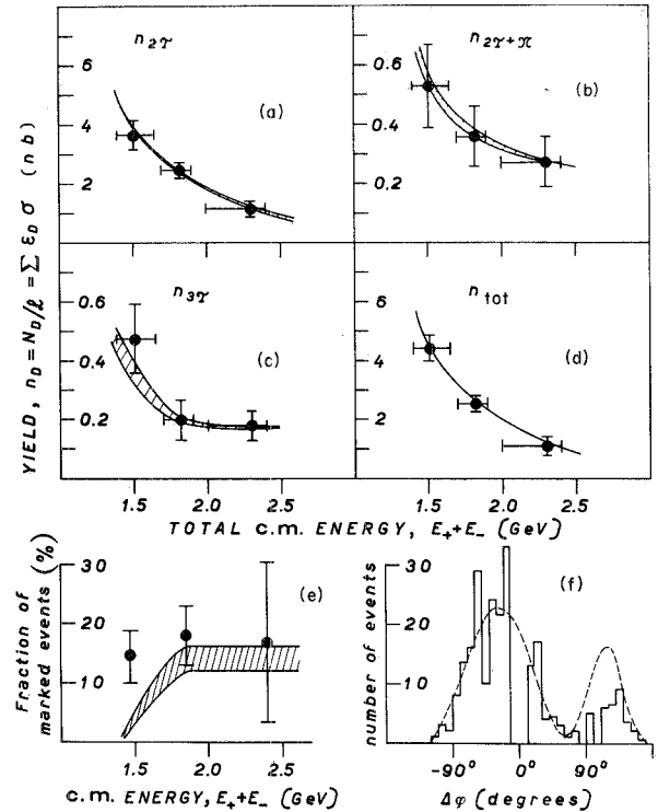
FIG. 21. Comparison of the experimental data on the reactions e^+e^- \rightarrow a^\pm + b^\pm + \text{anything} with the results of the fit (shown as curves and dashed bands in the figure). (a) Yield of two charged detected tracks events; (b) yield of two charged plus one neutral detected tracks events; (c) yield of three charged detected tracks events; (d) total yield (all the detected configurations); (e) fraction of marked events; (f) \Delta\phi distribution of two charged track events (4-chm events).
