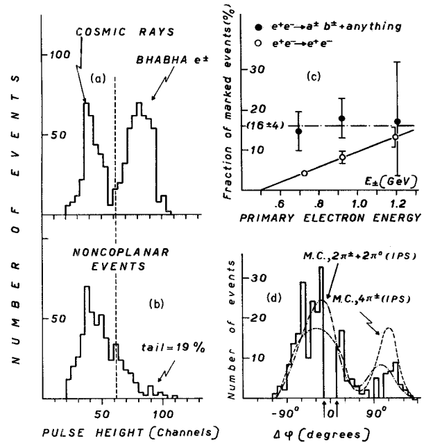
FIG. 13. (a) Cosmic-ray and Bhabha electrons pulse-height spectra in telescope T_1 ; (b) pulse-height distribution of in-time, in-source, noncoplanar events in telescope T_1 ; (c) fraction, f_M , of marked noncoplanar and Bhabha events; (d) \Delta\phi distribution of the two charged track, 2T , background-subtracted, 4-chm noncoplanar events compared with an IPS Monte Carlo calculation for two possible pion final states.
