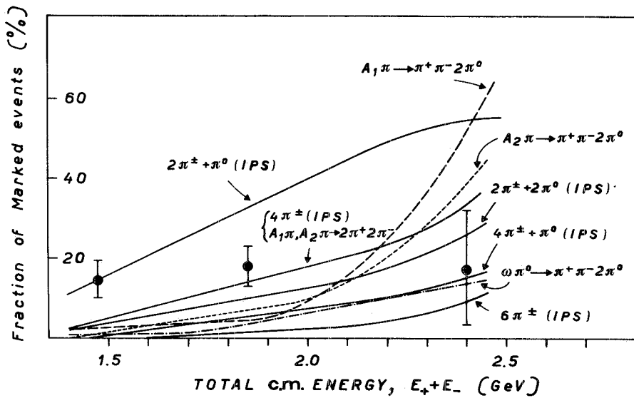
FIG. 24. Fraction of marked events, f_M , calculated with the Monte Carlo program for several different processes, compared with the experimental values for the reactions e^+e^- \rightarrow a^\pm + b^\pm + \text{anything} .
