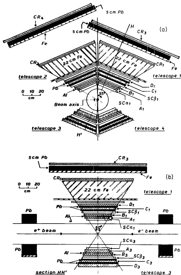
FIG. 1. The experimental apparatus. (a) Section orthogonal to the beam axis: A_i, B_i, C_i, D_i are plastic scintillation counters; SC\alpha_i and SC\beta_i are magnetostrictive monogap wire chambers; CR_i 's are veto counters for cosmic rays. (b) Section (along H, H' ) in a plane through the beam direction and orthogonal to a pair of opposite telescopes.
