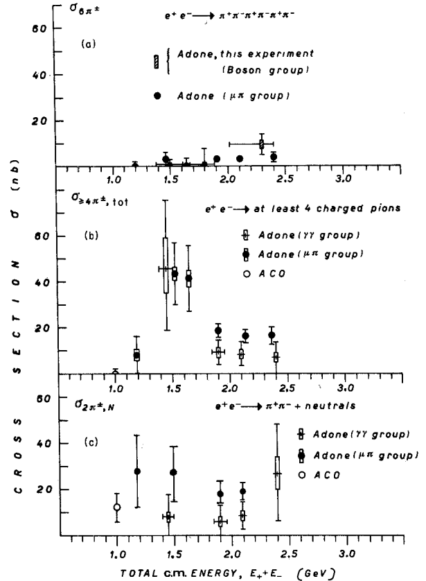
FIG. 23. Summary of the experimental determinations of the cross sections for reactions e^+e^- \rightarrow a^\pm + b^\pm + \text{anything} . Our results are compared with the data from ACO (Ref. 35), the Adone \gamma\gamma Group (Ref. 37), and the Adone \mu\pi Group (Ref. 38). Systematic uncertainties are indicated as rectangles. (a) Cross section to produce six charged pions \sigma_{6\pi^\pm} ; (b) cross sections to produce at least four charged pions (plus possible neutrals), \sigma_{4\pi^\pm, \text{tot}} ; (c) cross sections to produce two charged pions plus neutrals, \sigma_{2\pi^\pm, N} .
