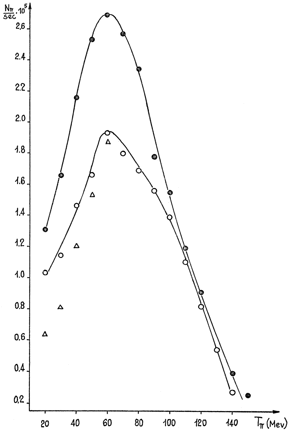
FIG. 3 - Experimental results obtained with pion beams on :
