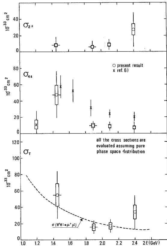
Fig. 2. Results on \sigma_T (total cross section for reactions (1)), \sigma_{4\pm} (reactions (3)), \sigma_{2\pm} (reactions (2)) as a function of 2E , total energy in c.m. system. The rectangles indicate a reasonable estimate of the width of our possible systematic errors. The bars represent the statistical errors. All these values are obtained under the assumption of a pure invariant phase space distribution: the limitations of this model are discussed in the text. The dashed line indicate the total cross section for the process e^+ + e^- \rightarrow \mu^+ + \mu^- .
