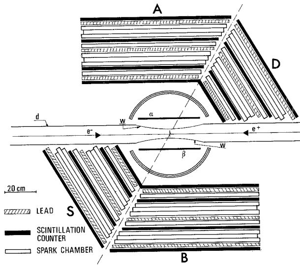
Fig. 1. Experimental apparatus: front view from Adone center. d: doughnut; w: 0.15 mm stainless steel window.
