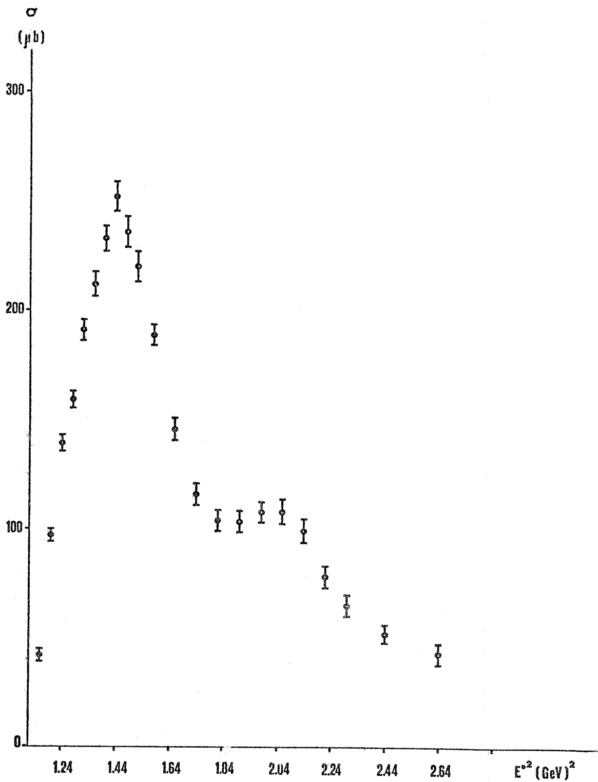
FIG. 12 - A maximal value of the total cross-section with the hypothesis that all the observed \gamma D \rightarrow pp\pi^- events could be considered as \gamma n events (see text).
