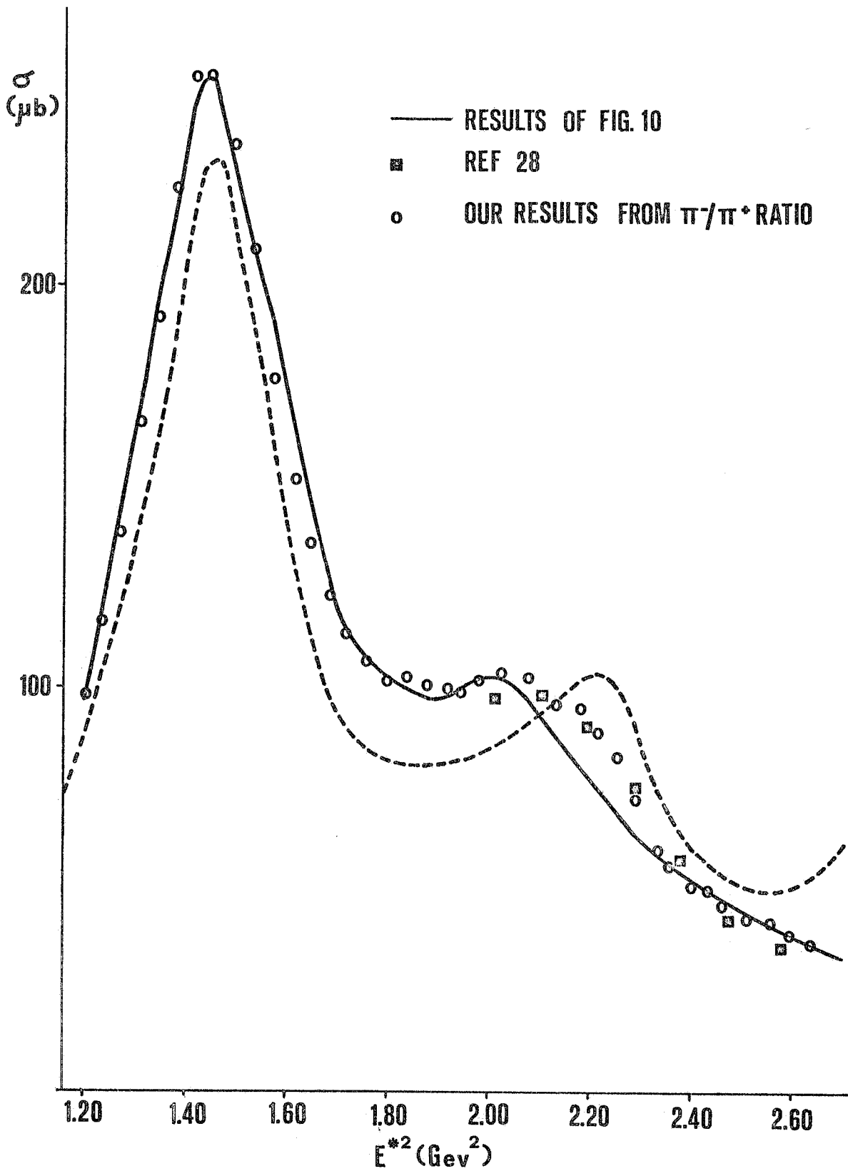
FIG. 17 - Total cross-section of the reaction \gamma n \rightarrow p\pi^- . The \pi^+ photoproduction cross-section is also reported (dashed line).
