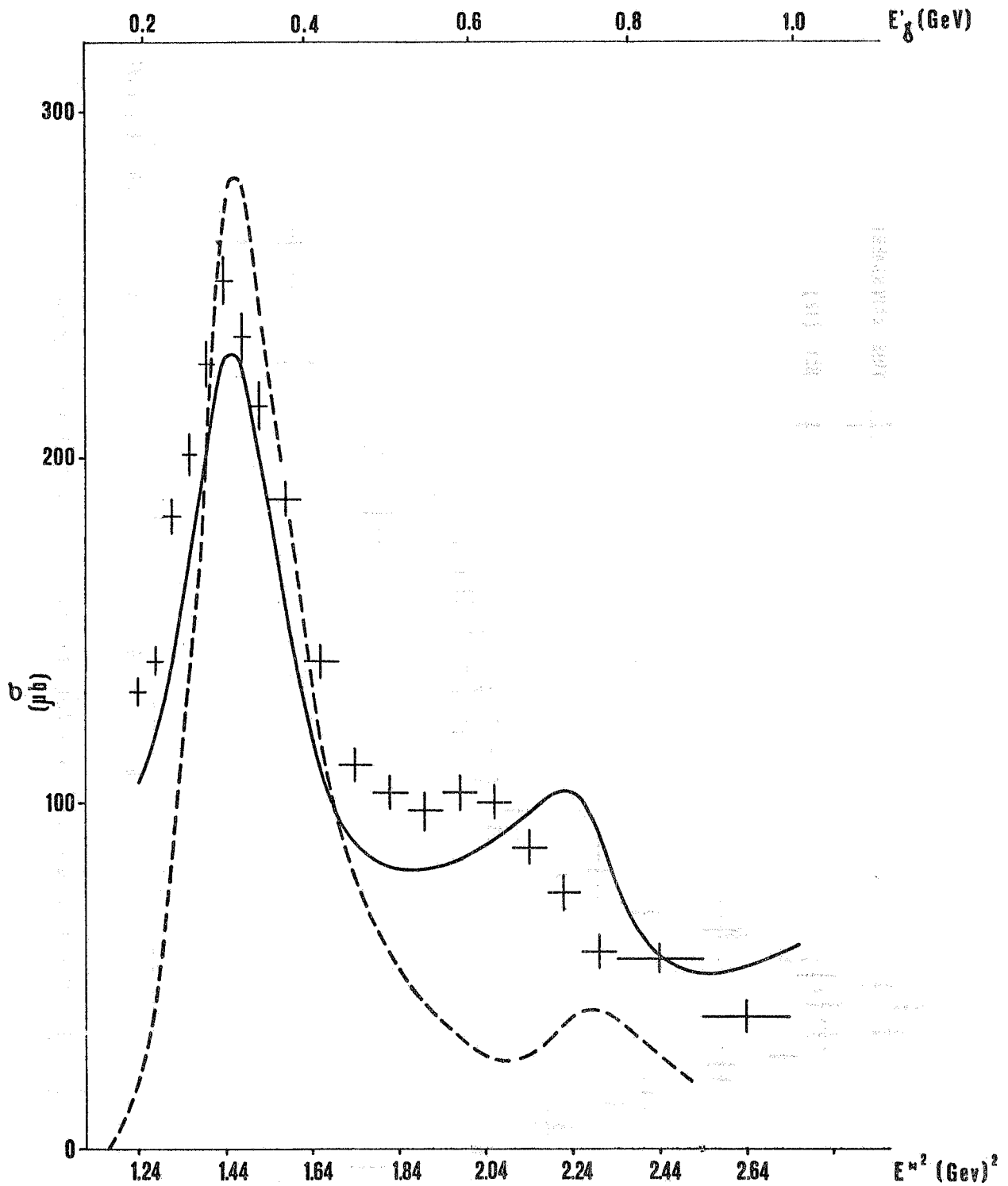
FIG. 10 - Total cross-section for the reaction \gamma + n \rightarrow p + \pi^- . The superimposed curves are the cross-sections for \gamma p \rightarrow p\pi^0 (dashed line) and \gamma p \rightarrow n\pi^+ (full line).
