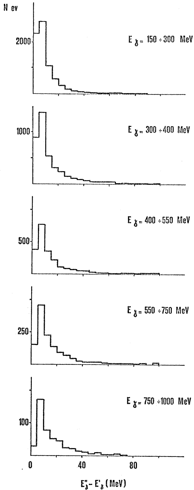
FIG. 8 - Differences between the effective photon energies, as obtained by the Lorentz transformation E''_{\gamma} , and the final state ( \pi^-p ) total energy E'_{\gamma} (see text), for various E_{\gamma} (in the L. s.) intervals.
