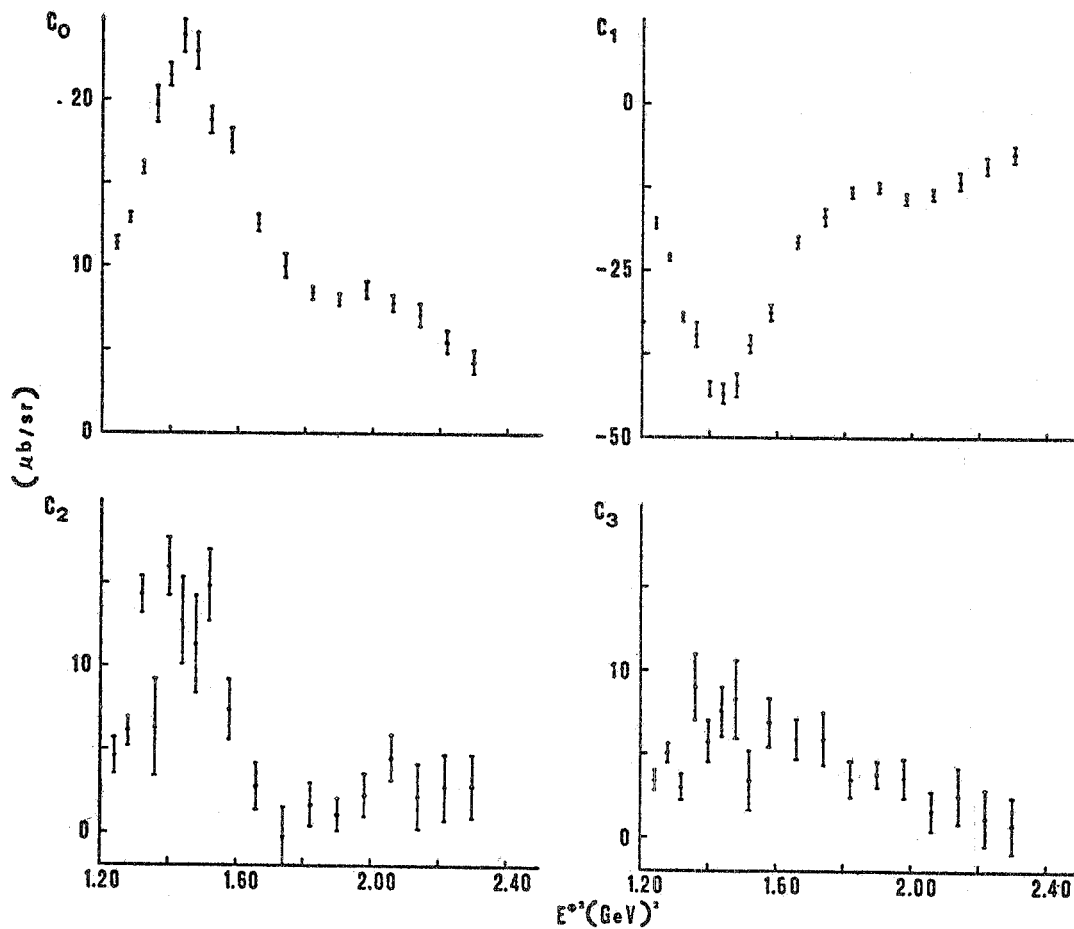
FIG. 13 - Behaviour of the coefficients of the Moravcsik polynomial fit to the angular distributions, as a function of E^{*2}
