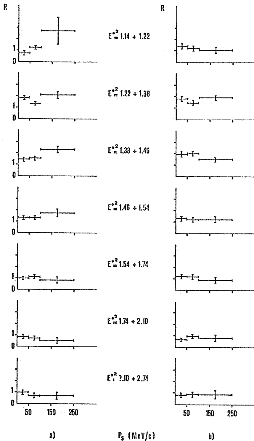
FIG. 14 - Ratios R between the \pi^- in the backward and in the forward directions (c. m. s.) as a function of p_s
