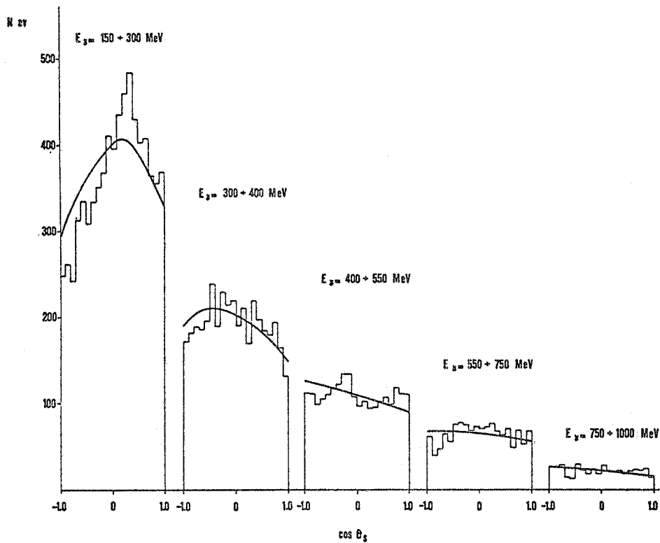
FIG. 7 - Same as fig. 4, but after the \theta_S^* cut.
