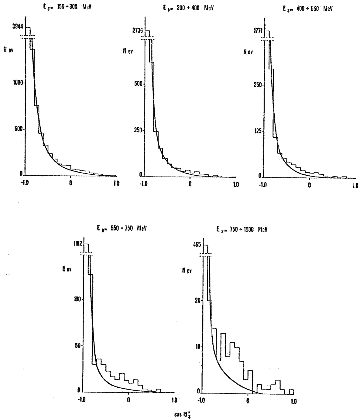
FIG. 5 - Angular distribution of the spectator proton in the \gamma D c.m.s. The curves show the predictions of the spectator model.
