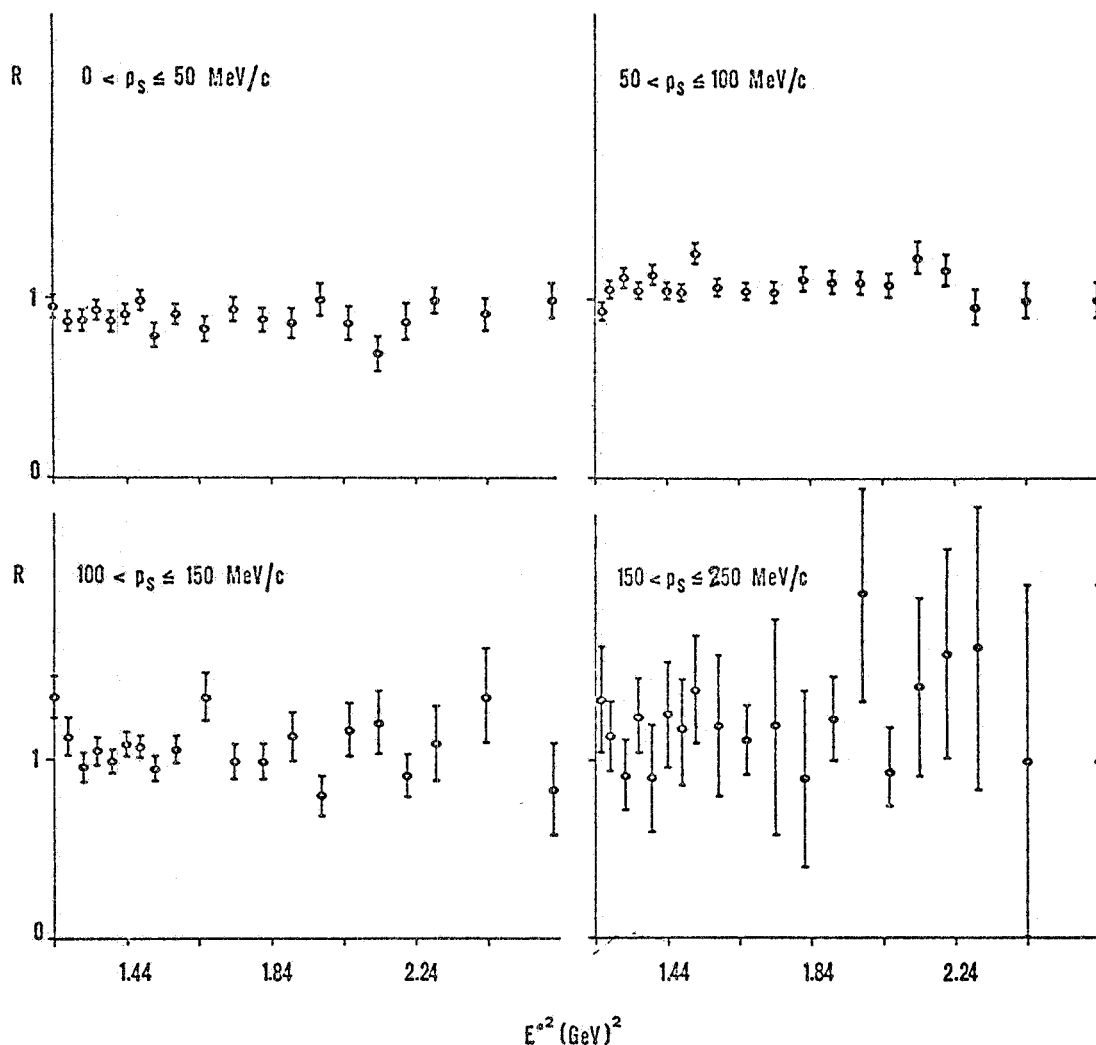
FIG. 11 - Plots of the ratios R = \sigma(p_0, 250)/\sigma(p_a, b) vs E^{*2} , where \sigma(p_a, b) is the cross-section value, obtained by the events with a \leq p_s \leq b .
