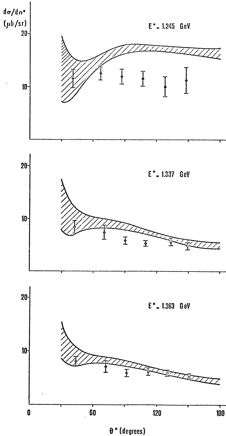
FIG. 16 - Comparison between the differential cross-sections for \pi^-p \rightarrow n\gamma (points from ref. 21) and \gamma n \rightarrow \pi^-p (shaded band).
