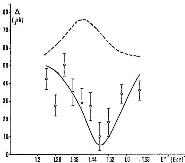
FIG. 15 - \Delta = q/K \left[ \sigma_T(\gamma n \rightarrow p \pi^-) - \sigma_T(\gamma p \rightarrow n \pi^+) \right] as a function of E^{*2} . The curves are the predictions (18) with x = 0.20 (full line) and x = 0 (dashed line).
