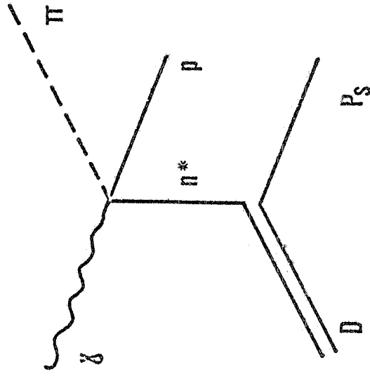
FIG. 2 - Diagram assumed to describe the reaction (1), according to the spectator model.
