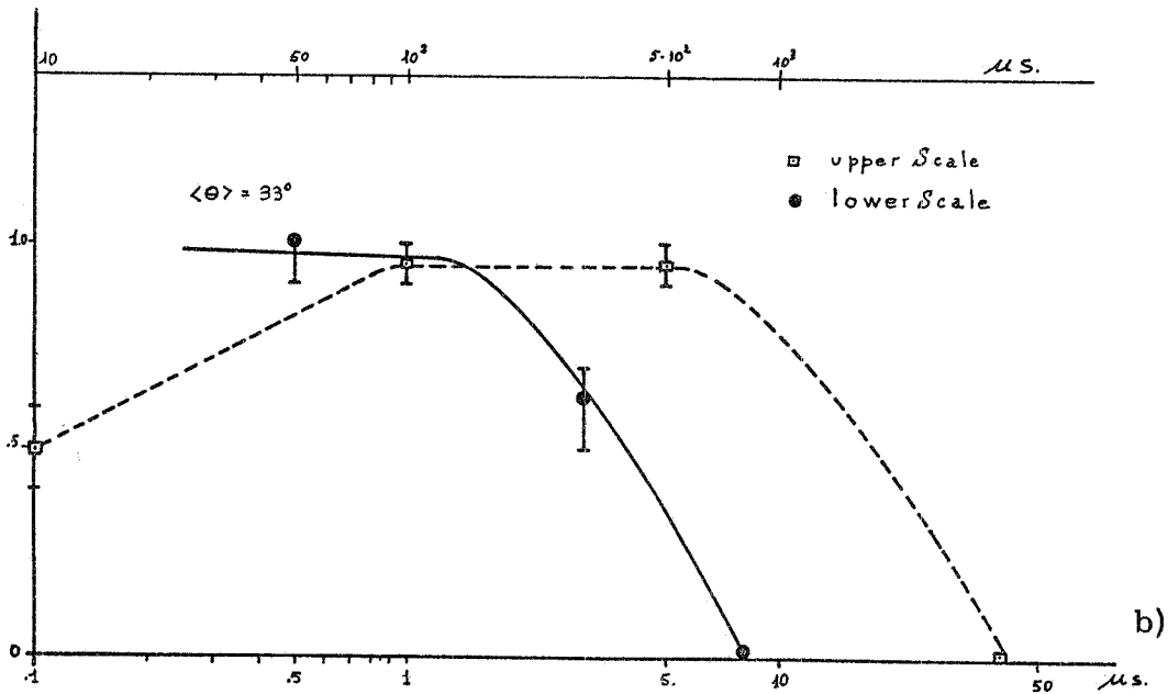
FIG. 6 - Comparison of storage and memory curves; Fig. 6a) shows the memory curve (dashed line) and storage curve (solid line) with a gas flow of 3 lt/hours; Fig. 6b) shows the same curves but with a gas flow of 1.5 lt/hours. However all other conditions are the same as in Fig. 3.
