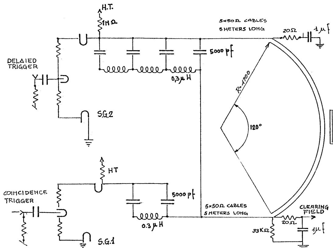
FIG. 7 - Experimental set-up for narrow gap tests.
