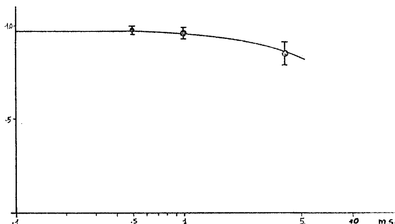
FIG. 4 - SC 1 efficiency versus Marx 2 delay in the same condition of 3b) but with \theta = 0^\circ .
