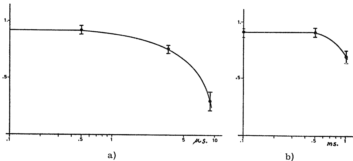
FIG. 3 - a) SC 1 efficiency versus Marx 2 delay with Marx 1 off; for 33^\circ \pm 5^\circ tracks the gas is neogal (80% Ne, 20% He) saturated with water vapours, E_2 = 6 KV/cm. - b) SC 1 efficiency versus Marx 2 delay in the same condition of a) but with Marx 1 on. E_1 = 10 KV/cm, \tau_1 = 40 nsec, E_2 = 8.8 KV/cm, \tau_2 = 200 nsec.
