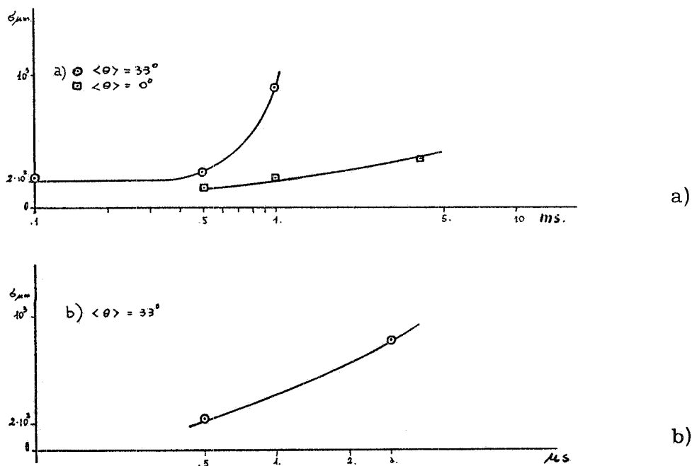
FIG. 5 - Spark distortion: a) versus Marx 2 delay in the same condition of 3b); - b) versus Marx 2 delay with Marx 1 off. These numbers are averaged on about one hundred sparks for every point.
