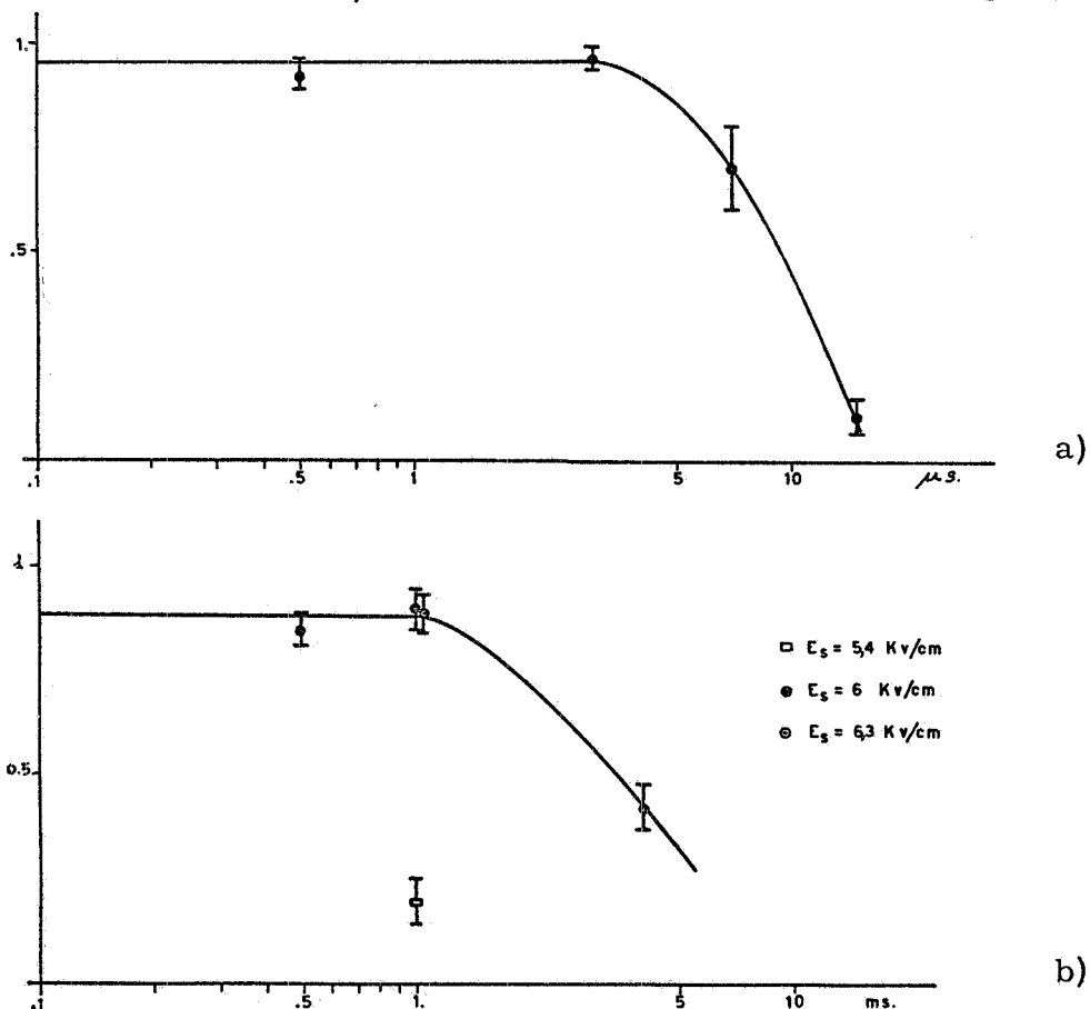
FIG. 2 - a) SC_1 efficiency versus Marx 2 delay, Marx 1 is off, the gas is henogal (80% He, 20% Ne) and E_2 = 6 KV/cm. - b) SC_1 efficiency versus Marx 2 delay with Marx 1 on, for various storage pulses amplitude, in the same condition of Fig. a); \tau_1 is 220 nsec and \tau_2 is 1100 nsec.
