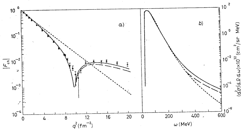
Fig. 1. - a) Elastic and b) quasi-elastic ( \epsilon = 600 MeV, \theta = 10^\circ ) electron scattering cross-sections for {}^4\text{He} . The dashed curves represent predictions without correlations where the oscillator parameter \alpha = 156 MeV is used. The solid curves correspond to the hard-core interaction with C = 0.56 fm, B = 0.77 fm ^{-1} , while the dashed curves are given by the soft-core correlation with C = 0 , B = 0.64 fm ^{-1} . Elastic experimental data are taken from ref. (15) .
