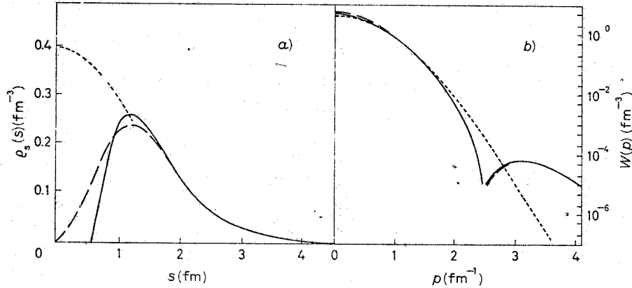
Fig. 2. - a) The separation density and b) momentum distribution in {}^4\text{He} . The three types of curves correspond to the correlations described in the caption of Fig. 1.
