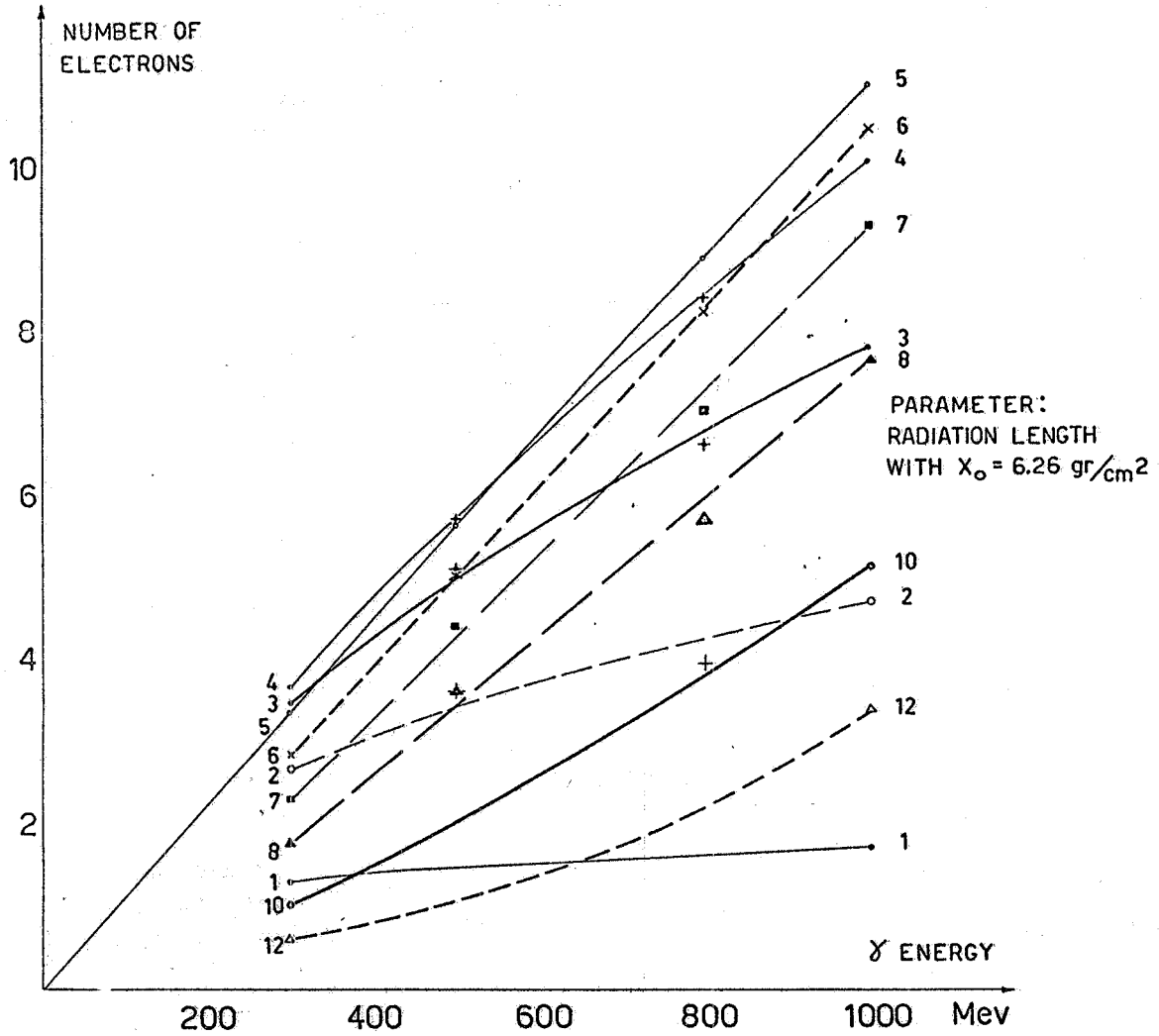
FIG. 1 - Pb showers generated by photons: charge multiplicity versus incident \gamma energy, the converter thickness as a parameter. The data have worked out by the authors from the quoted reference.
