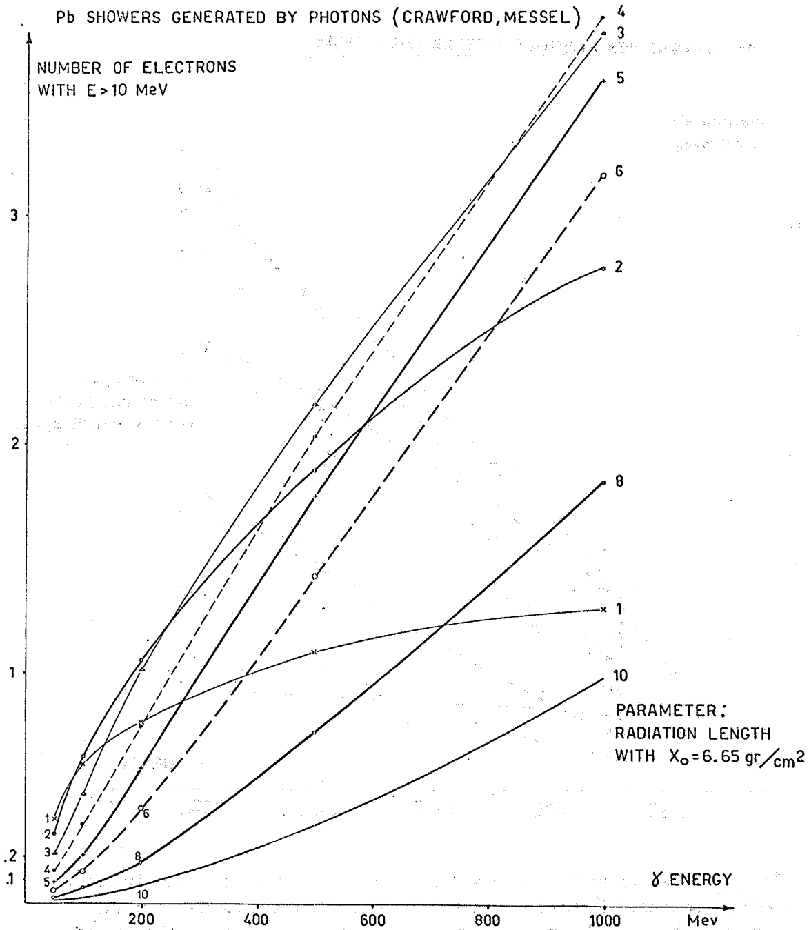
FIG. 2 - Pb showers generated by photons: charge multiplicity versus incident \gamma energy, the converter thickness as a parameter. The data have worked out by the authors from the quoted reference.
