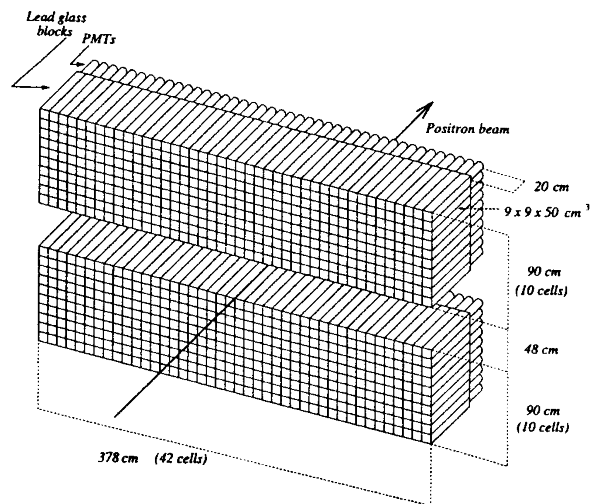
Fig. 1. Isometric view of the HERMES calorimeter.
