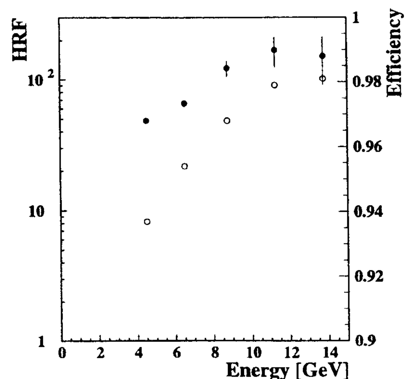
Fig. 11. Off-line hadron rejection factors for the system calorimeter + pre-shower (full circles and left scale) and corresponding efficiencies (empty circles and right scale).
