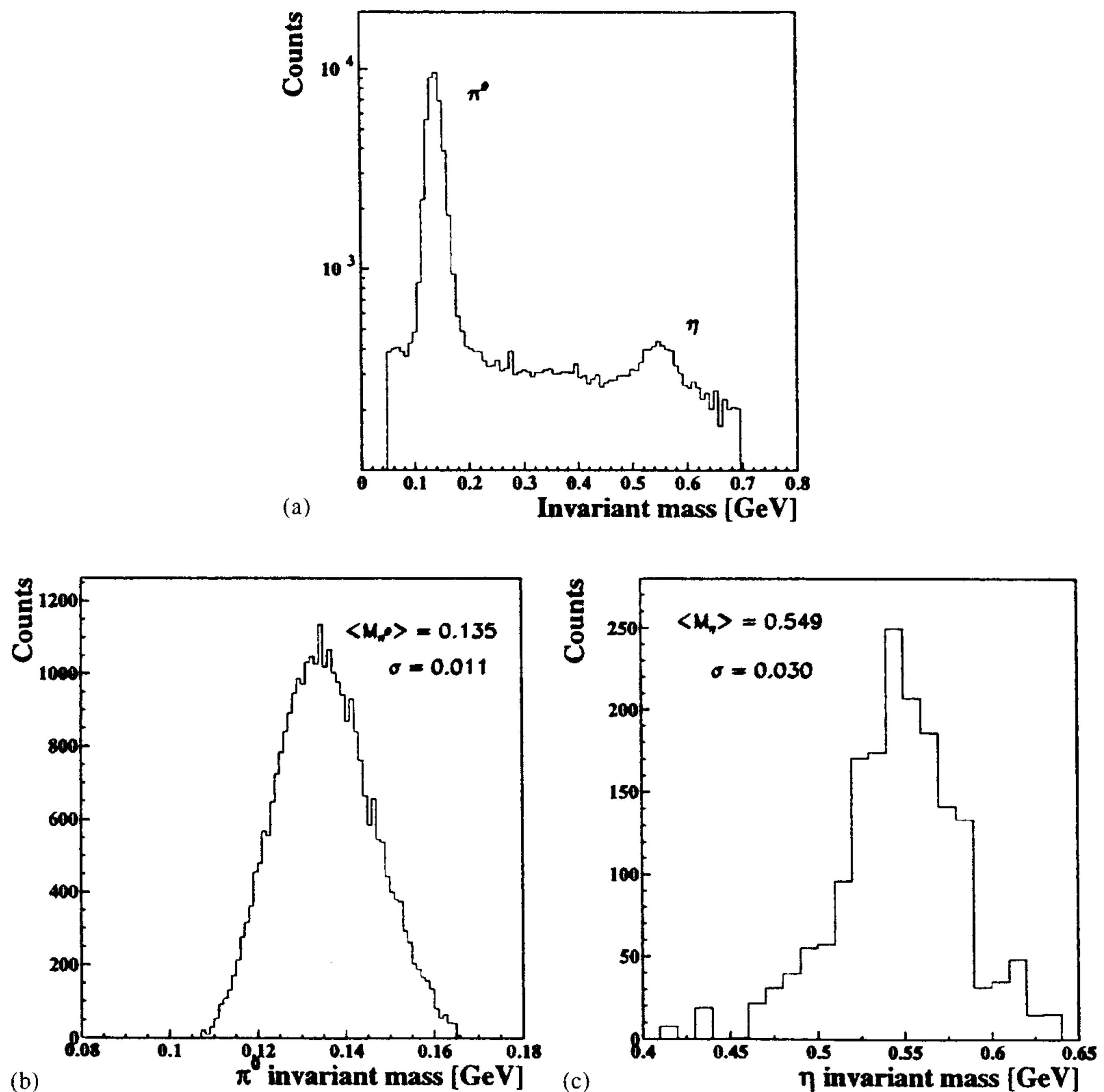
Fig. 12. Two-photon invariant mass distribution in the calorimeter: (a) peaks of \pi^0 and \eta ; (b) and (c) peaks of \pi^0 and of \eta , respectively, after applying kinematical cuts and background subtraction.
