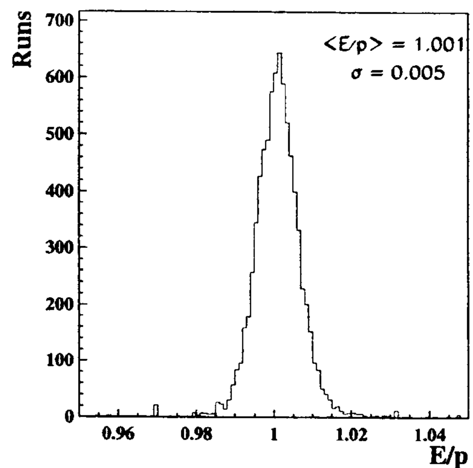
Fig. 9. E/p averaged distribution for all lead-glass blocks over a one-year of data taking period.
