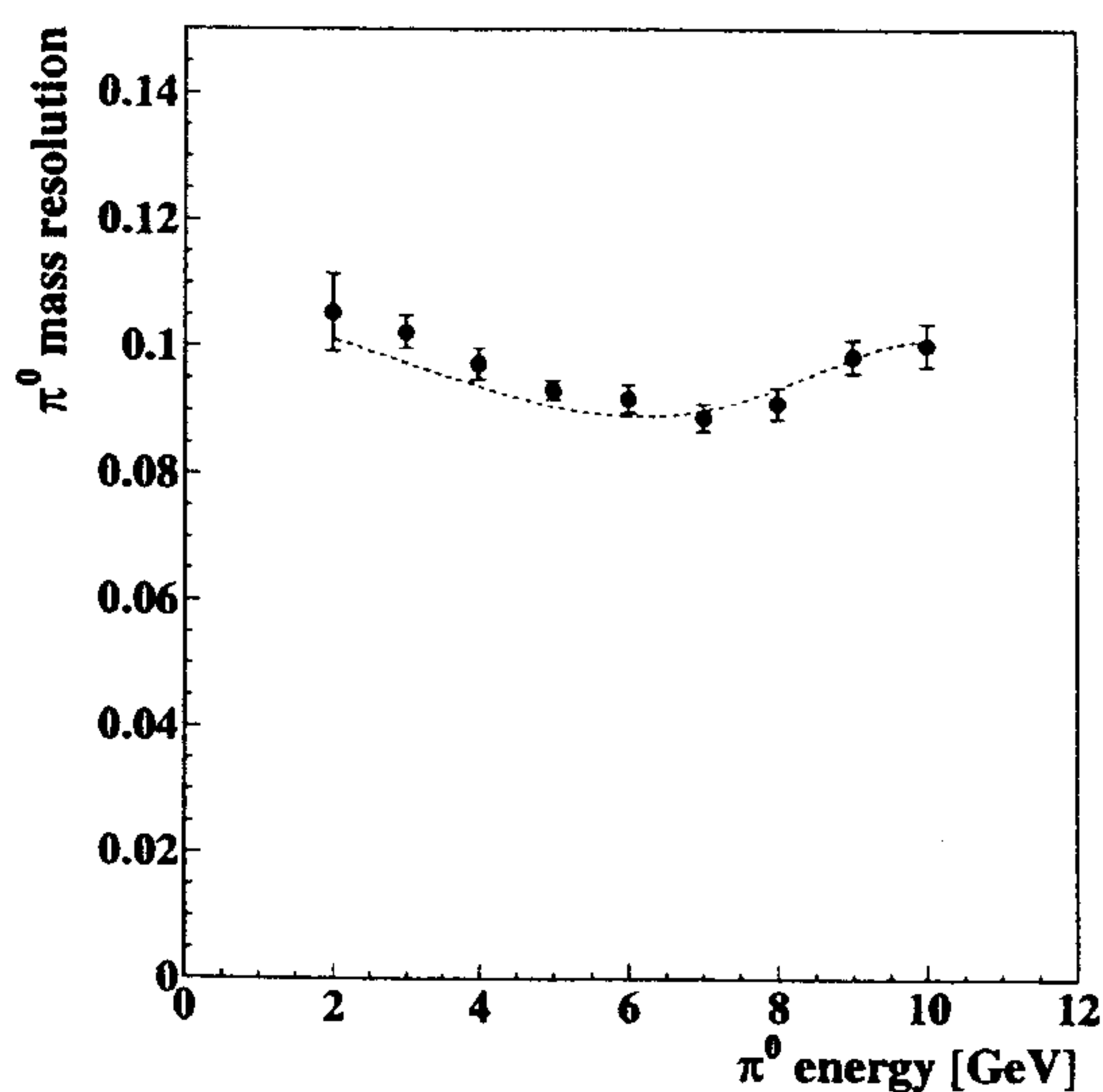
Fig. 13. Resolution of the \pi^0 invariant mass as calculated from the measured energy and position resolutions of two-photon events in the calorimeter (dashed curve), compared to the values obtained from semi-inclusive DIS events (closed circles).
