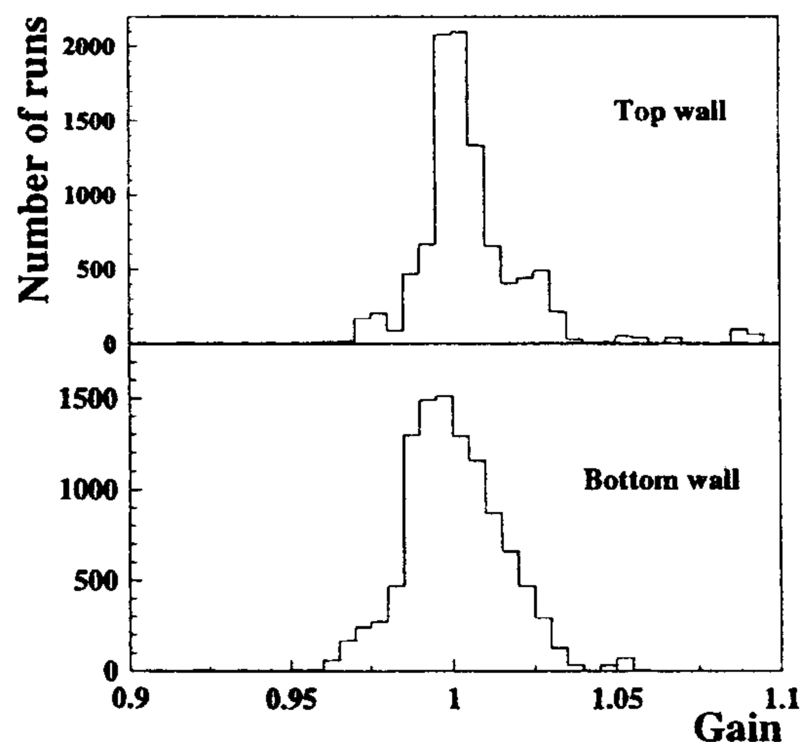
Fig. 10. Distribution of the relative gain from the GMS for calorimeter blocks located in the vicinity of the beam.
