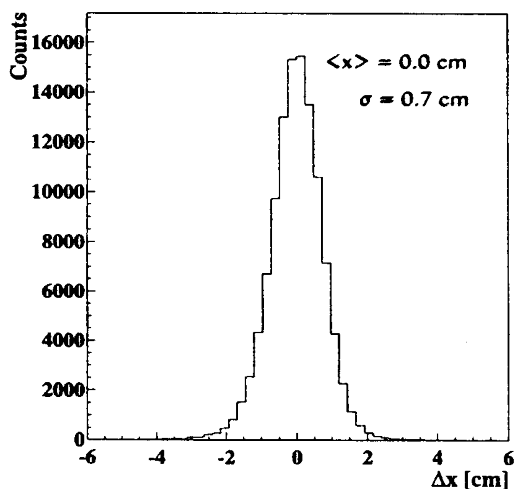
Fig. 6. Distribution of the differences \Delta x = x_{\text{calo}} - x_{\text{track}} between the hit positions measured by the calorimeter and those determined by the spectrometer.
