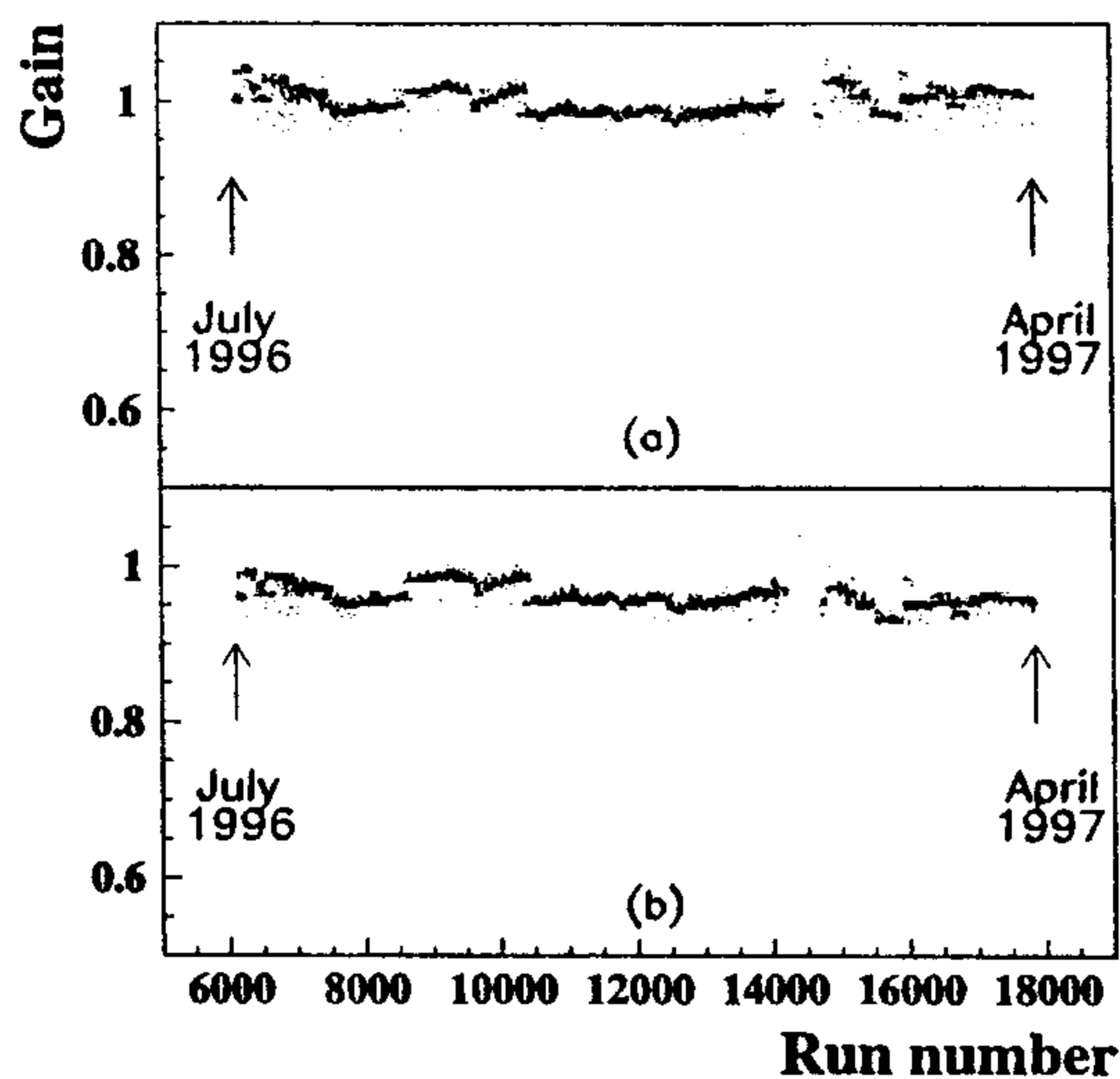
Fig. 8. Relative gain variations of two typical PMTs of the lead glass counters measured during the 1996 and part of 1997 data taking periods (a typical length of a run is about 10 min.); (a) counter from top calorimeter wall, (b) counter from bottom calorimeter wall.
