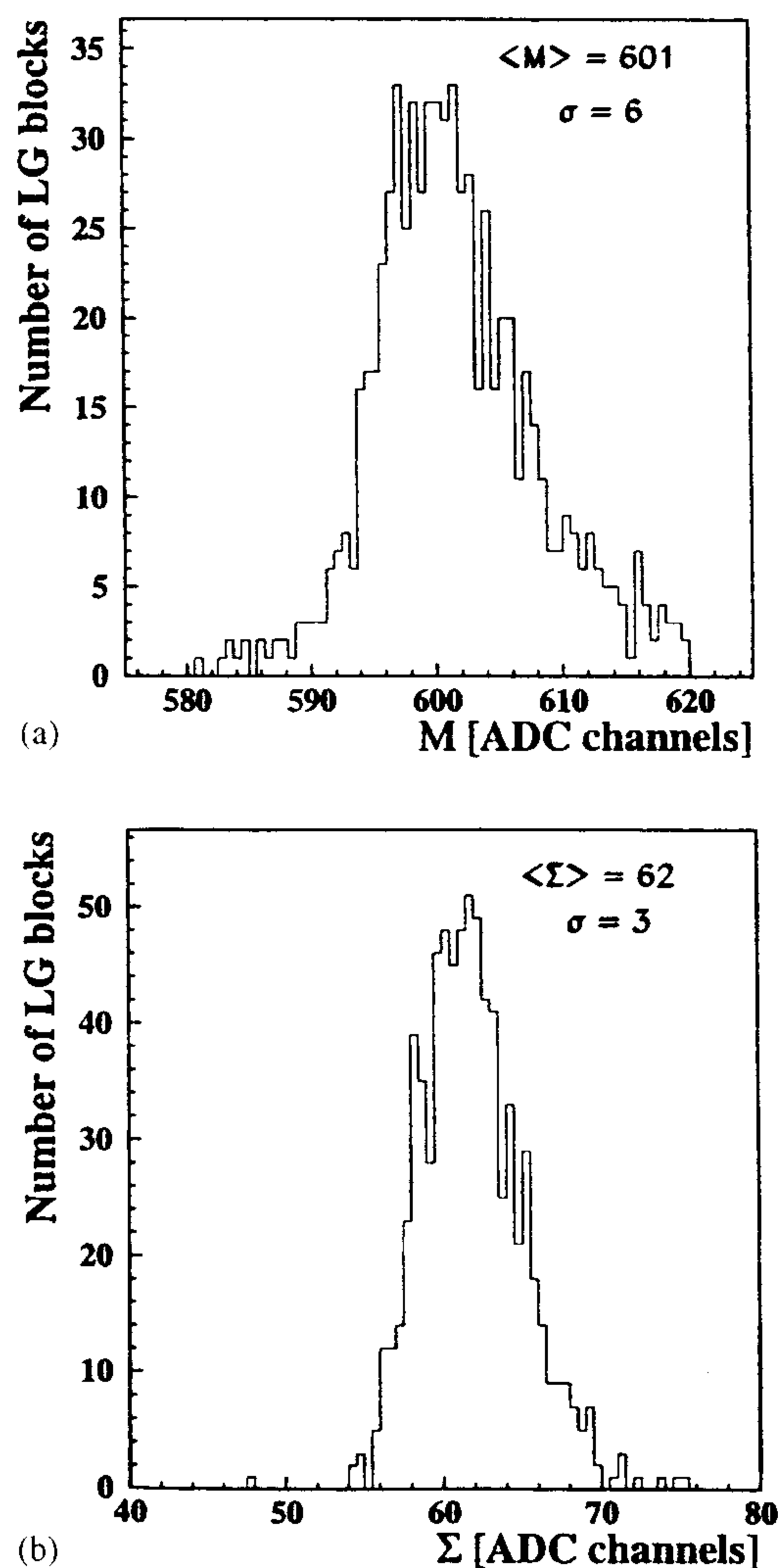
Fig. 2. Equalization of the 840 lead-glass (LG) blocks in a 3 GeV electron beam: (a) distribution of the mean M ADC values; (b) distribution of the standard deviation \Sigma of ADC values.
