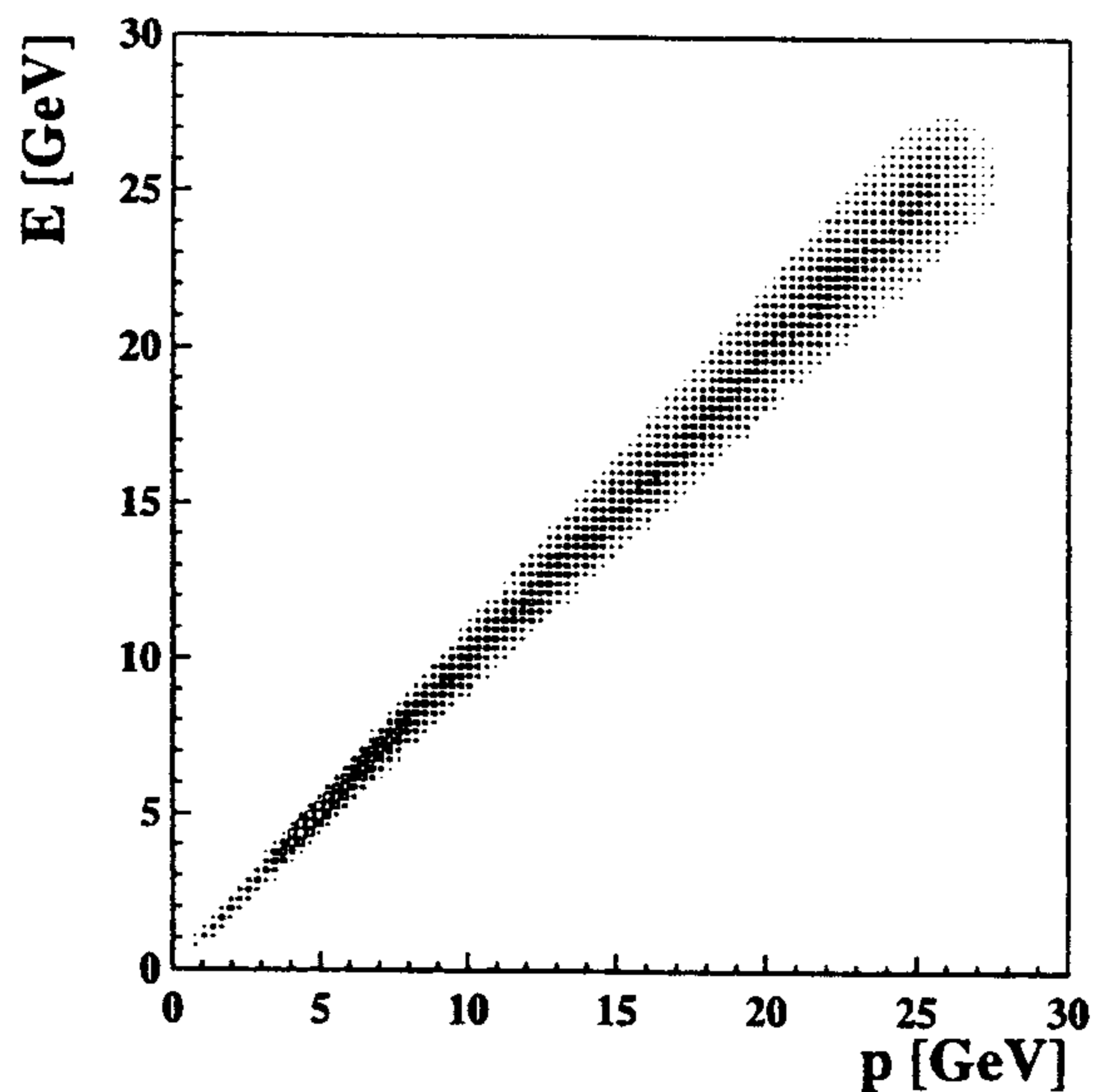
Fig. 3. Positrons energies E measured by the calorimeter versus the positrons momenta p reconstructed in the spectrometer during data taking.
