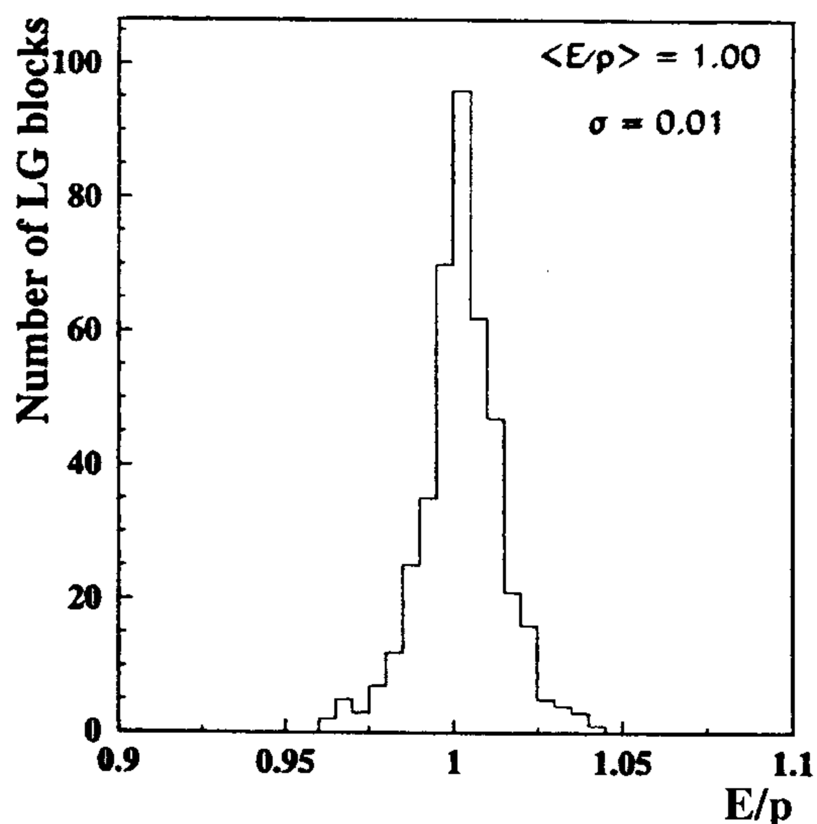
Fig. 4. Distribution of the E/p values measured for each counter for all runs collected over one year data taking period.
