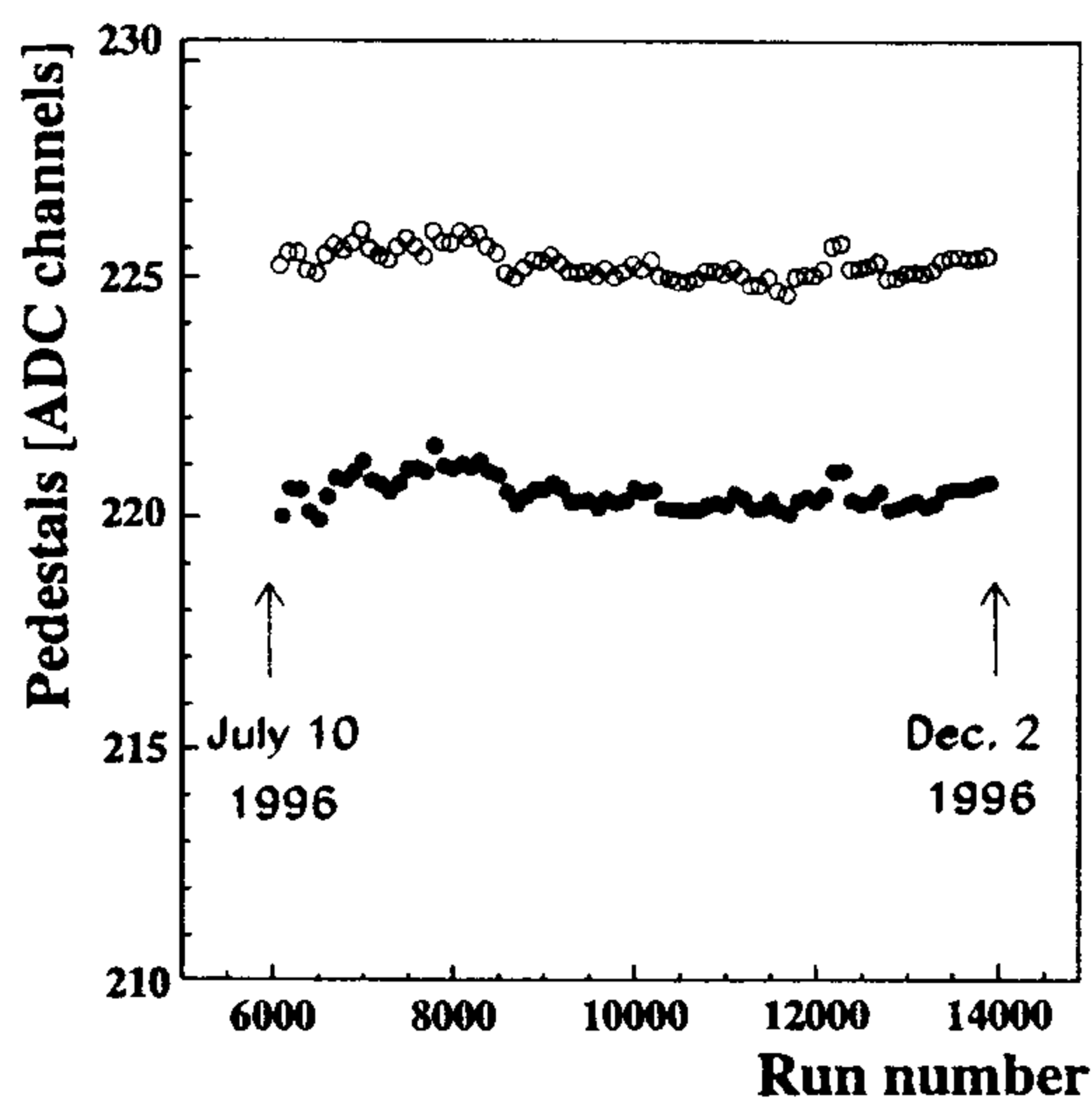
Fig. 7. Pedestal behavior for two typical counters during the 1996 running period.
