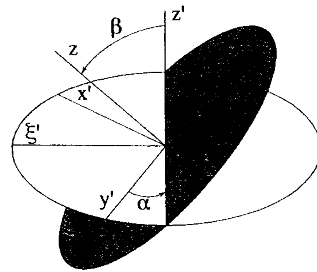
FIG. 1. The y-convention of the Euler angles.
