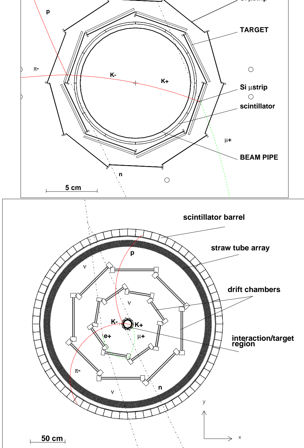
Figure 4: Sketch of the FINUDA detector front (beam) view. The interaction-target region (top); the outer tracker and scintillator barrel (bottom). An hypernuclear event is superimposed. A \phi decays to K^+K^- . The K^+ decays to \mu^+\nu_\mu , followed by \mu^+ \rightarrow e^+\nu_e\bar{\nu}_\mu . The K^- crosses the inner trigger scintillator, is tracked by the inner Si- \mu strip detector, stops in the target and forms an hypernucleus (eq.6). The momentum of the emitted prompt \pi^- , proportional to the energy of the hypernuclear level formed, is measured by the spectrometer. The hypernuclear \Lambda undergoes the process \Lambda p \rightarrow n p .
