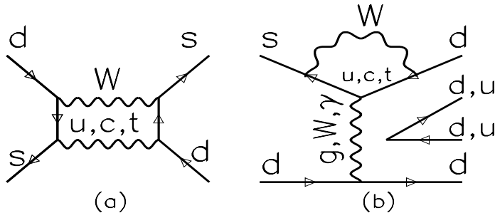
Figure 1: a) K^0 - \bar{K}^0 mixing b) Direct CP violation through penguin diagrams.
