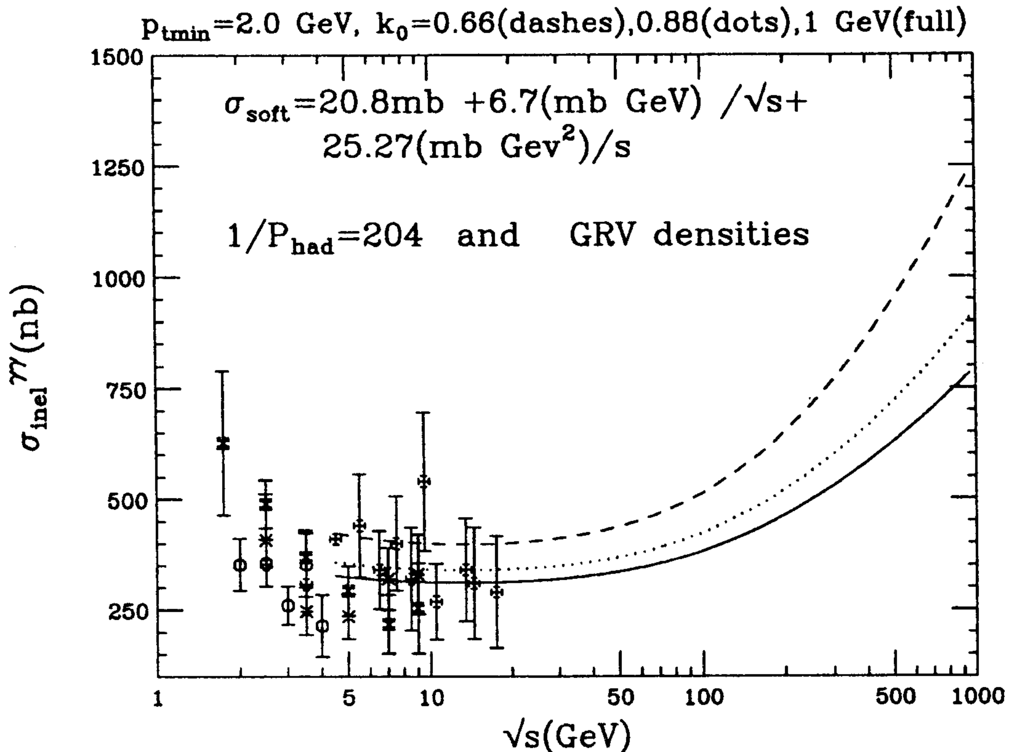
Figure 1: Total inelastic photon-photon cross-section for p_{tmin} = 2. GeV and different parton b-distribution in the photon. The solid line corresponds to k_0 = 1. GeV.
