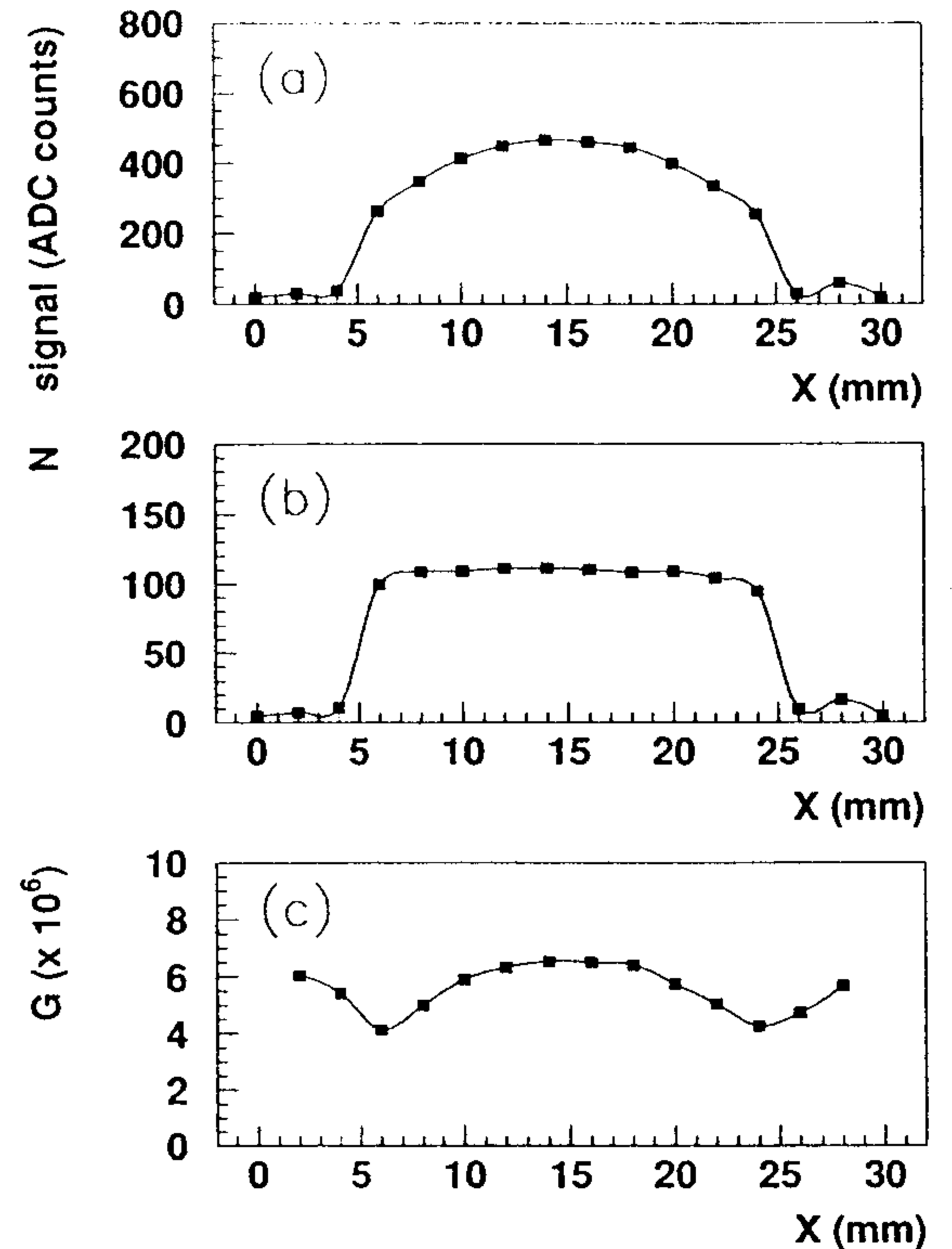
Fig. 9. Response of a 1 \frac{1}{8} in. H5756 tube in the same experimental conditions as in Fig. 7.
