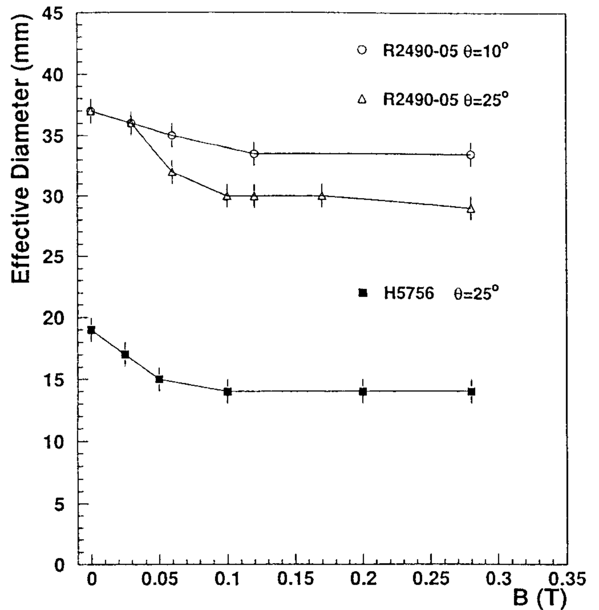
Fig. 13. Effective photocathode diameter (FWHM) for a 2 in. R2490-05 tube and a 1\frac{1}{8} in. H5756 tube, as a function of the magnetic field B . The angles are \theta = 25^\circ and \theta = 10^\circ .
