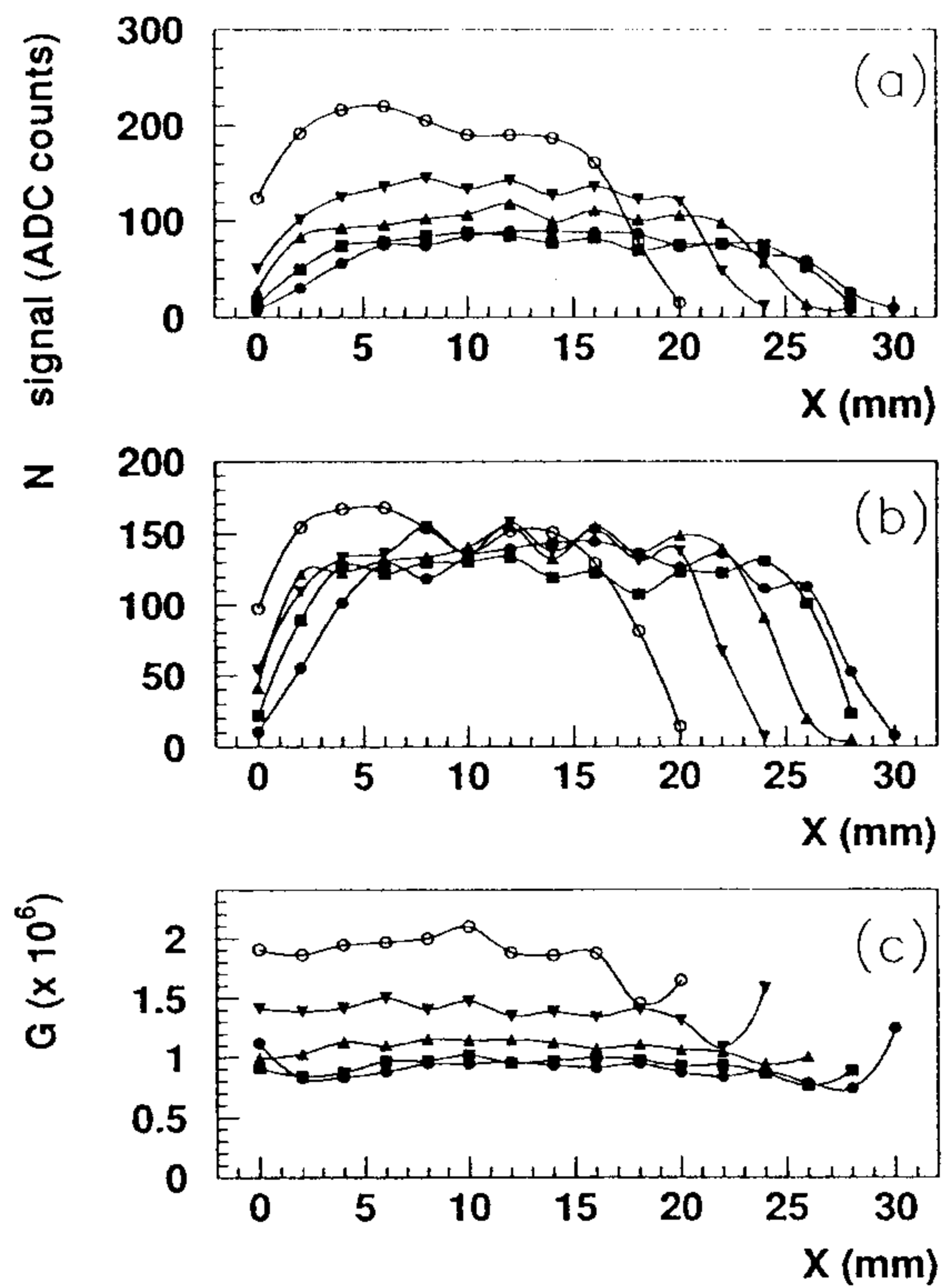
Fig. 11. Response of a 1.5 in. R2021 tube as a function of the light spot position along a diameter at B = 0.1 T and \theta = 0^\circ, 9^\circ, 18^\circ, 27^\circ, 36^\circ (full circles, squares, upwards triangles, downwards triangles, open circles, respectively). Plots (a), (b) and (c) as in Fig. 10.
