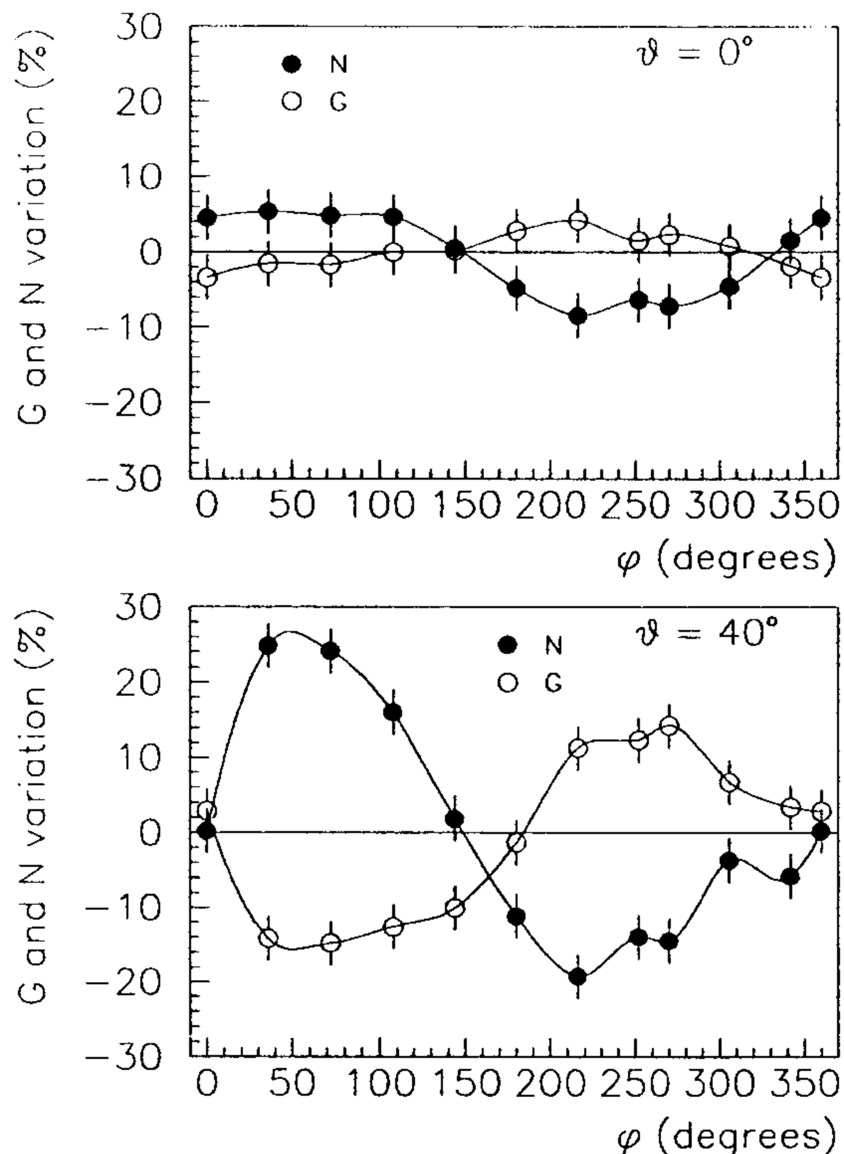
Fig. 6. Same plots as in Fig. 5 for a 1 in. R3423-01 tube.
