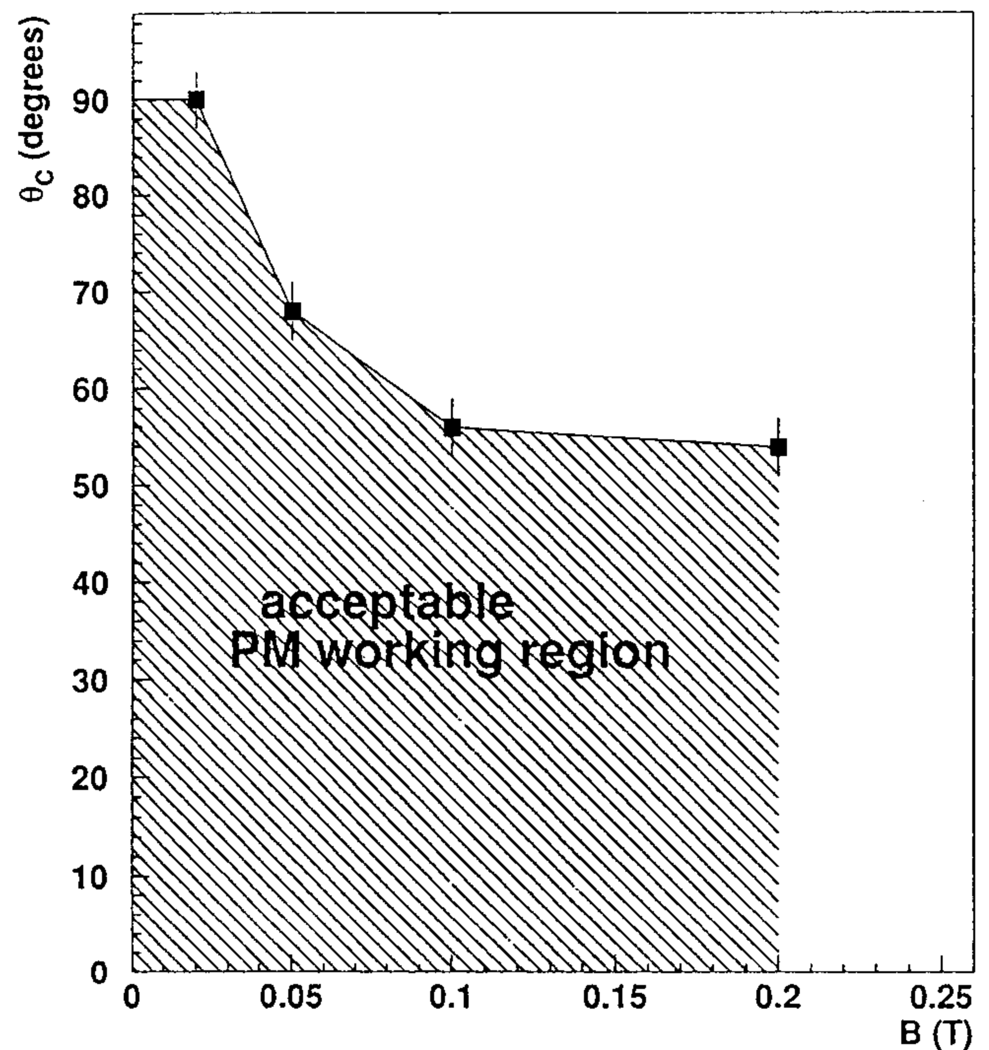
Fig. 3. Critical angle \theta_c as a function of the magnetic field. \theta_c is the angle between tube axis and magnetic field beyond which the photoelectrons collected by the multiplier starts to decrease sharply, as shown in Fig. 2c. the line is drawn to guide the eye.
