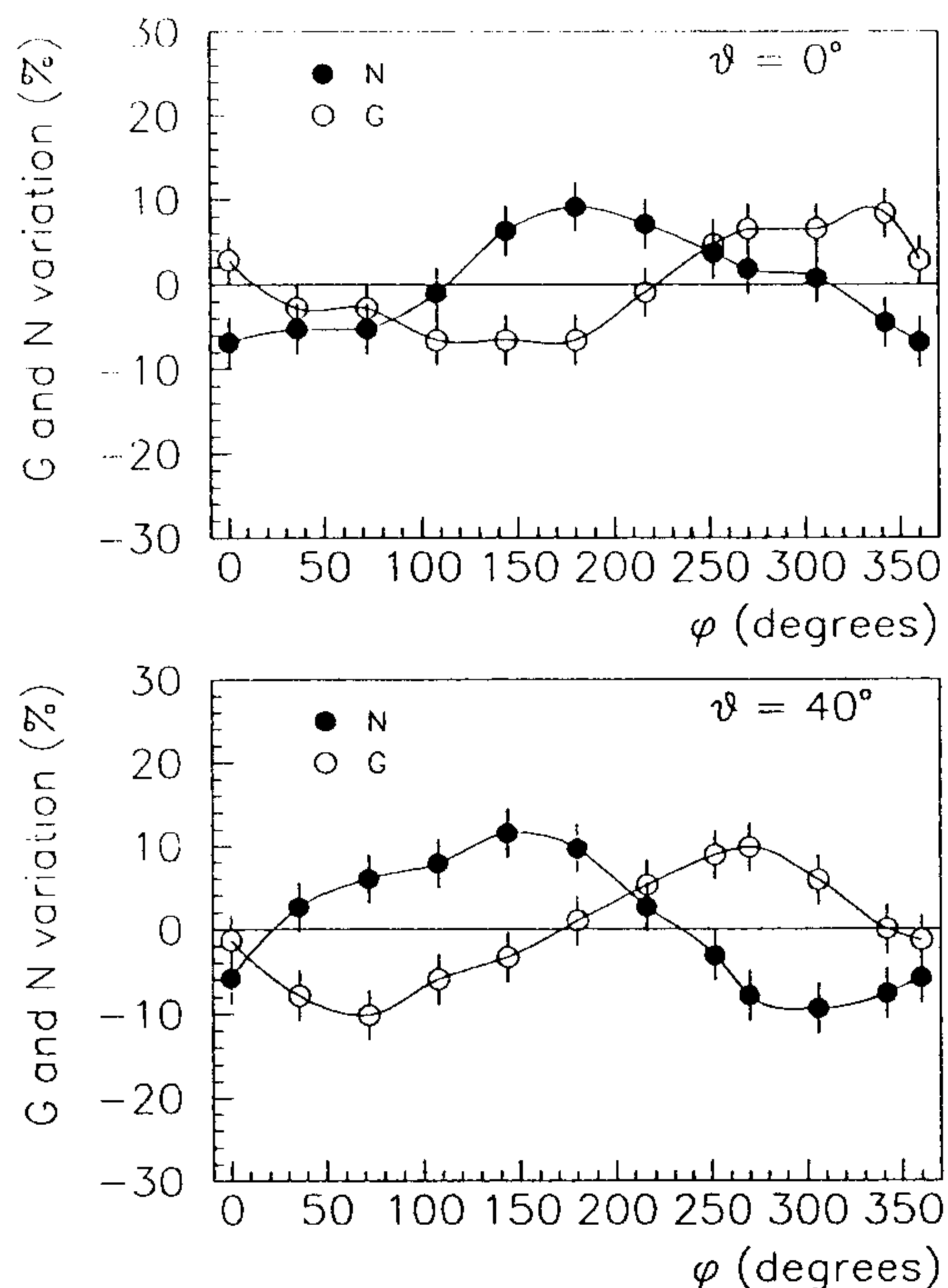
Fig. 5. Relative variation of the PM gain G with respect to the mean G value, and of the average number of photoelectrons N with respect to the N mean value, as a function of angle \phi at B = 0.13 T, \theta = 0^\circ and \theta = 40^\circ , for a R2490-05 tube. The lines are drawn to guide the eye.
