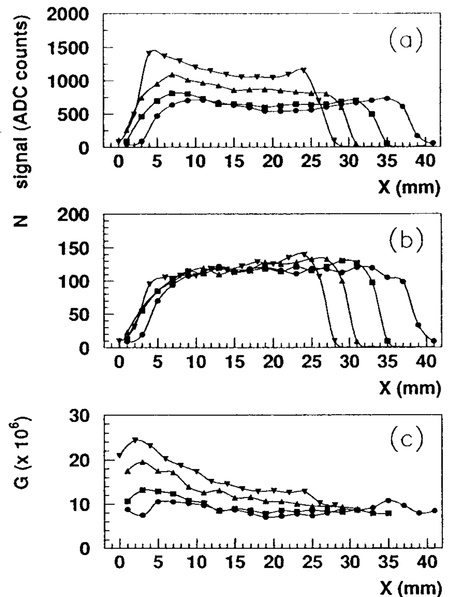
Fig. 10. Response of a 2 in. R2490-05 tube as a function of the light spot position along a diameter at B = 0.28 T and \theta = 0^\circ, 20^\circ, 25^\circ, 35^\circ (circles, squares, upwards and downwards triangles, respectively). (a) Signal spectrum mean value; (b) average number of photoelectrons N ; (c) PM gain G .
