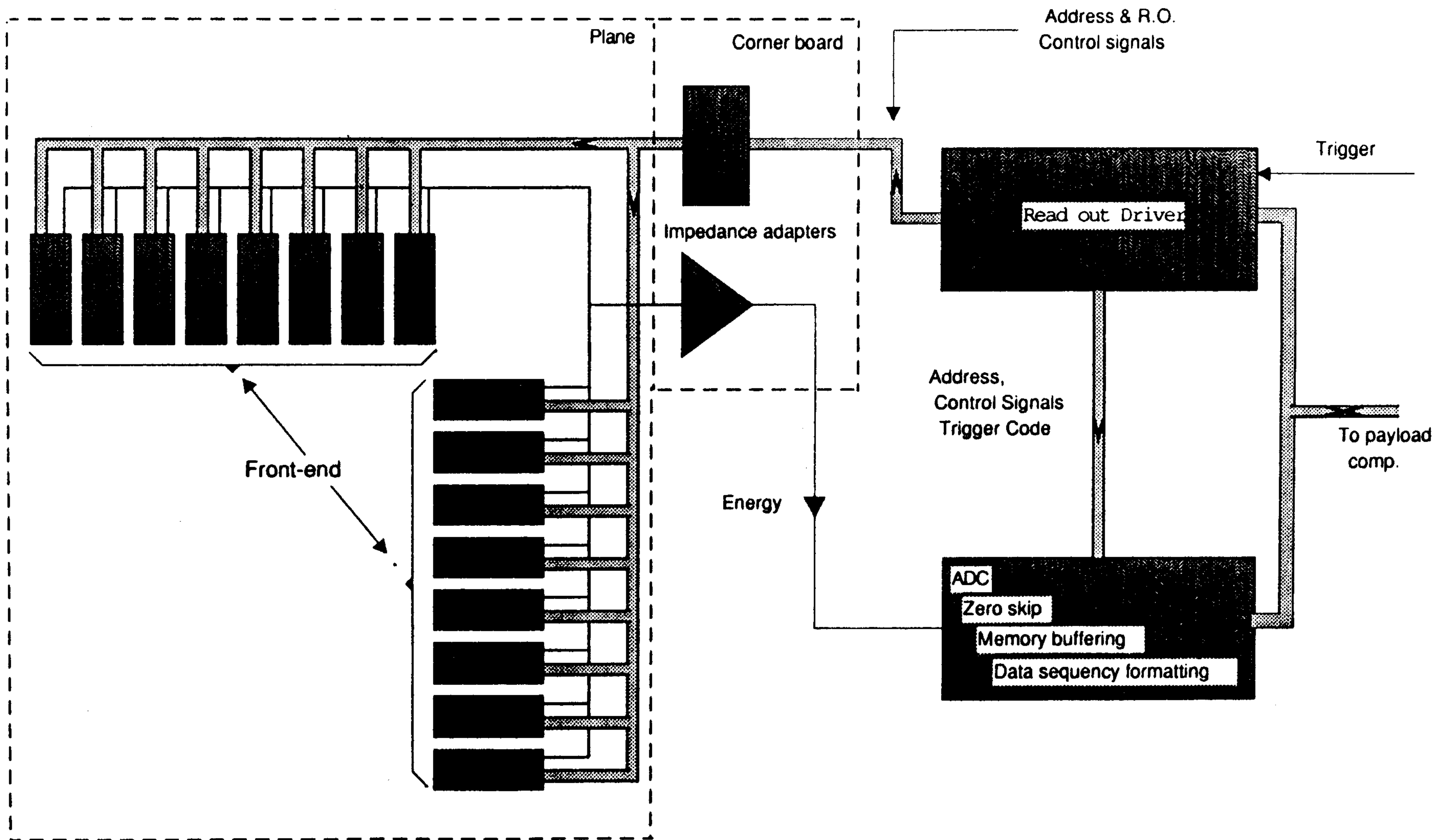
Figure 5 – The organization of the data acquisition system (right side) and the read-out logic for one plane (left side).
