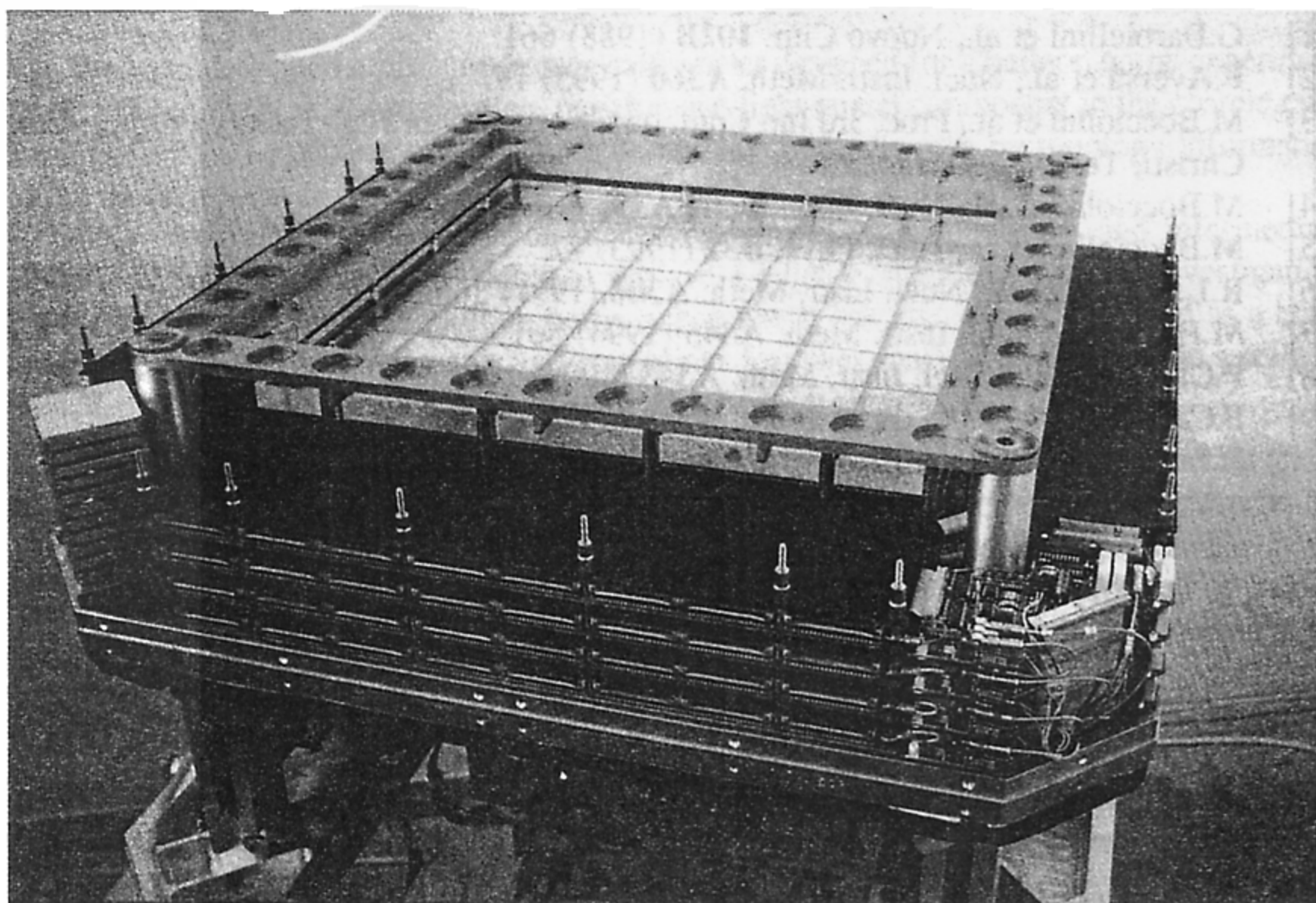
Figure 2 - The calorimeter assembled on its mechanical structure.
