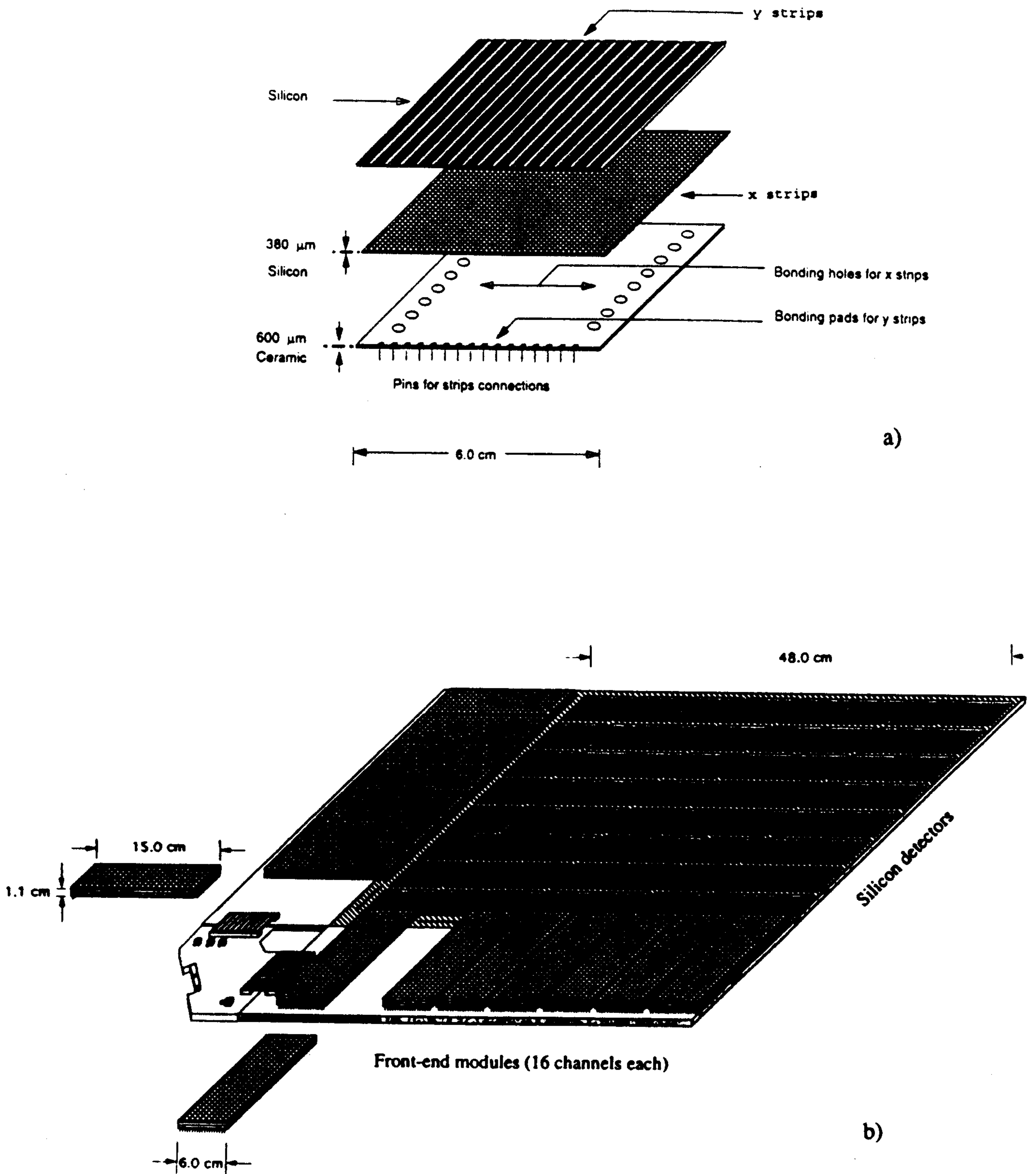
Figure 3 – a) Exploded view of one a single silicon module (x and y coordinates) on its ceramic support; b) the silicon plane arrangement. The 16-channel preamplifier modules are also shown.
