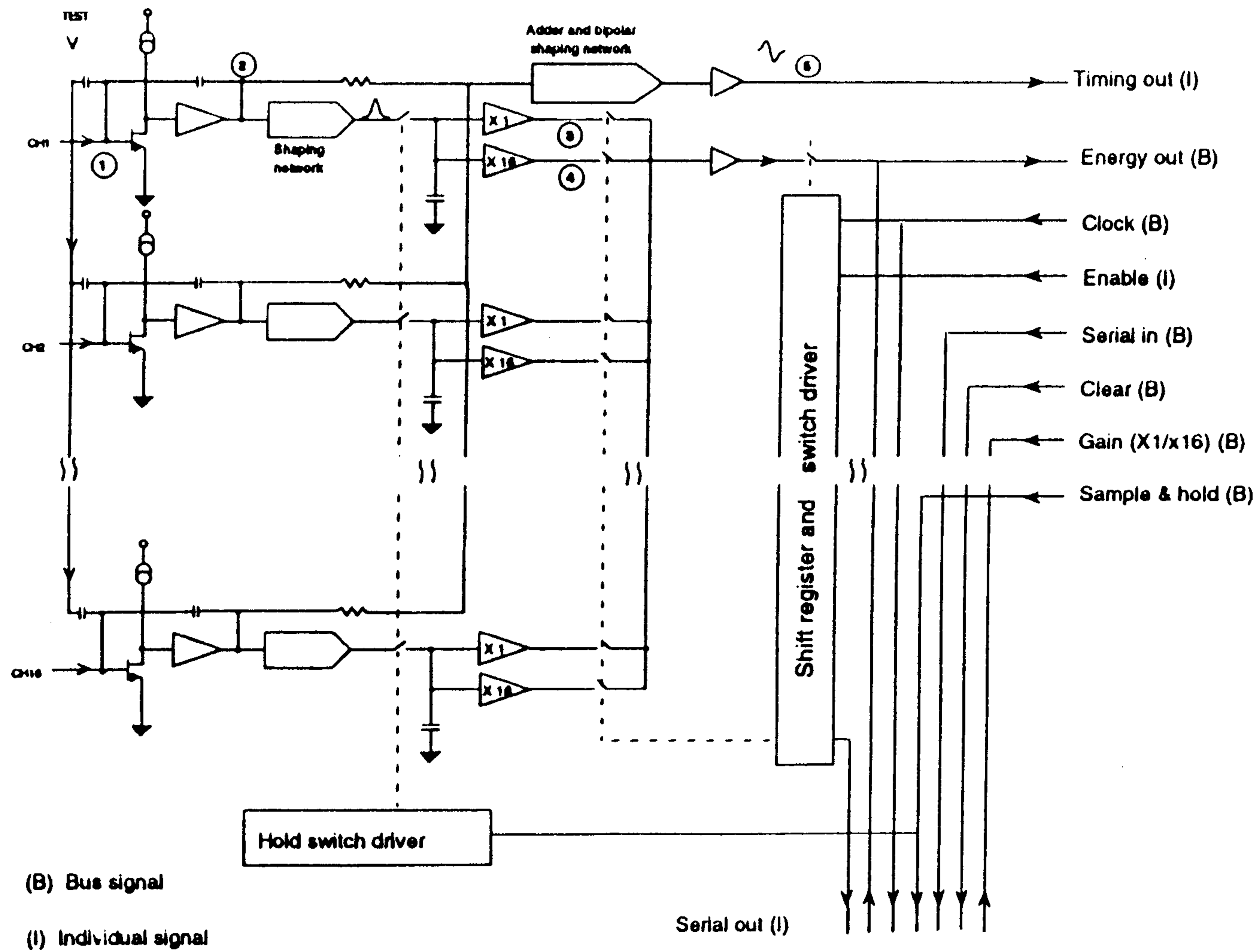
Figure 6 - Front-end schematic diagram for a single 16-channel preamplifier module. The time correlation of some of the analog signals is also shown.
