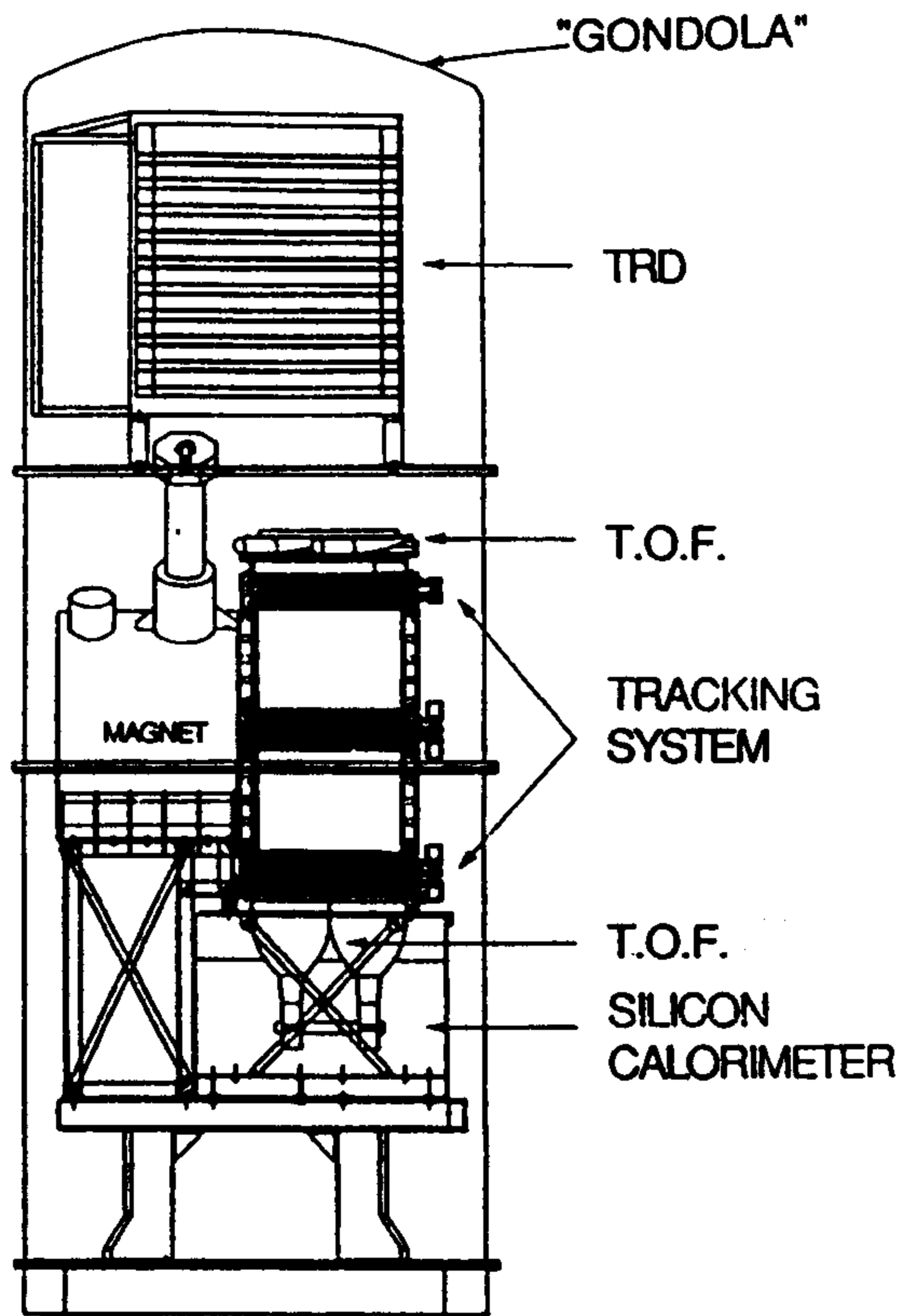
Fig. 1 – The New Mexico State University balloon-borne magnet facility equipped with Wizard TS93 apparatus used for the 1993 flight to identify cosmic ray electrons and positrons in the energy range from 5 to 50 GeV.
