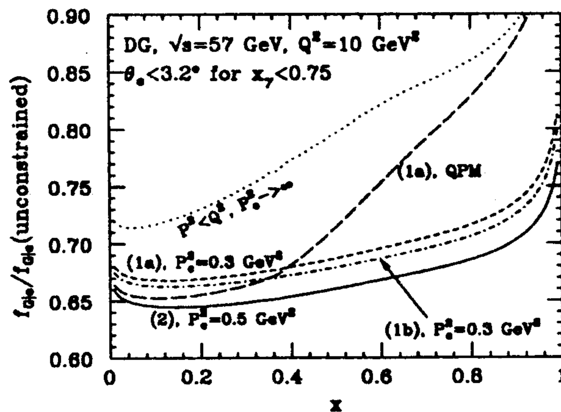
Figure 2: Reduction of the gluon density in the electron for an anti-tag situation, \theta < 3.2^\circ if z < 0.75 , due to the bound P^2 < Q^2 as well as from the suppression due to virtuality of the photon according to the different ansätze of Eqs. (14), (16), (17) and the QPM ansatz, at TRISTAN energies for Q^2 = 10 \text{ GeV}^2 .
