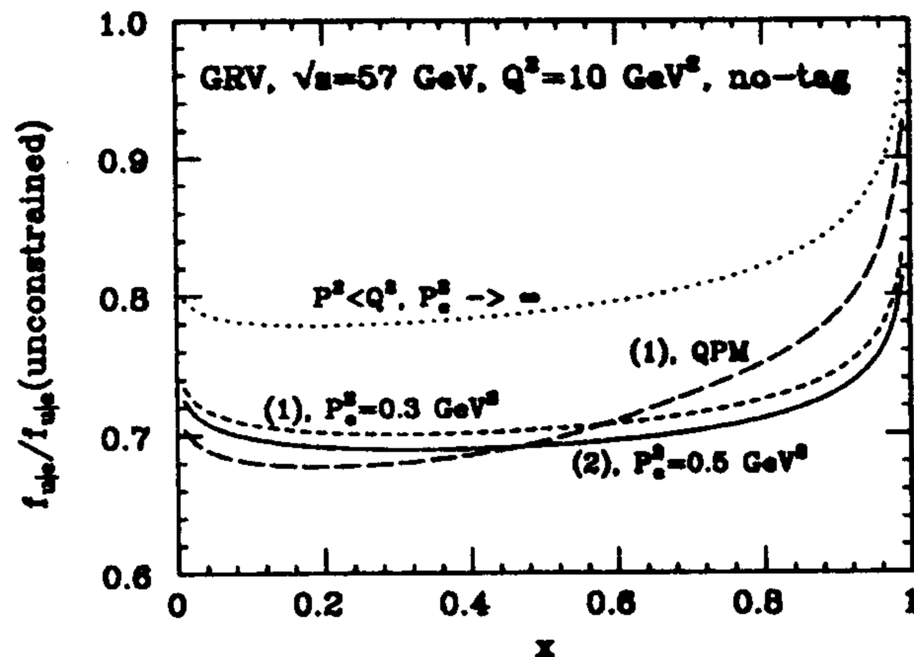
Figure 1: Reduction of the quark density in the electron in a no-tag situation due to the bound P^2 < Q^2 as well as from the suppression due to virtuality of the photon according to the different ansätze of Eqs. (8) and (11) at TRISTAN energies.
