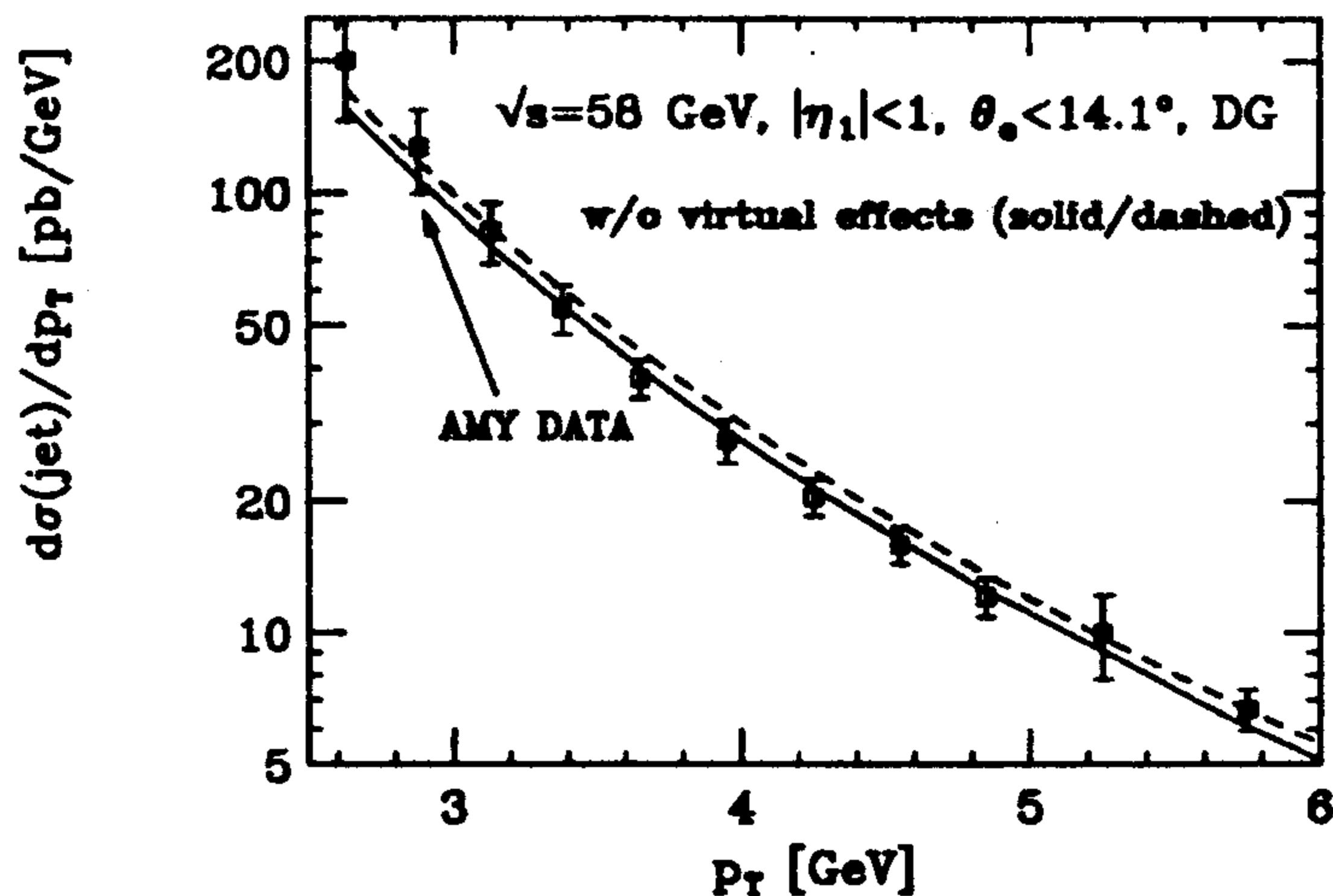
Figure 3: Effect on the jet cross-section in e^+e^- collisions for \sqrt{s} = 58 GeV, for the antitag-condition of the AMY collab. [1]: \theta < 14.1^\circ if z < 0.75 . The solid line includes suppression due to the virtuality of photons in addition to P^2 < Q^2 . The data are from the AMY collab. Ref. [1].
