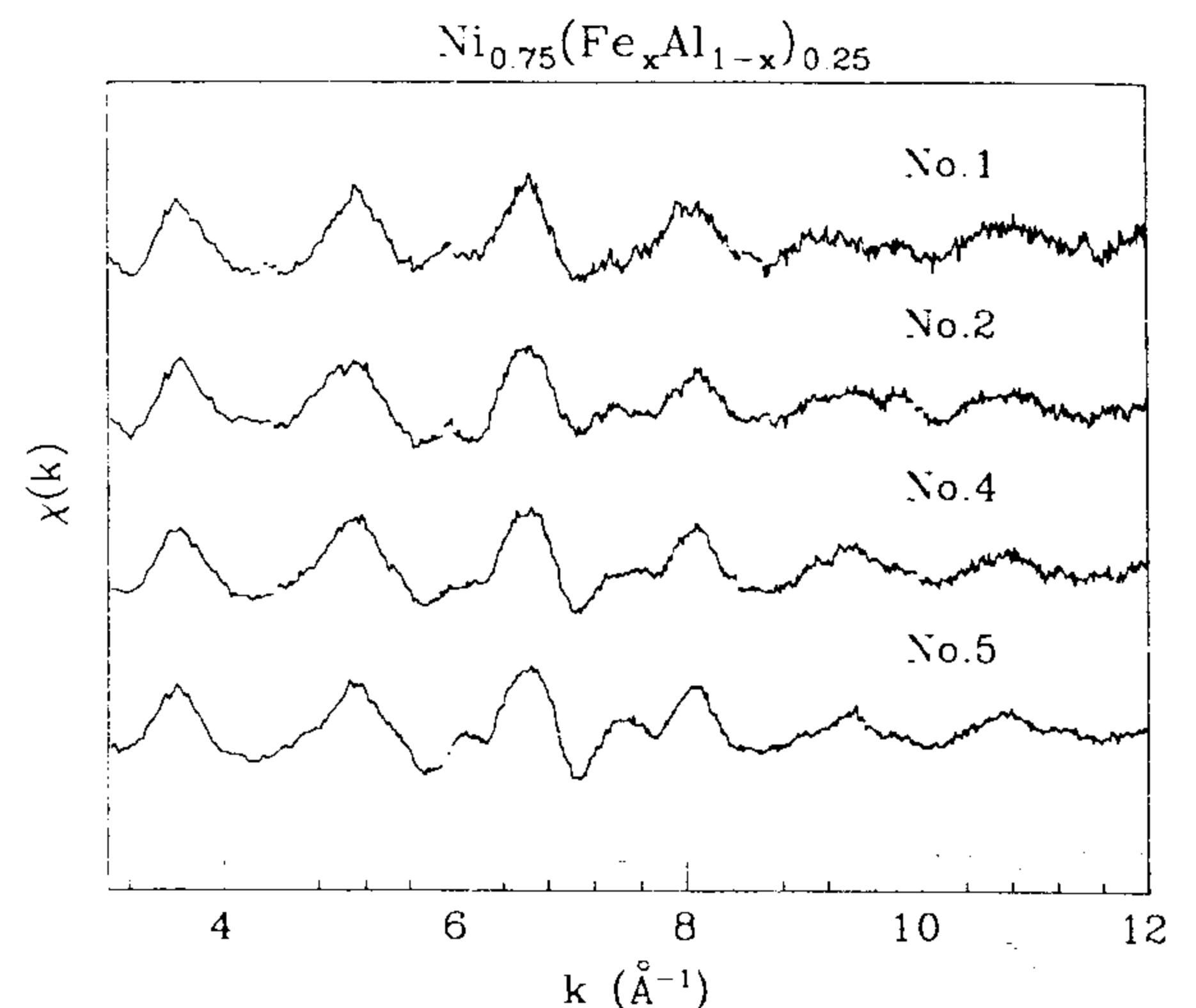
FIG. 1. Fe K -edge EXAFS measured in the fluorescence mode at T = 77 K. Data as been corrected for reabsorption.
