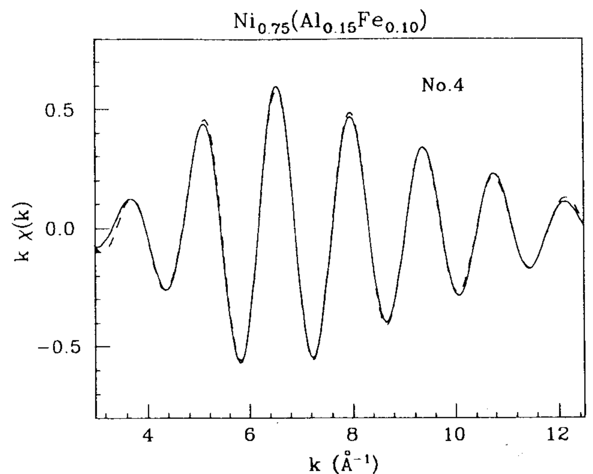
FIG. 4. Best fit to the filtered Ni K -edge EXAFS signal for sample No. 4. Average Ni- M ( M = \text{Ni, Fe} ) and Ni-Al contributions are included. We show the k\chi(k) signal as the solid line and the fit as the dashed line.
