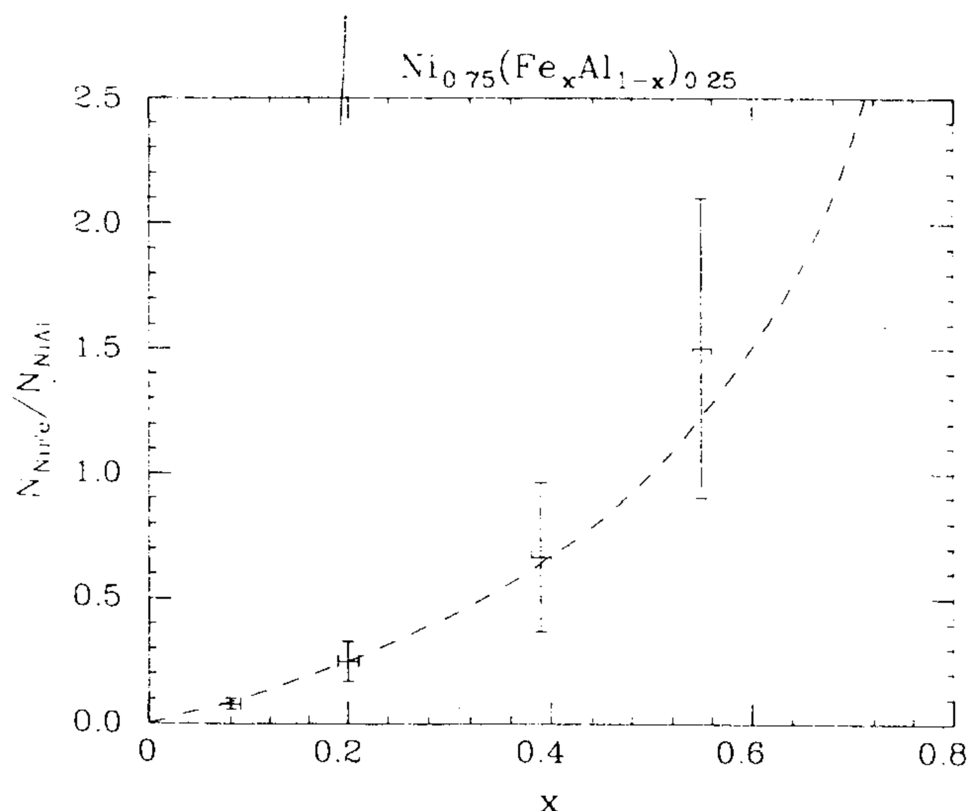
FIG. 5. The dashed curve indicates the ratio N_{\text{NiFe}}/N_{\text{NiAl}} in an L1_2 structure. Values of N_{\text{NiFe}}/N_{\text{NiAl}} obtained from Ni K -edge data are shown to follow the expected distribution for the L1_2 phase.
