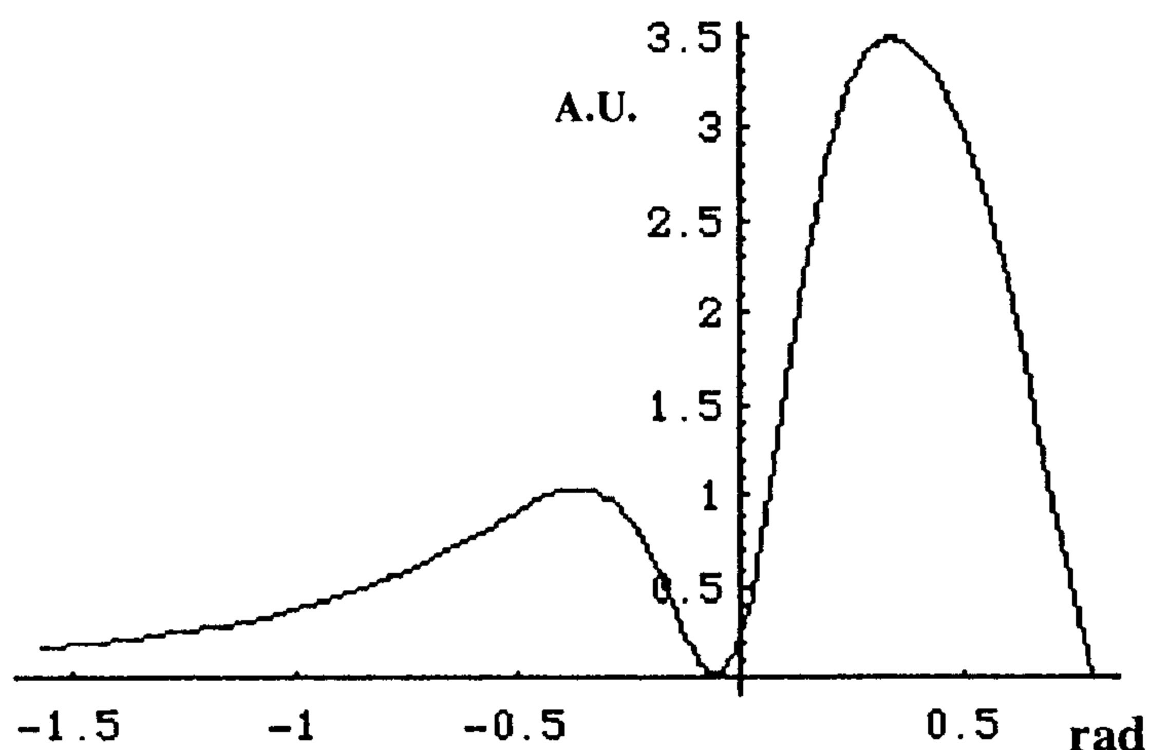
Fig. 2 - Intensity distribution on the horizontal plane of OTR from an Al mirror
