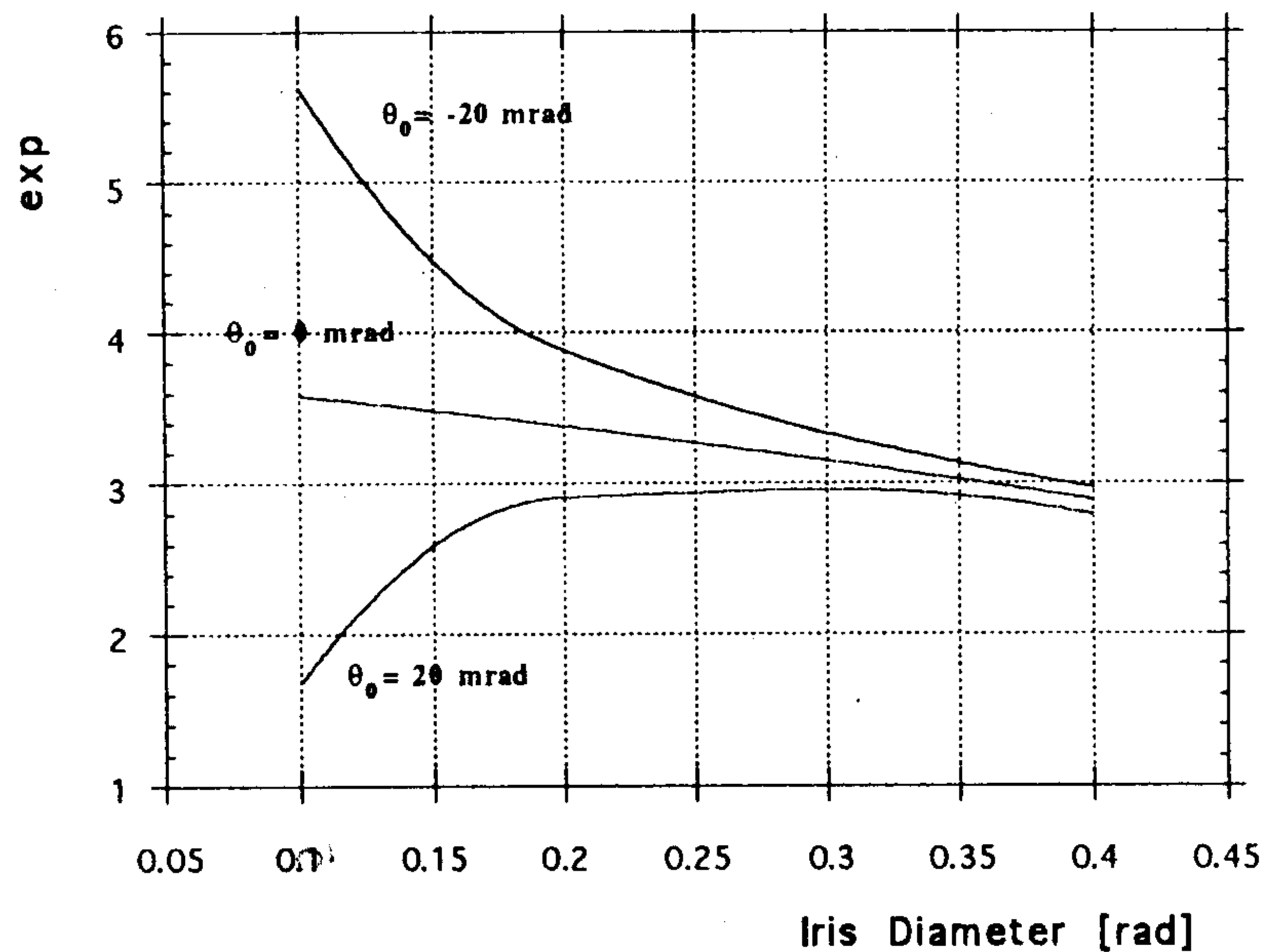
Fig. 6 - Behavior of the power law exponent as function of the iris diameter for three different radiation axis directions
