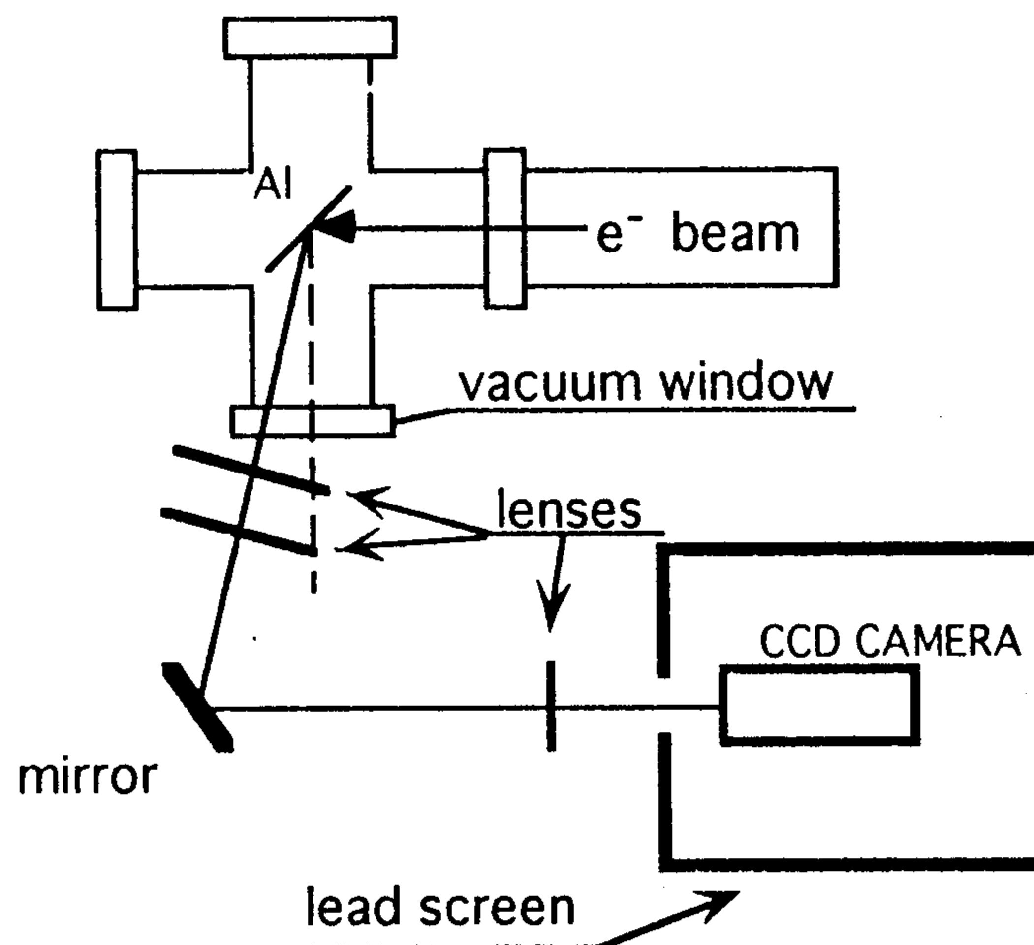
Fig. 7 - Schematic layout of the experimental set-up
