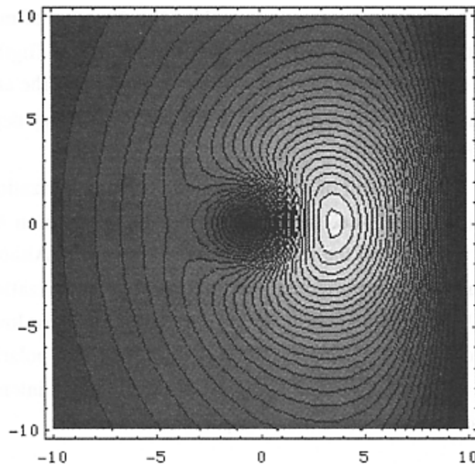
Fig. 1 - OTR radiation pattern backward emitted from an aluminum target by a 1 MeV electron
