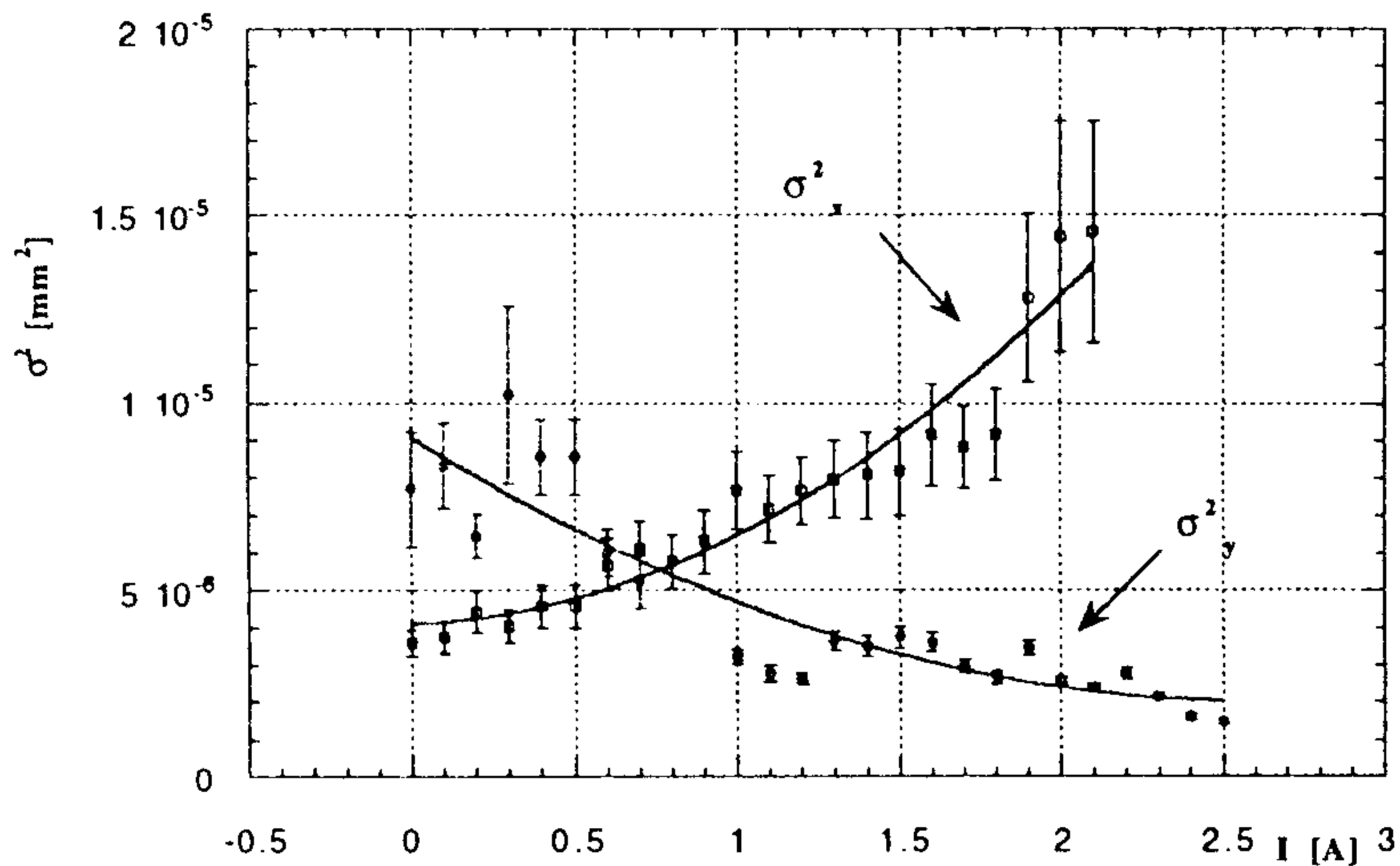
Fig. 11 - Square of the beam spot size vs quadrupole current in the horizontal and vertical planes
