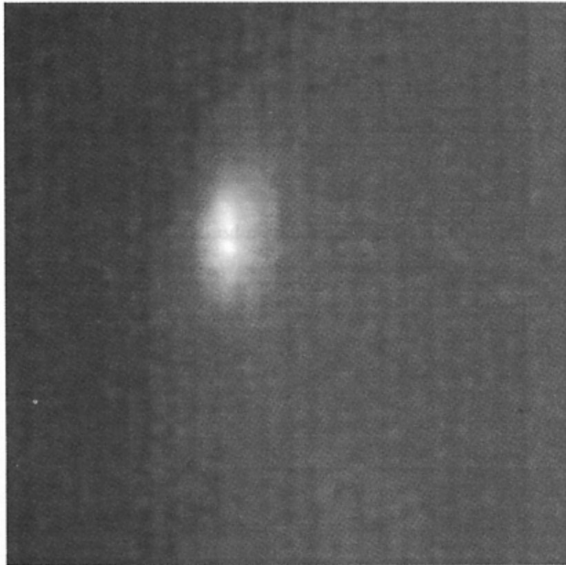
Fig. 8 - Image of the OTR beam spot with 1 mA mean current and 2 ms pulse length. The full-width dimension of the spot on the target is 4 mm in the vertical direction and 2.2 mm in the horizontal one
