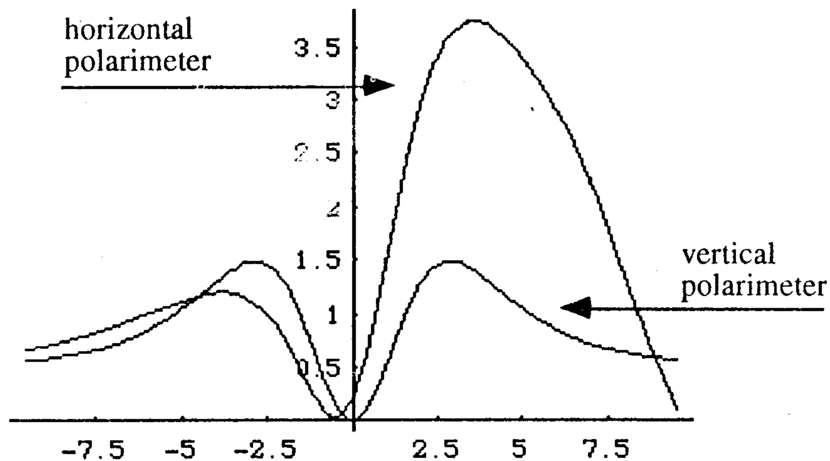
Fig. 5 - Intensity distributions along the horizontal and vertical axes corresponding to the maxima of the two polarization states
