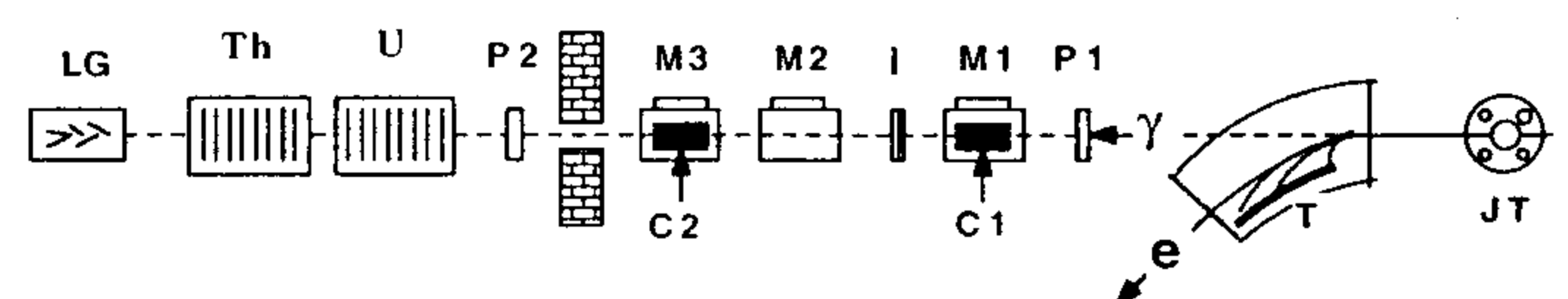
FIG. 2. Layout of the Jet Target tagged photon beam (not to scale): JT, Jet Target; T, tagging system; P1, P2 , movable photon beam profile chambers; M1, M2, M3 , sweeping magnets; C1, C2 , collimators; I , relative intensity beam monitor; U and Th , parallel-plate avalanche detectors loaded with uranium and thorium; LG , lead-glass photon spectrometer.
