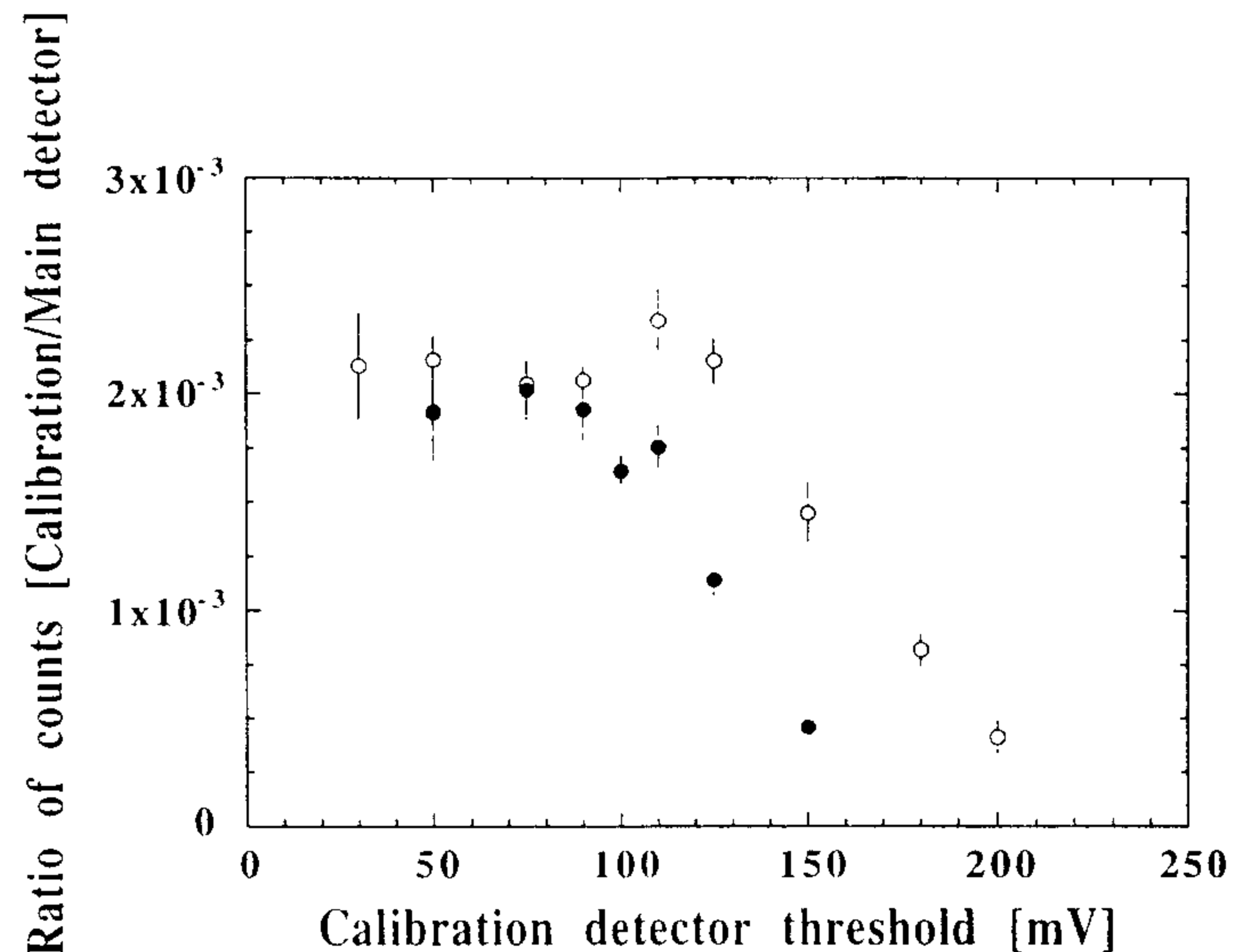
FIG. 3. Threshold curves of the ^{232}\text{Th} (closed circles) and ^{238}\text{U} (open circles) calibration detectors used to measure the effective thicknesses of the main ^{232}\text{Th} and ^{238}\text{U} target detectors.
