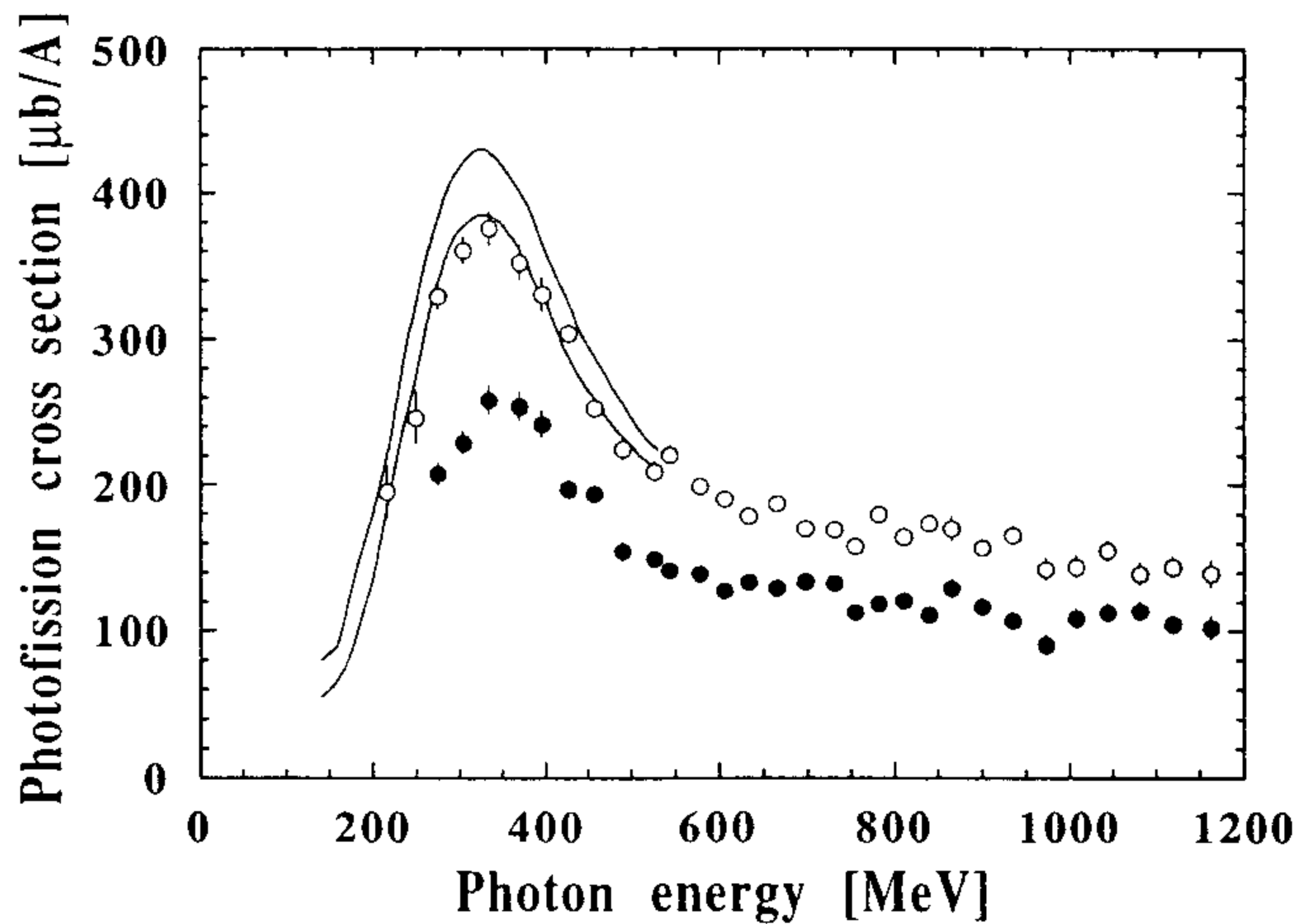
FIG. 4. The photofission cross section normalized to the mass number: present ^{232}\text{Th} data (closed circles) and ^{238}\text{U} data (open circles), Ref. [5]; the area between the two curves represents the universal behavior of the total nuclear cross section.
