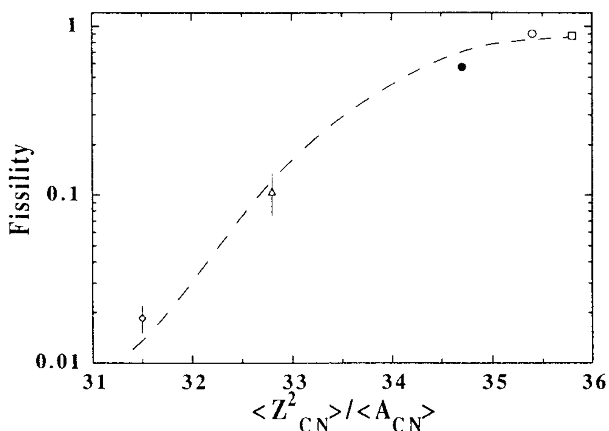
FIG. 6. Comparison of photofissility values for different nuclei measured with 300-MeV photons: ^{232}\text{Th} (closed circle), this work; ^{197}\text{Au} (diamond), Ref. [11]; ^{209}\text{Bi} (triangle), Ref. [12]; ^{238}\text{U} (open circle), Ref. [5]; ^{235}\text{U} (square), Ref. [7]. The dashed line is the result of an INC calculation.
