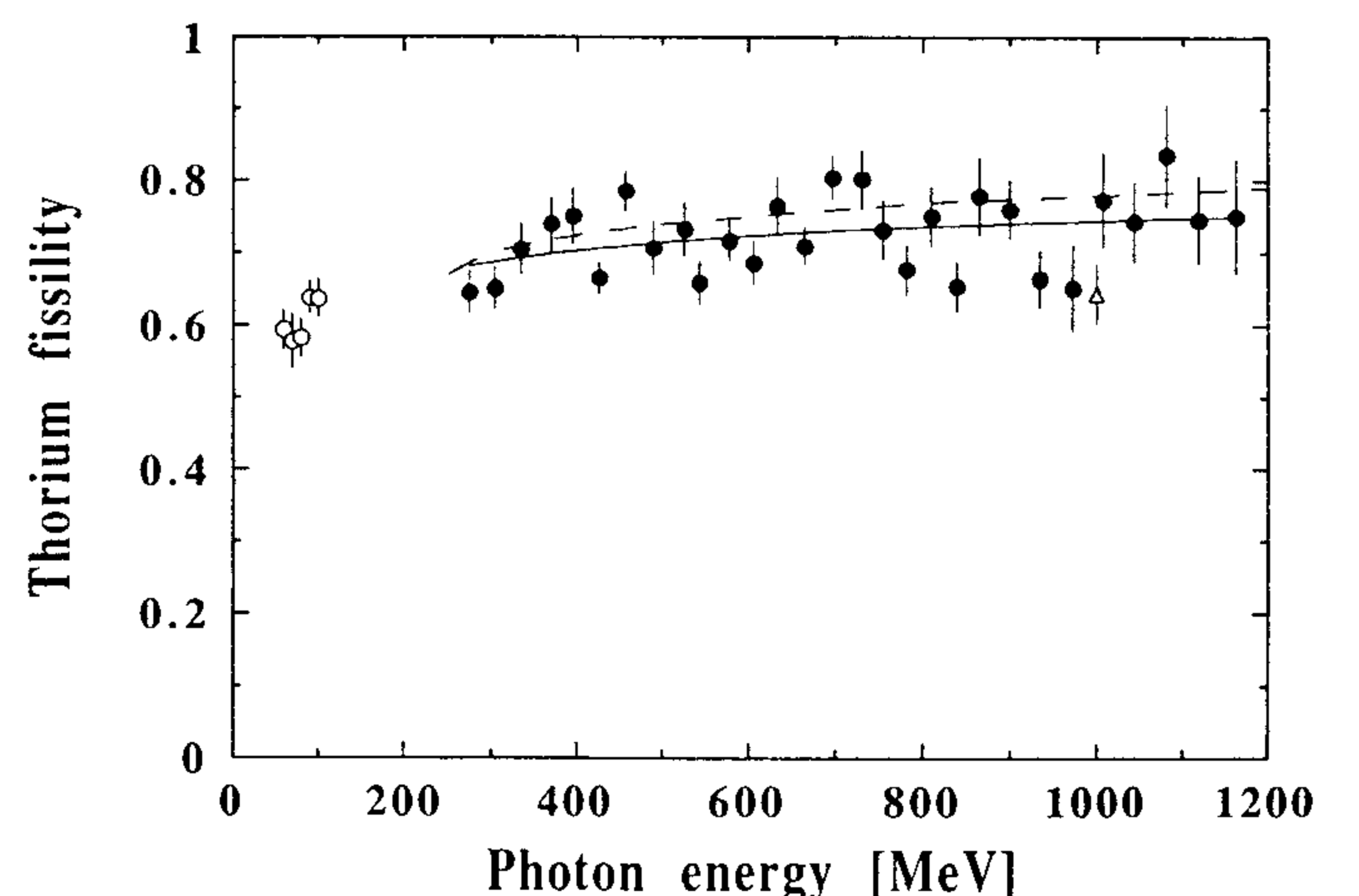
FIG. 5. Photofissility values for ^{232}\text{Th} obtained as described in the text (closed circles). Also shown are the values obtained with the same procedure from the data of Ref. [9] (open circles) and Ref. [25] (open triangle); the solid line is a fit of the form \ln W_f(k) = A - Bk^{-1/2} . The dashed line is the result of an INC calculation.
