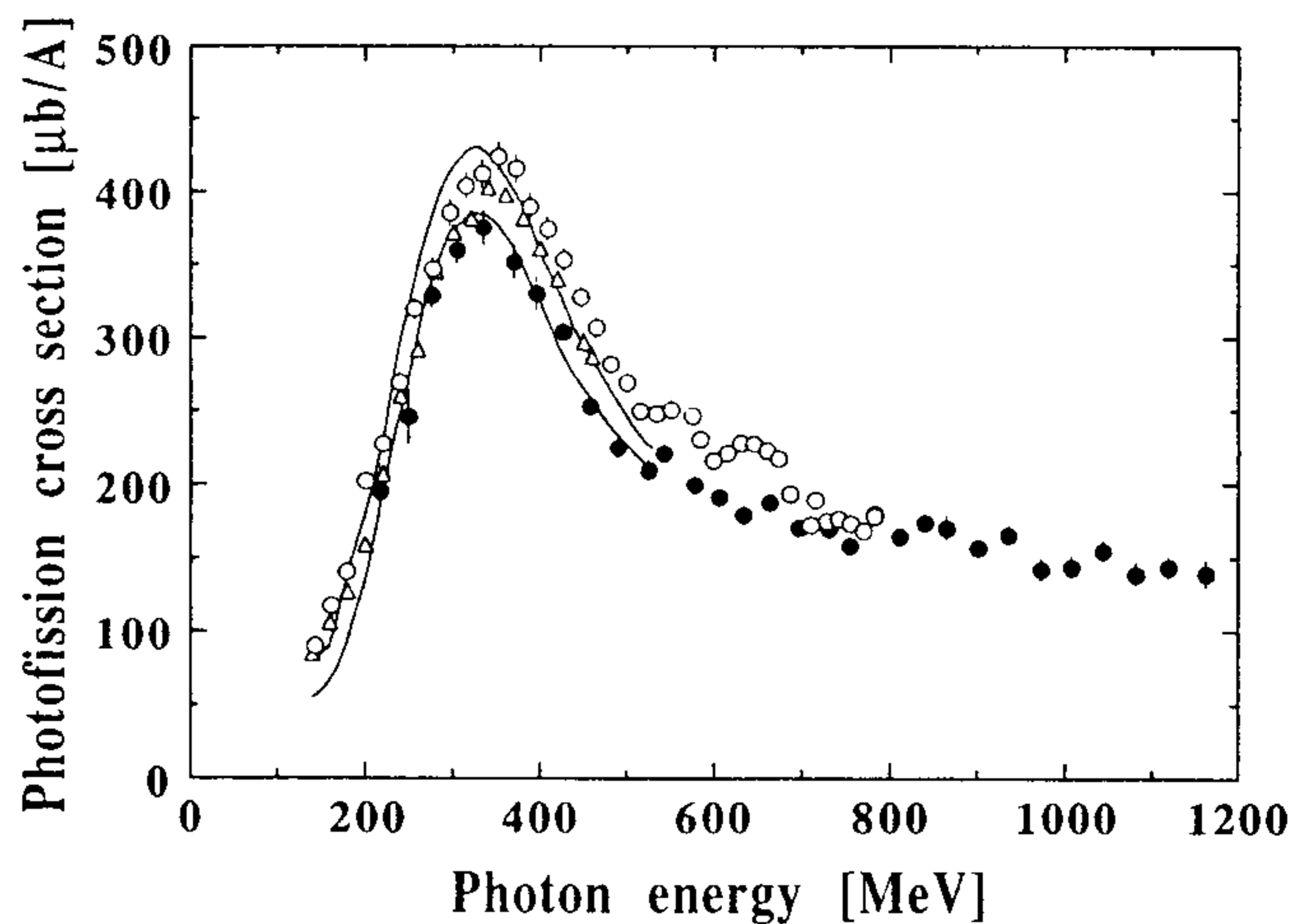
FIG. 1. ^{238}\text{U} photofission cross section data normalized to the mass number A , measured with tagged photons above the pion threshold: Ref. [5] (closed circles), Ref. [6] (open circles), Ref. [7] (open triangles). The area between the two curves represents the universal behavior of the total nuclear cross section (see the review in Ref. [8]).
