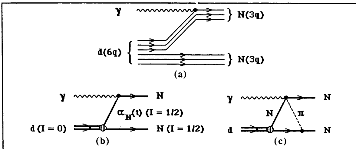
FIG. 1 – The 3-quark-exchange diagram which dominates the deuteron photodisintegration amplitude at sufficiently high energy and small t or u (a). In the Regge language this contribution corresponds to the exchange of the Reggeon \alpha_N(t) (b). At large energies the diagram of (b) includes the contribution of the graph (c), which describes the photoproduction on a nucleon.
