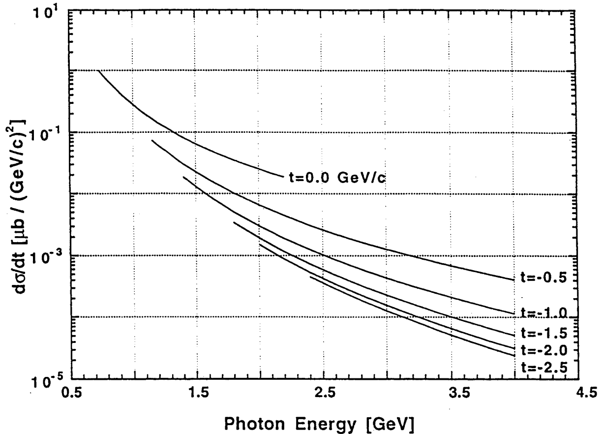
FIG. 3 – Differential cross section for deuteron photodisintegration at t=0, -0.5, -1, -1.5, -2, and -2.5 (GeV/c) 2 as a function of the photon energy.
