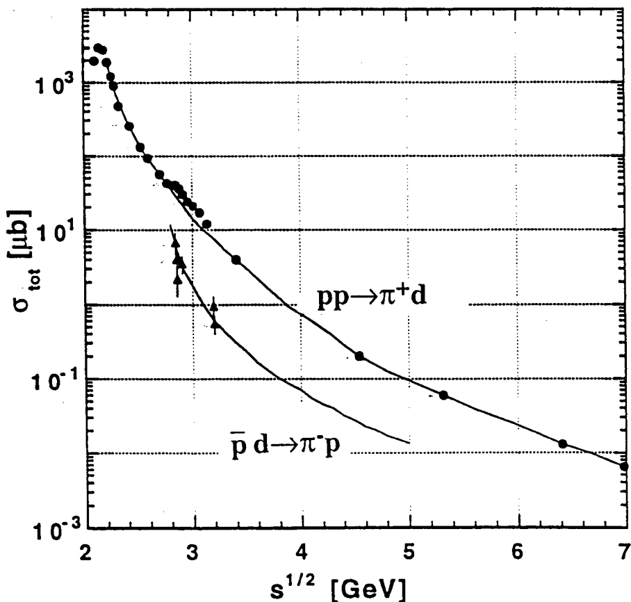
FIG. 2 – Total cross sections of the reactions pp \rightarrow \pi^+ d [16] and \bar{p}d \rightarrow \pi^- p [17,18] as a functions of c.m. energy, and the predictions of the QGS model. [14]
