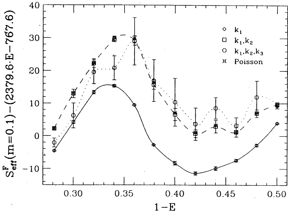
Figure 2: Same as Figure 1, but at m = 0.1
