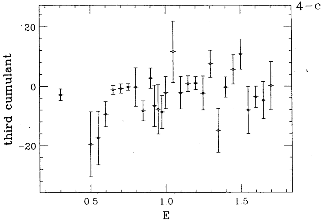
Figure 4: a) first, b) second and c) third cumulant of S_f^{eff} versus E at m = 0 for an 8^4 lattice.
