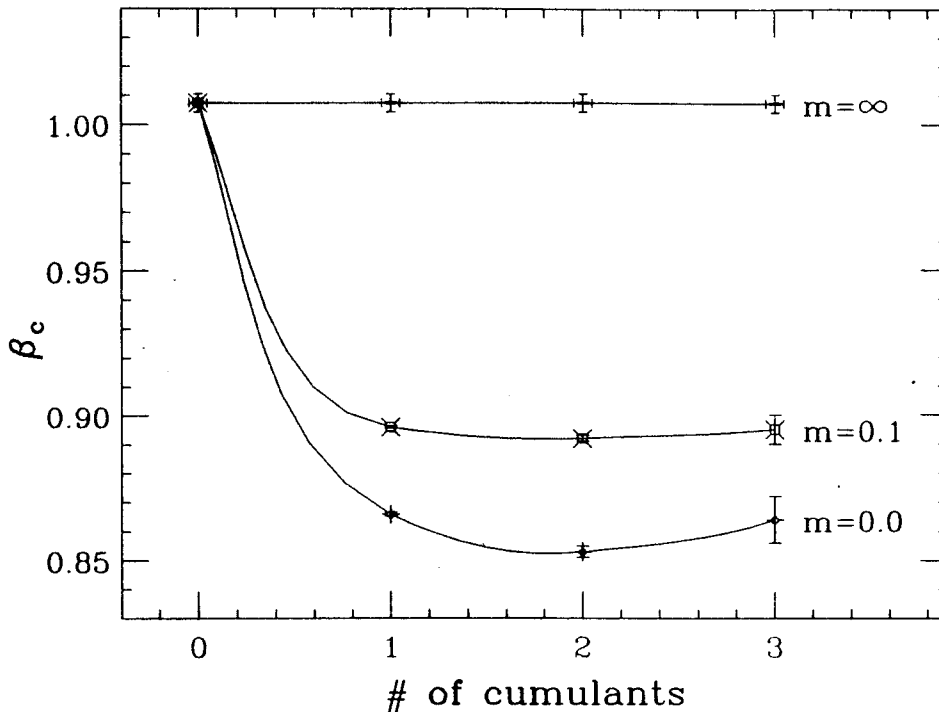
Figure 7: Measurement of \beta_c in an L = 8 lattice for compact U(1) with n_f = 4 . The x axis corresponds to the order of the approximation in the cumulant expansion. The values corresponding to the quenched ( m = \infty ), m = 0.1 and m = 0.0 cases are presented.
