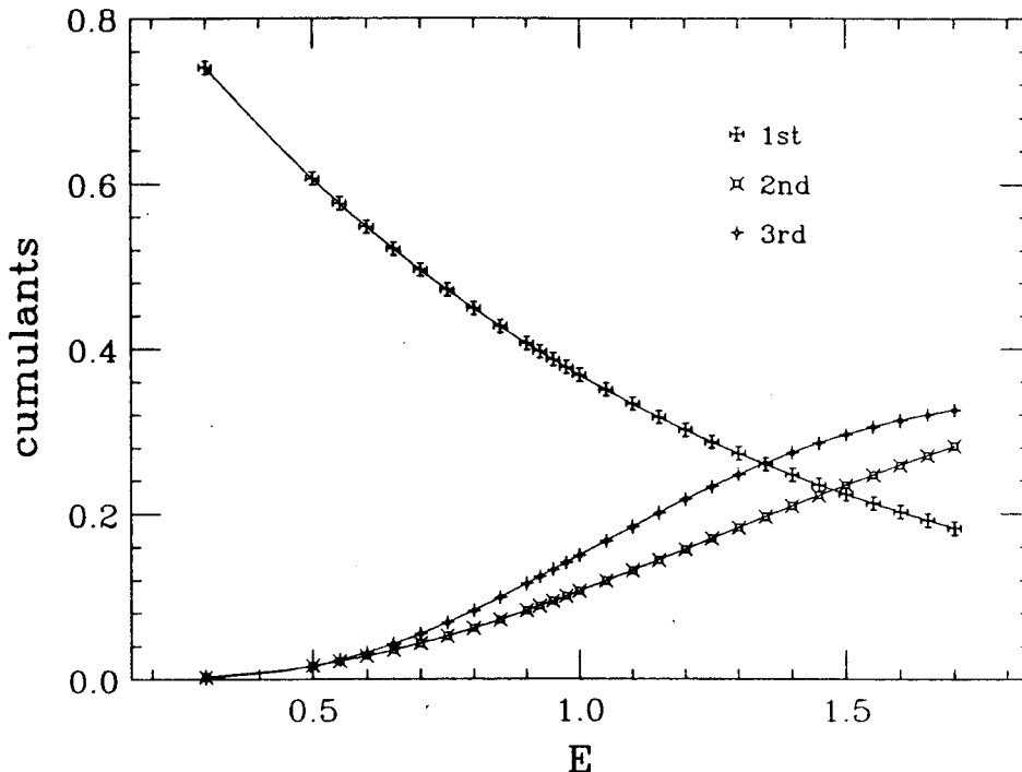
Figure 9: First cumulants of e^{-S_{eff}(E)} = \langle e^{-S_G(U_{x,\mu})} \rangle_E (eqn. 4.6).
