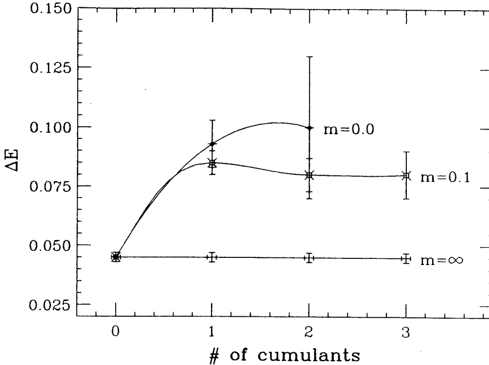
Figure 8: Latent Heat as a function of m .
