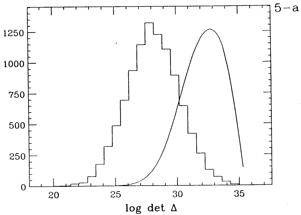
Figure 5: p.d.f. of the logarithm of the determinant, and its product with the exponential in (9) for V = 4^4 (a) and V = 12^4 (b).
