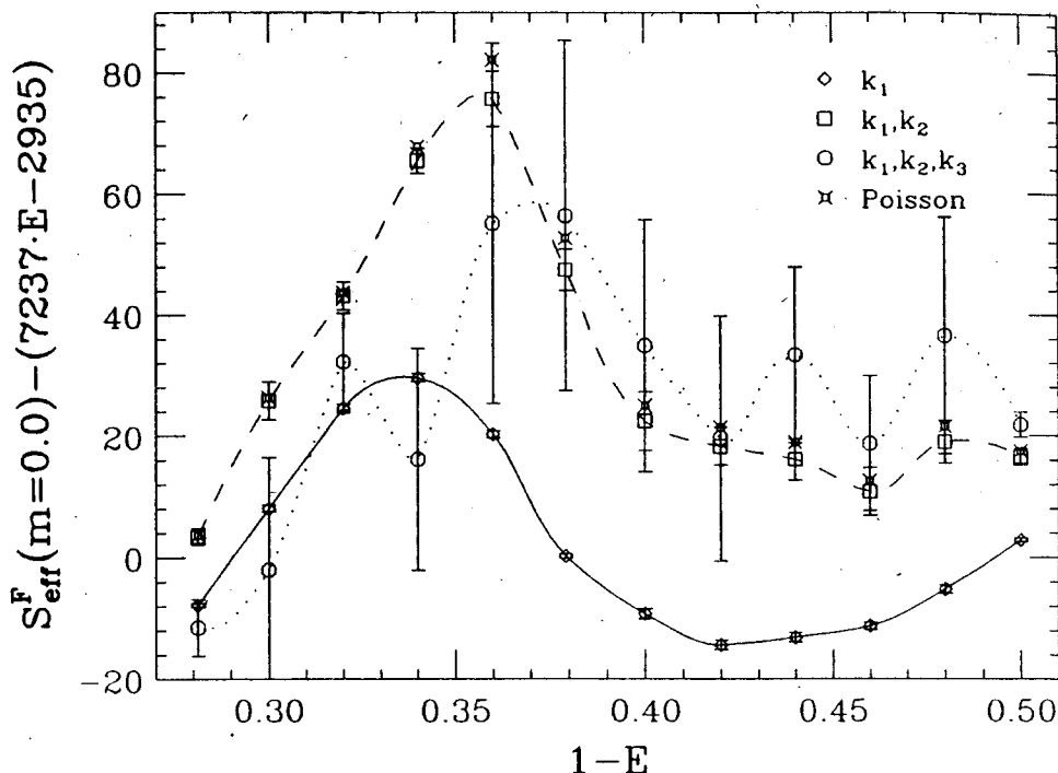
Figure 1: The logarithm of the average determinant in an L = 8 lattice, with n_f = 4 , m = 0 at the first ( k_1 ), second ( k_1, k_2 ), third order of the cumulant expansion, as well as for a Poisson distribution. In this last case error bars are not shown for clarity; they are very similar to the second order ones. The y axis is the action with a linear shift ( of the results of the first order ) to increase visibility.
