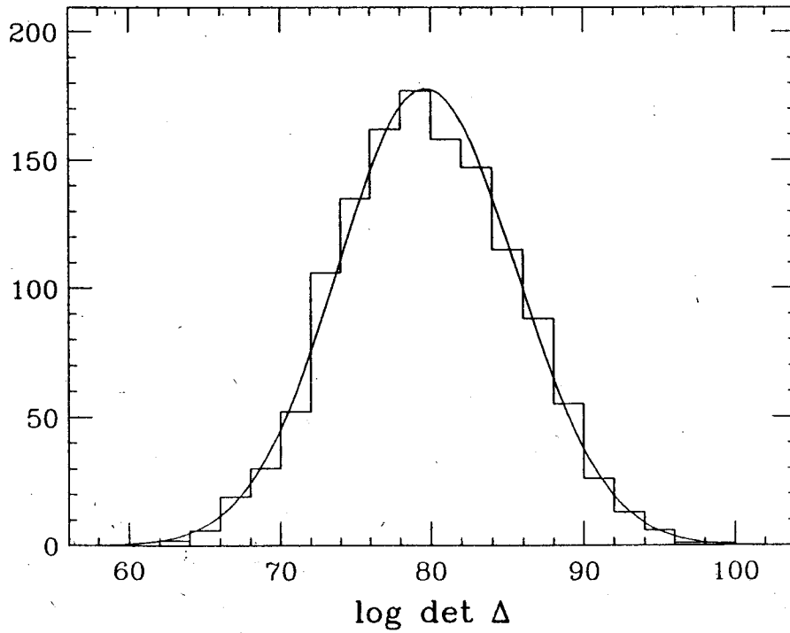
Figure 3: Probability distribution of \log \Delta(m, A_\mu) at m = 0.0 , E = 1.20 , N_f = 4 for an 8^4 lattice. The continuous line is a gaussian fit, with \chi^2/d.o.f. = 0.487 .
