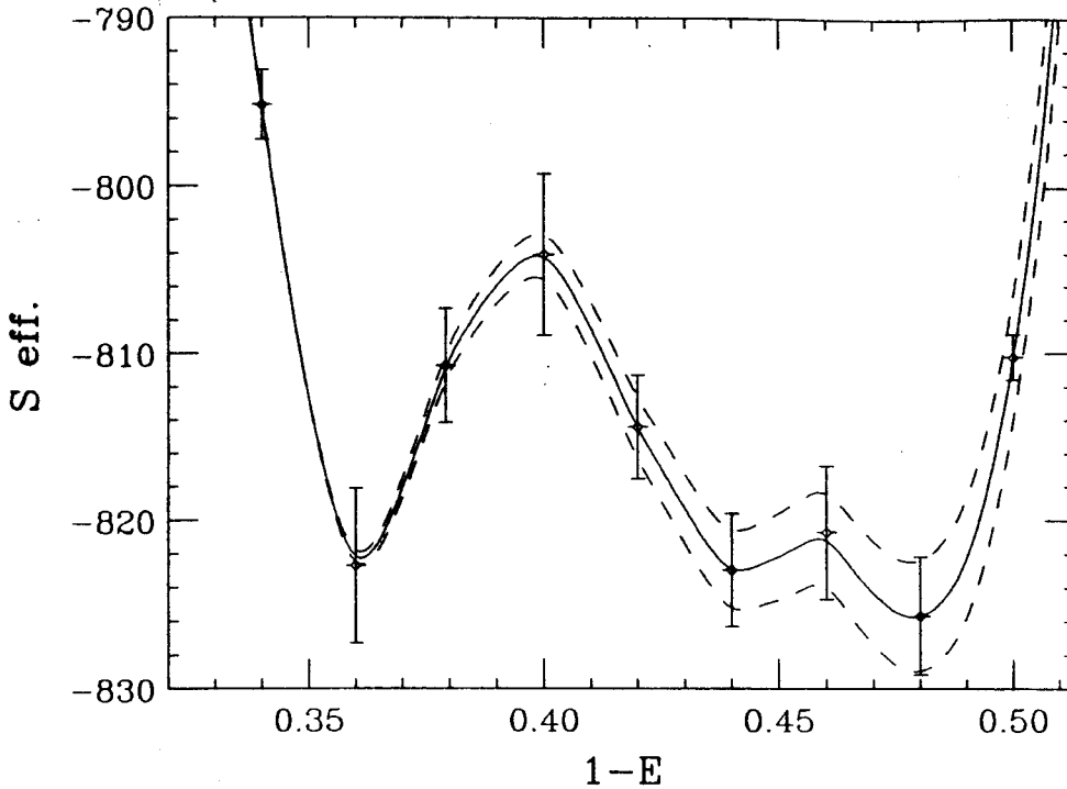
Figure 6: Effective potential S_{eff}(E, V, \beta, m) for L = 8 , n_f = 4 and m = 0 obtained by summing the pure gauge contribution computed by folding different Monte Carlo simulations, and the fermionic action in the gaussian approximation (cumulants expansion up to k_2 ). The continuous line corresponds to \beta = 0.853 (our determination of \beta_c ). Broken lines correspond respectively to \beta = 0.852 and \beta = 0.854 and are shown to allow an estimation of the error.
