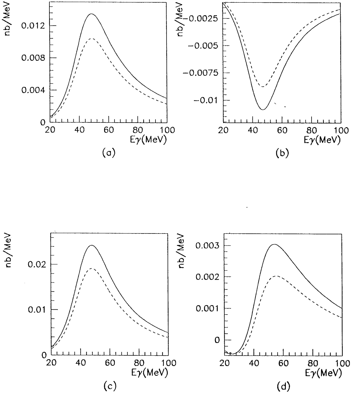
Figure 5. a. \gamma spectrum: f_0 \rightarrow \pi^+ \pi^- \gamma ; b. 2\Re(A_\rho \cdot A_{f_0}^*) ; c. |A_\rho|^2 - 2\Re(A_\rho \cdot A_{f_0}^*) ; d. |A_\rho|^2 + 2\Re(A_\rho \cdot A_{f_0}^*) . \text{BR}_{\phi f_0 \gamma} = 2.5 \times 10^{-4} . Solid lines are without angular cuts, dotted lines are for |\cos \theta_{\gamma, \text{beam}}| < 0.9 and |\cos \theta_{\pi \gamma}| < 0.9 .
