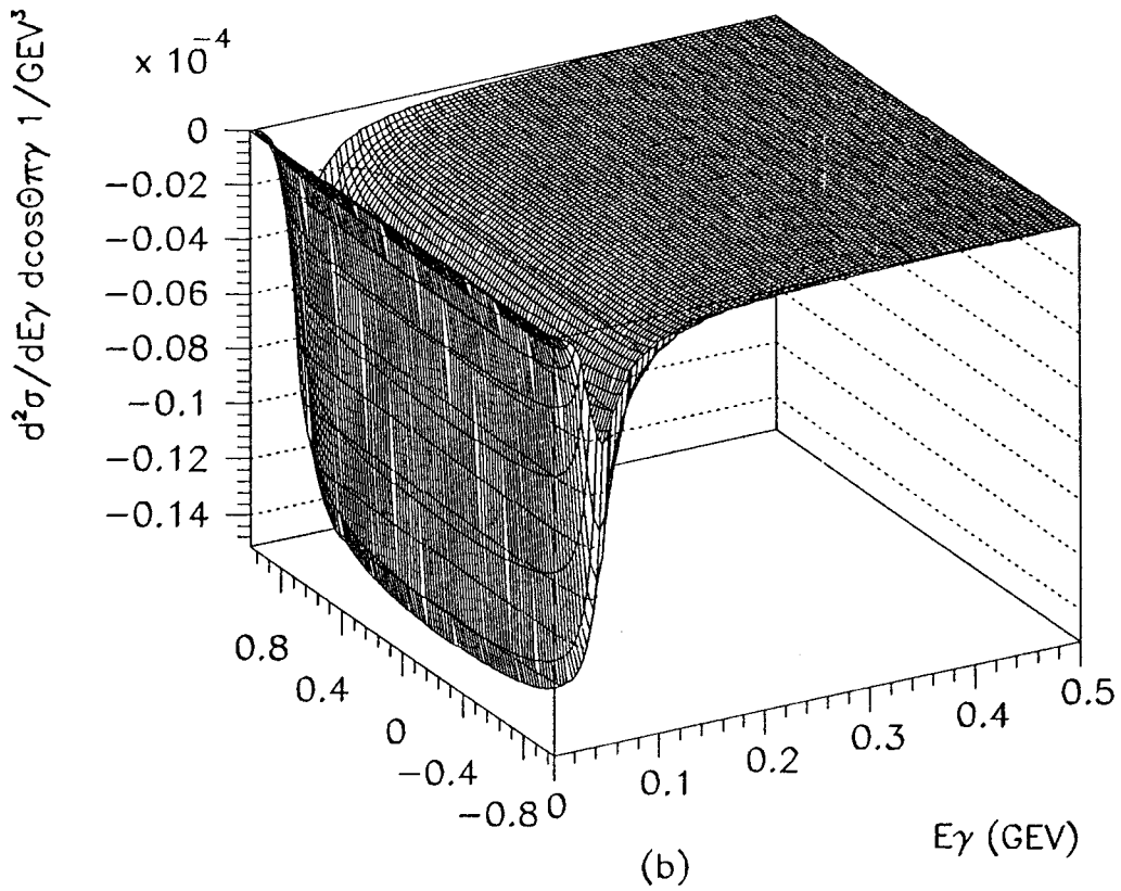
Figure 16. a. d^2\sigma/dE_\gamma d\cos\theta_{\gamma,\text{beam}} vs E_\gamma , \cos\theta_{\gamma,\text{beam}} ; b. d^2\sigma/dE_\gamma d\cos\theta_{\pi\gamma} vs E_\gamma , \cos\theta_{\pi\gamma} for the interference of final state radiation with the signal process, \phi \rightarrow f_0\gamma \rightarrow \pi^+\pi^-\gamma .
