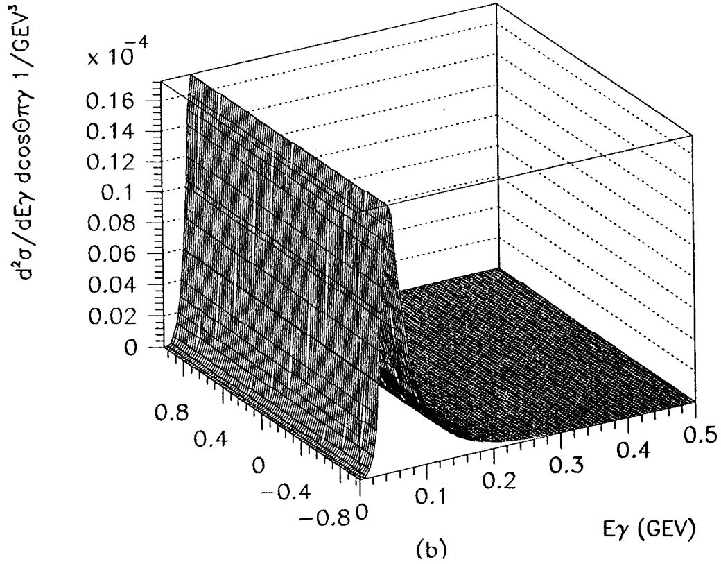
Figure 15. a. d^2\sigma/dE_\gamma d\cos\theta_{\gamma,\text{beam}} vs E_\gamma , \cos\theta_{\gamma,\text{beam}} ; b. d^2\sigma/dE_\gamma d\cos\theta_{\pi\gamma} vs E_\gamma , \cos\theta_{\pi\gamma} for the signal process, \phi \rightarrow f_0\gamma \rightarrow \pi^+\pi^-\gamma .
