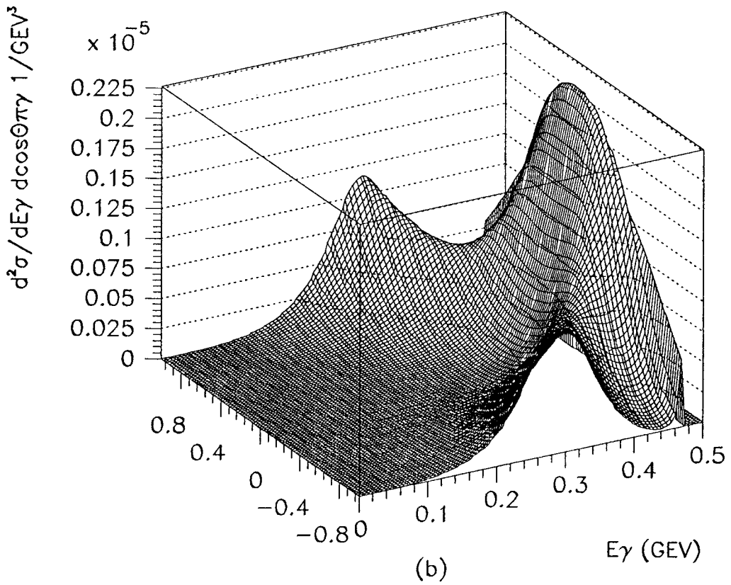
Figure 12. a. d^2\sigma/dE_\gamma d\cos\theta_{\gamma,\text{beam}} vs E_\gamma , \cos\theta_{\gamma,\text{beam}} ; b. d^2\sigma/dE_\gamma d\cos\theta_{\pi\gamma} vs E_\gamma , \cos\theta_{\pi\gamma} for \phi_{e^+e^-} \rightarrow \rho\pi \rightarrow \pi^0\pi^0\gamma .
