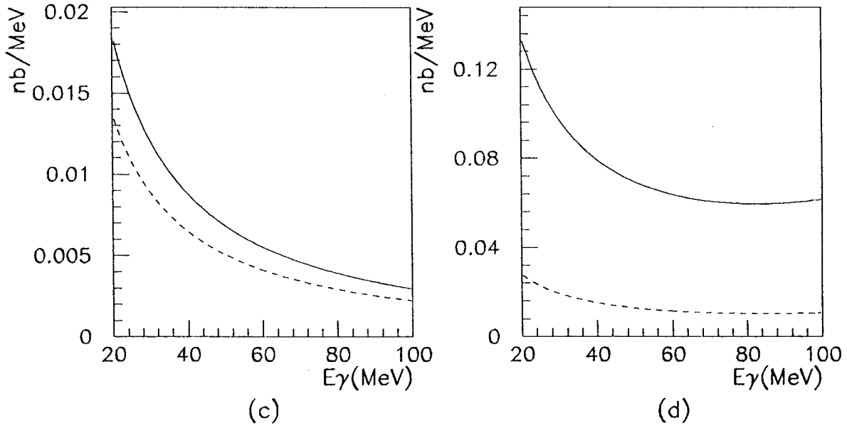
Figure 3. a. |A_1|^2 contribution; |A_2|^2 contribution; c. |A_\rho|^2 contribution; d. Total incoherent background. Solid lines are without angular cuts, dotted lines are for |\cos\theta_{\gamma, \text{beam}}| < 0.9 and |\cos\theta_{\pi\gamma}| < 0.9 .
