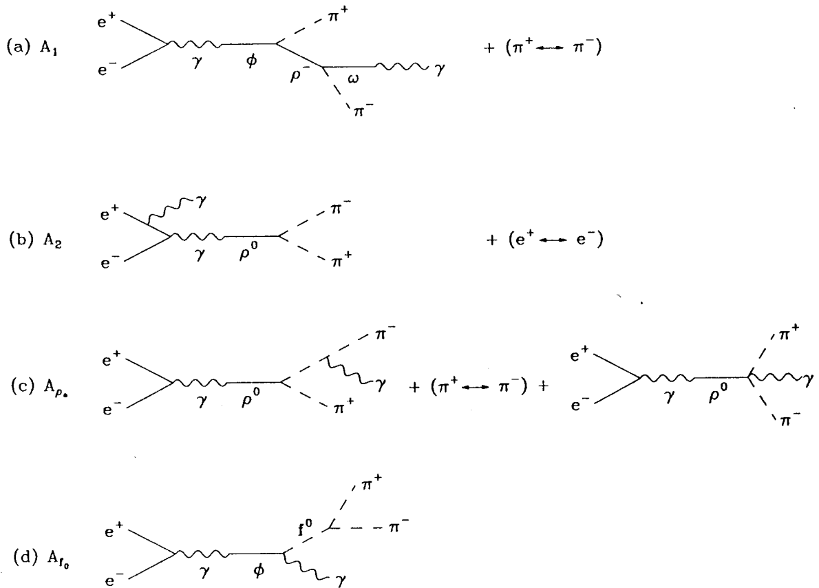
Figure 2. The Feynman diagrams of the processes discussed in the text.
