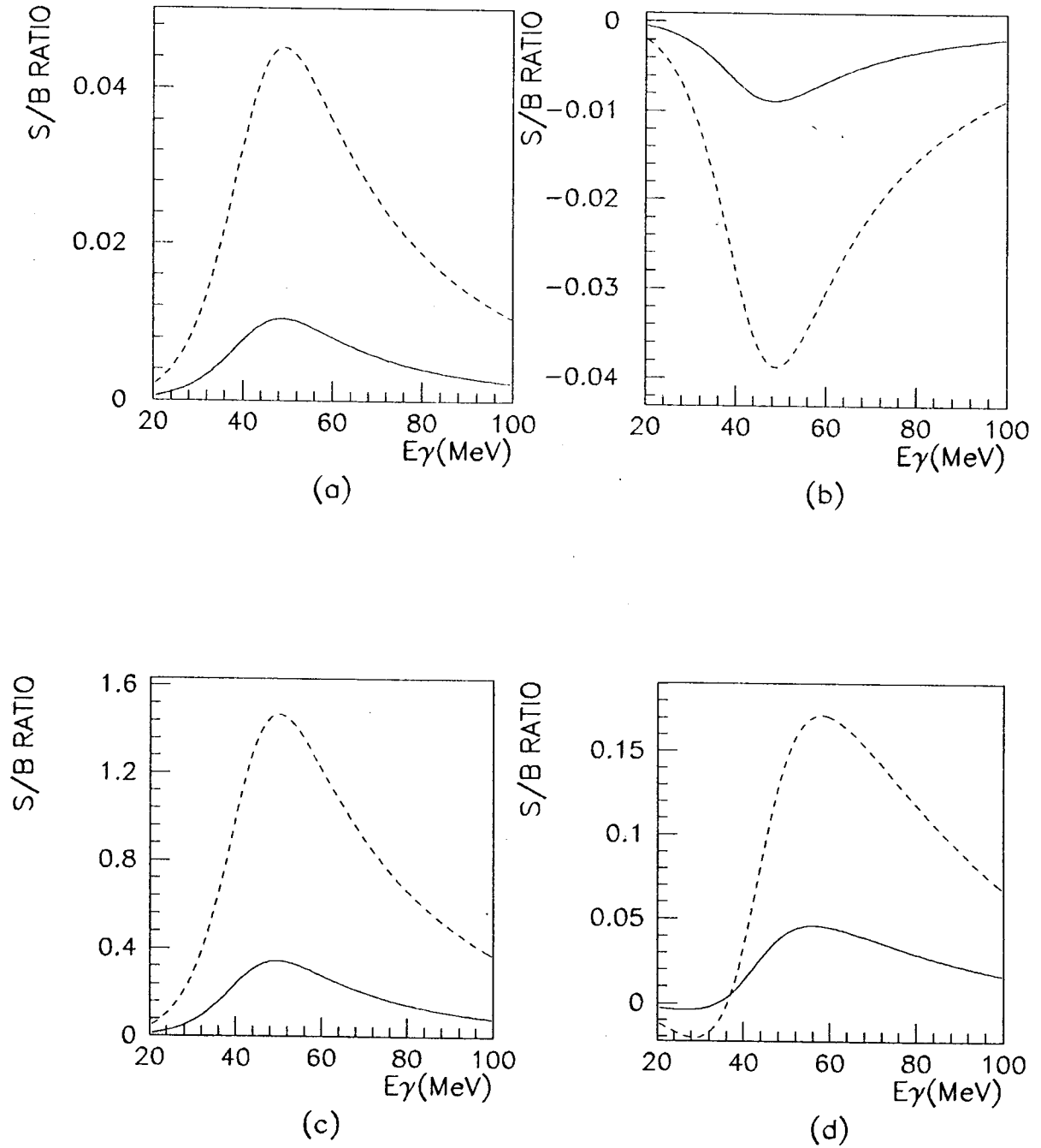
Figure 8. S/B ratio for a. constructive b. destructive interference, BR=1 \times 10^{-6} ; c. constructive d. destructive interference, BR=2.5 \times 10^{-4} . Solid lines are without angular cuts, dotted lines are for |\cos \theta_{\gamma, \text{beam}}| < 0.9 and |\cos \theta_{\pi\gamma}| < 0.9 .
