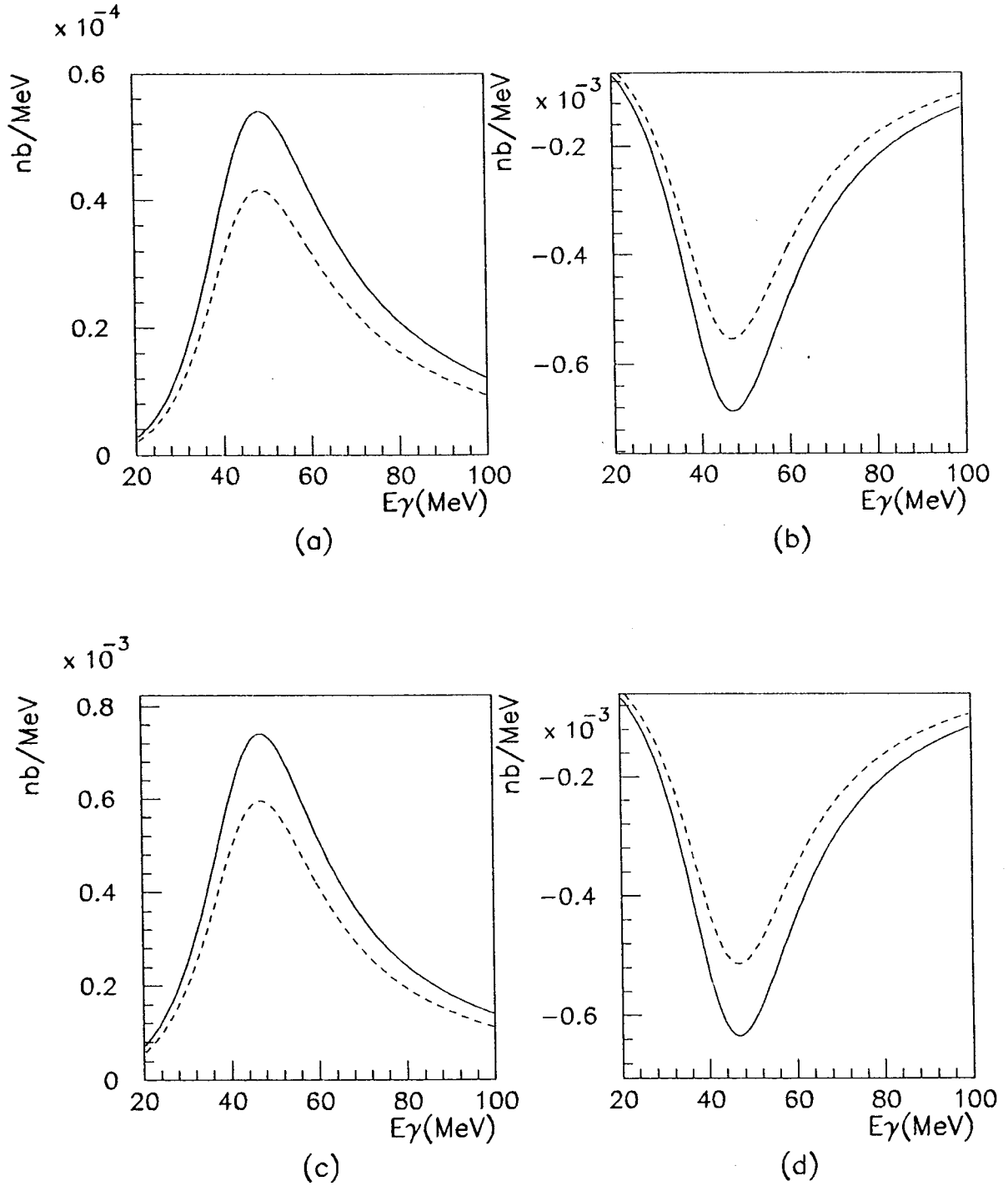
Figure 4. a. \gamma spectrum: f_0 \rightarrow \pi^+ \pi^- \gamma ; b. 2\Re(A_\rho \cdot A_{f_0}^*) ; c. |A_\rho|^2 - 2\Re(A_\rho \cdot A_{f_0}^*) ; d. |A_\rho|^2 + 2\Re(A_\rho \cdot A_{f_0}^*) . \text{BR}_{\phi f_0 \gamma} = 1 \times 10^{-6} . Solid lines are without angular cuts, dotted lines are for |\cos \theta_{\gamma, \text{beam}}| < 0.9 and |\cos \theta_{\pi \gamma}| < 0.9 .
