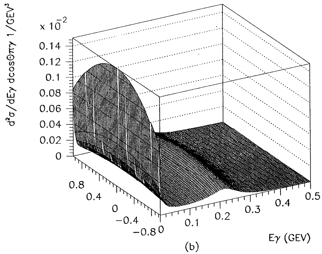
Figure 13. a. d^2\sigma/dE_\gamma d\cos\theta_{\gamma,\text{beam}} vs E_\gamma , \cos\theta_{\gamma,\text{beam}} ; b. d^2\sigma/dE_\gamma d\cos\theta_{\pi\gamma} vs E_\gamma , \cos\theta_{\pi\gamma} for initial state radiation.
