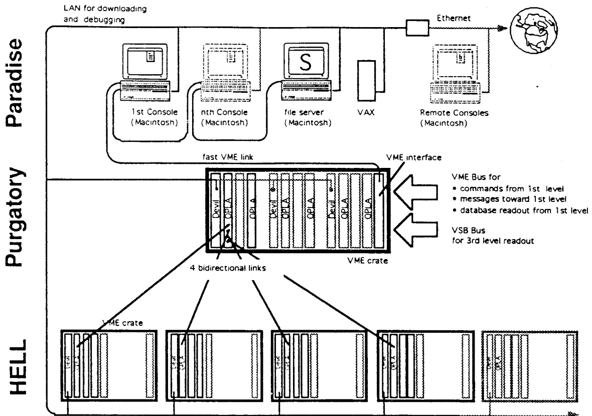
Fig. 2: DANTE schematic diagram
