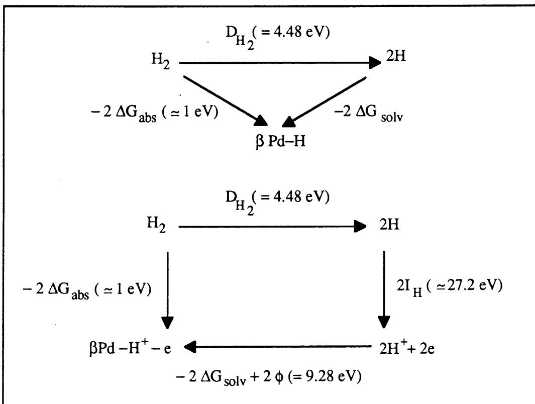
FIG. 1 - Two possible Born-Haber cycles for \beta Pd-H.
