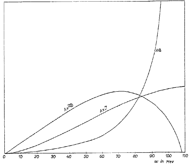
FIG. 1. The different contributions to the \pi^+ spectrum in K \rightarrow \pi + \pi^0 + \gamma . A\mathcal{B} is the bremsstrahlung term, A\alpha^2\mathcal{D} is the direct term, and A\alpha g is the interference between the two. The value of the parameter \alpha is here chosen to be 15.
