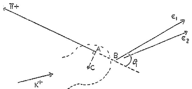
FIG. 1. Diagram showing the procedure for estimating the projected flight path of the \pi^0 meson. C is the center of the last grain in the K -meson track which is indicated by an irregular broken line.
