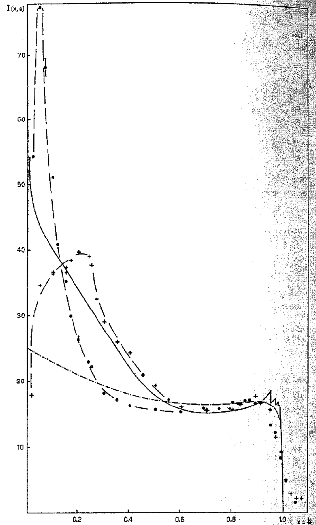
FIG. 2. Intensity of the bremsstrahlung produced in a Si single crystal ( T = 293^\circ\text{K} ) versus x = k/E (the fractional energy of the photon with respect to the electron energy E = 1 Gev). The solid curve represents I(x, \theta) given by formula (3) for \theta = 6 mrad. The dash-dot line represents the same quantity for a noncrystalline target [H. Bethe and W. Heitler, Proc. Roy. Soc. (London) A146 , 83 (1934); Wheeler and Lamb, reference 4]. The experimental points represent the quantity (5). The circles are relative to \theta = 6 \pm 0.5 mrad, while the crosses are relative to \theta = 1 \pm 0.5 mrad.
