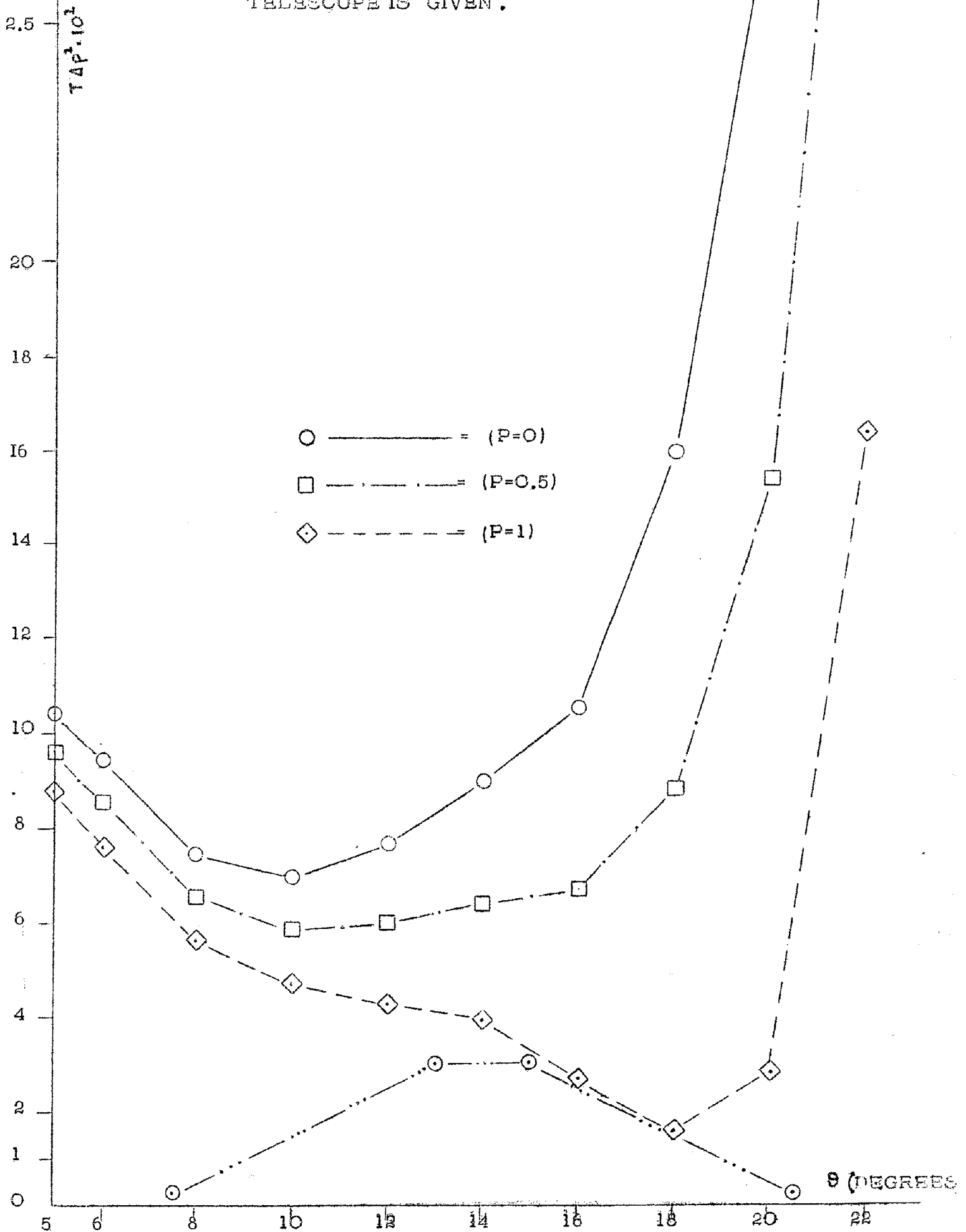
FIG.5 THE PRODUCT T\Delta p^2 VERSUS THE ELASTIC SCATTERING ANGLE IN CARBON OF 180 MEV PROTONS . BELOW THE CURVES THE ANGULAR RESOLUTION OF OUR TELESCOPE IS GIVEN .
